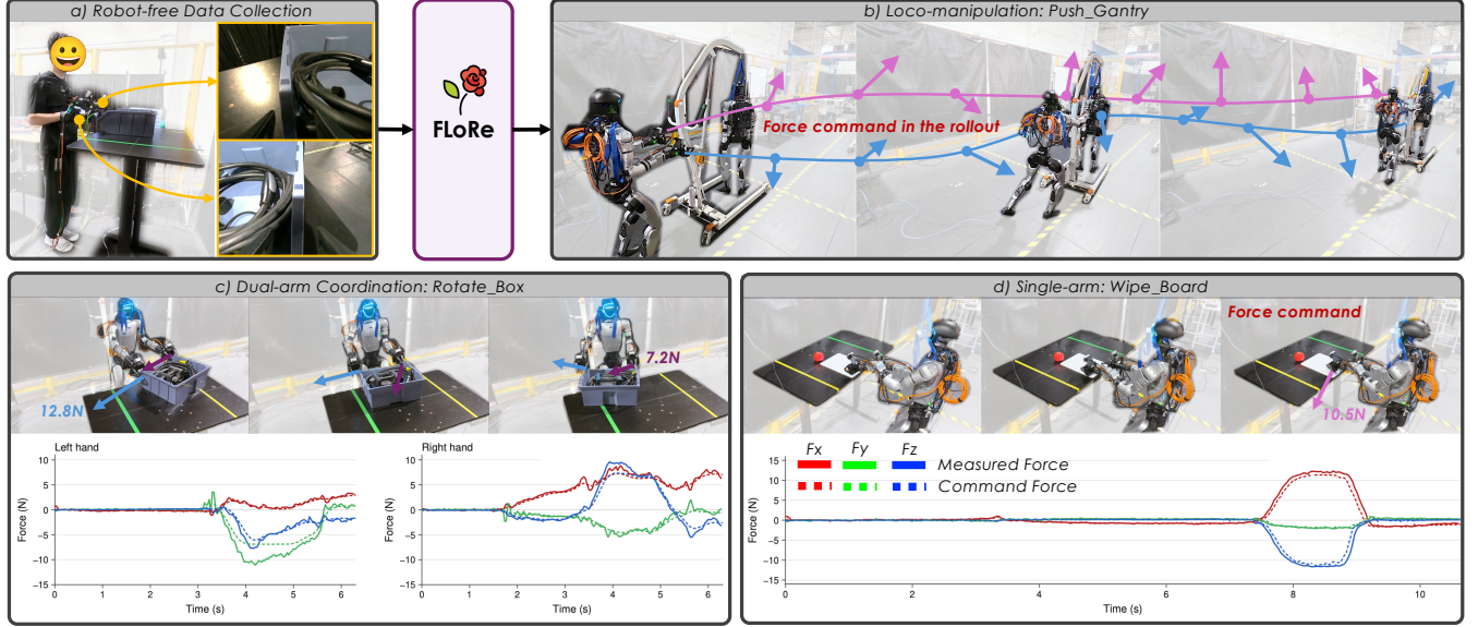
Fig. 1. FLORE is a framework that learns force-reactive loco-manipulation from robot-free demonstrations. (a) Two handheld UMI-style grippers carrying 6-axis F/T sensors and three trackers record hand/torso motion, gripper width and contact forces. From these demonstrations, we train a force-reactive diffusion policy that predicts per-hand force commands. A unified force-position whole-body controller then executes the motion and force together, enabling the following capabilities: (b) robustness to force variation : the robot walks a heavy wheeled gantry forward with both hands; (c) bimanual coordination : the robot rotates a heavy box (12 kg) while dragging it across the table without tipping or lifting it; (d) sustained contact : one hand presses an eraser against a whiteboard and holds a steady normal force through the stroke. The overlaid curves trace the hand keypoints and the arrows mark the commanded force at its peak; the traces below show the commanded (dashed) and measured (solid) force per hand and axis.
