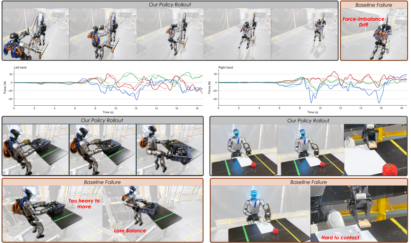
Fig. 6. Rollouts on the robot and failure modes of the position-only baseline. Top: Ours walks the gantry forward from left to right. The baseline either fails to move the gantry or pushes unequally, causing it to drift from its heading. The traces show commanded (dashed) and measured (solid) force for each hand and axis. Bottom left: Ours drags and rotates the box. The baseline either cannot move it or leans into it and loses balance. Bottom right: Ours erases the strip under steady pressure. The baseline hovers above the board and never makes contact.
