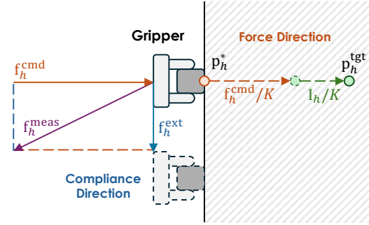
Fig. 3. Control law of the hybrid compliance controller. Along the force direction, the target \mathbf{p}_h^{\text{tgt}} is shifted from the motion reference \mathbf{p}_h^* into the surface by the force command and the force feedback, until the measured force \mathbf{f}_h^{\text{meas}} balances the command. Along the compliance direction, the gripper yields to \mathbf{f}_h^{\text{ext}} (dashed gripper).
