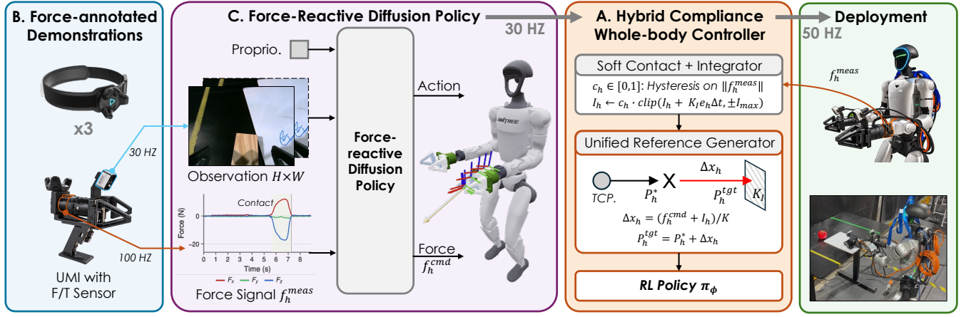
Fig. 2. Overview of our FLORE framework. (B) Two handheld UMI-style grippers with F/T sensors and three additional trackers record images, motion, and contact force without a robot. (C) A force-reactive diffusion policy takes images, state and measured force as input and outputs keypoint motion and desired force commands at 30 Hz. (A) The hybrid compliance whole-body controller with force tracking converts the force command into a shift of the target along the force direction, so that one RL policy tracks motion and force simultaneously while remaining compliant along other directions.
