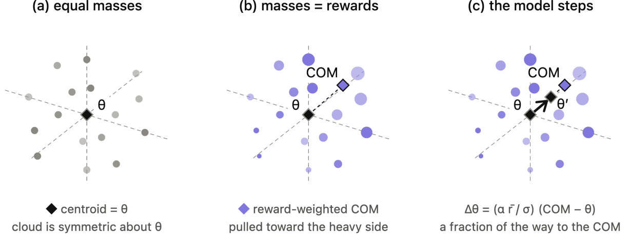
Figure 1: One ES update as a change of center of mass. (a) Candidates are sampled around the model \theta in antithetic pairs, so with equal masses the population’s centroid coincides with \theta . (b) Giving each candidate a mass equal to its reward moves the center of mass (COM) towards the high-reward side. (c) The update is proportional to the displacement from the centroid to the COM, \Delta\theta = (\alpha \bar{r} / \sigma) (\mathbf{p}_{\text{COM}} - \bar{\mathbf{p}}) , which here starts at \theta . The same sixteen candidates are shown in every panel; displacements are exaggerated for visibility.
