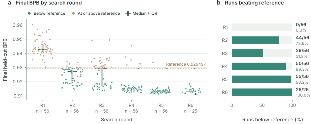
Figure 6: The quality-driven search progressively moves into a stronger region. Each point shows the final held-out BPB of one valid candidate, grouped by search round; horizontal jitter is used only to avoid overlap. Green points outperform the fixed reference (dashed line), while gray bars show the median and interquartile range within each round. The distribution shifts substantially below the reference after the first round and becomes increasingly concentrated at lower BPB in later rounds. Overall, 203 of 305 valid candidates outperform the reference.
