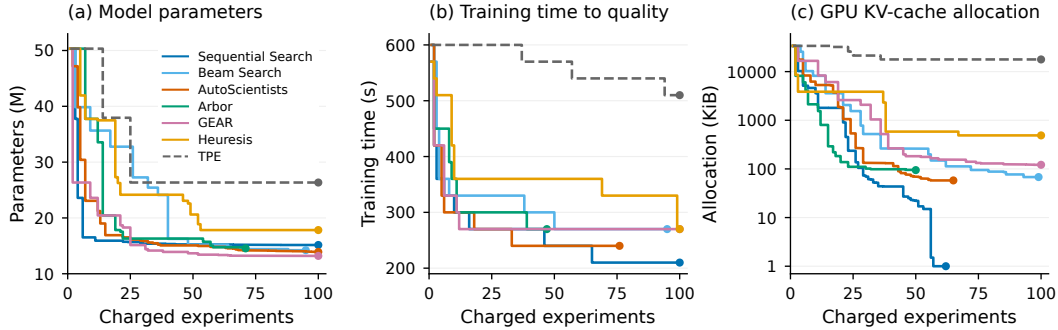
Figure 3: Research trajectories behind the Opus 5 benchmark results. Curves track the best admissible result found as each search proceeds, ordered by charged experiments; lower is better. Counts include the reference evaluation and charged failures, and dots mark the end of each recorded search. Training time is measured at 30-second validation checkpoints, and KV-cache allocation is shown on a logarithmic scale.
