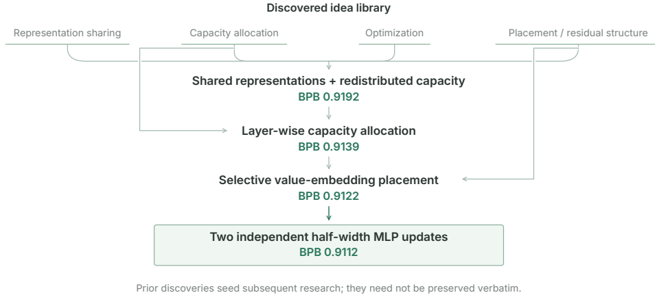
Figure 5: The selected design emerges through reuse and reinterpretation of prior discoveries. The quality-driven search builds on mechanisms for representation sharing and capacity allocation, subsequently changing where these mechanisms act and ultimately reinterpreting the MLP update as two independent half-width sublayers. Rather than simply accumulating prior discoveries, the search selects, recombines, and modifies them into new designs.
