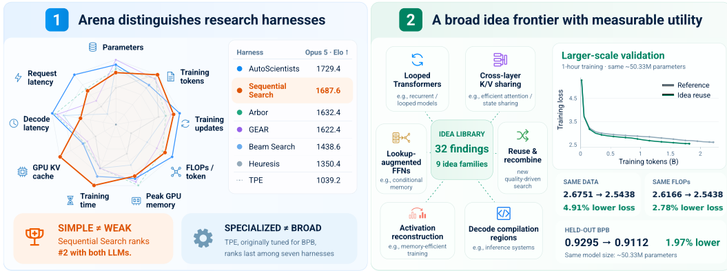
Figure 1: Auto-Research Arena evaluates research systems and expands the idea frontier. Left: Arena differentiates research harnesses across nine complementary objectives. Our simple Sequential Search baseline remains competitive, whereas the TPE method tailored to validation-loss minimization underperforms in this broader evaluation. Right: Multi-target research reveals a broad frontier of ideas. A program combining these discoveries achieves lower training loss than the reference program under matched data and FLOP budgets, as well as lower final held-out BPB at the same model size.
