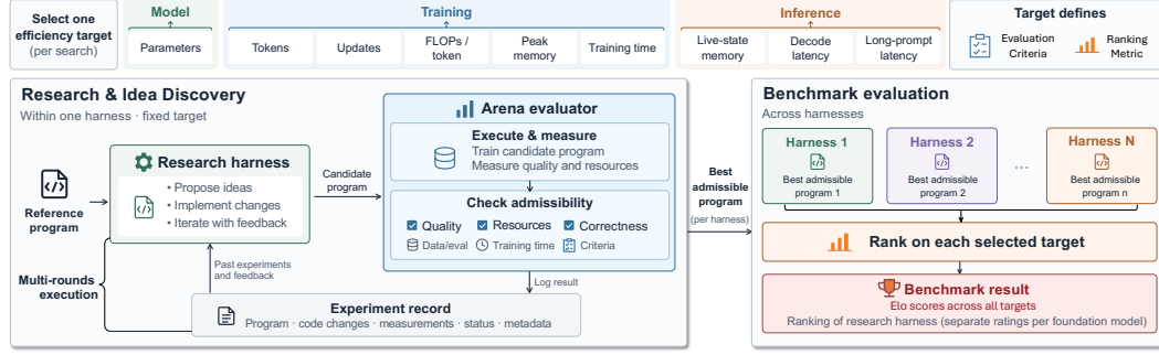
Figure 2: Overview of Auto-Research Arena Pipeline. Each search run optimizes one of nine efficiency targets. A research harness proposes and implements changes to a reference program. Arena evaluates the resulting candidates, records outcomes, and provides feedback. The best admissible candidate determines the benchmark result.
