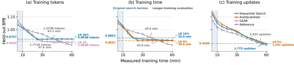
Figure 4: Discovered programs can transfer beyond the search horizon. Programs discovered with 10-minute candidate training are retrained from random initialization for 60 minutes alongside the reference. Several retain their advantages for substantially longer than the original search horizon, although these gains can diminish later as horizon-specific training policies take effect. Curves show held-out BPB against training time. Annotated comparisons use checkpoints after the learning-rate schedule reaches its floor, except in figure (c), where AutoScientists’ final BPB defines the shared target.
