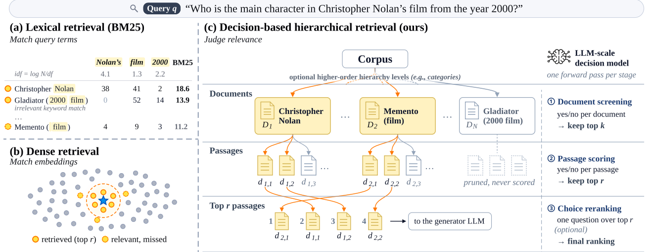
Figure 2. Retrieval by matching versus retrieval by decisions. (a) BM25 and (b) dense retrieval match query terms or embeddings and can miss the relevant page. (c) DecisionRAG walks the corpus hierarchy: a decision model judges all candidates of a level in one forward pass, keeping the top k documents and then the top r passages; pruned documents are never expanded. Term frequencies, IDF values, BM25 scores, and rankings in panel (a) are illustrative.
