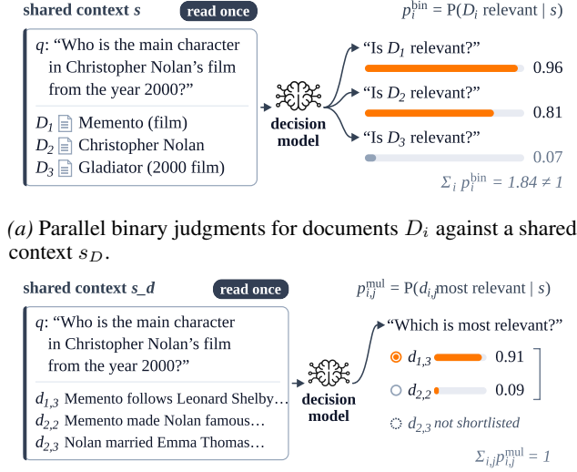
(a) Parallel binary judgments for documents D_i against a shared context s_D . (b) Multiple-choice reranking of the top passages from the binary judgments against the same shared context s ; the probabilities sum to one.
