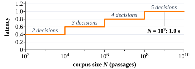
Figure 4. Analytical model: sequential stages grow with the depth of the hierarchy, not the size of the corpus. Theoretic latency per query (Equation (4), b = 100 ), assuming a balanced hierarchy and enough serving capacity to judge every level in parallel: each 100\times more passages adds one level, i.e., one more sequential decision ( \approx 0.2 s).
