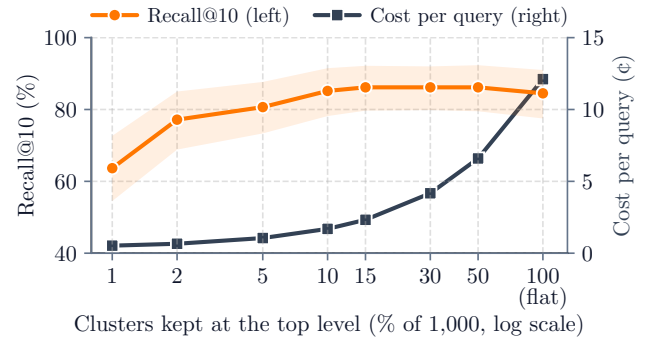
Figure 7. Recall@10 (left axis) and Jev cost per query (right axis) on Natural Questions as the top level keeps more and more clusters. First 100 test questions of Table 2; band: 95% interval.
