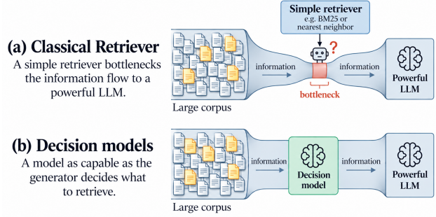
Figure 1. Capability asymmetry: a simple retriever bottlenecks a powerful LLM (a); decision models level the playing field (b).
