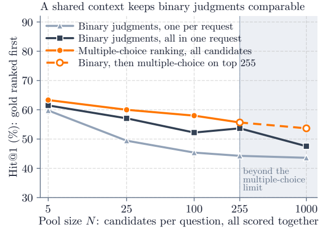
Figure 5. Hit@1 on Natural Questions as the candidate pool grows, with all N candidates scored in one request (150 questions).
