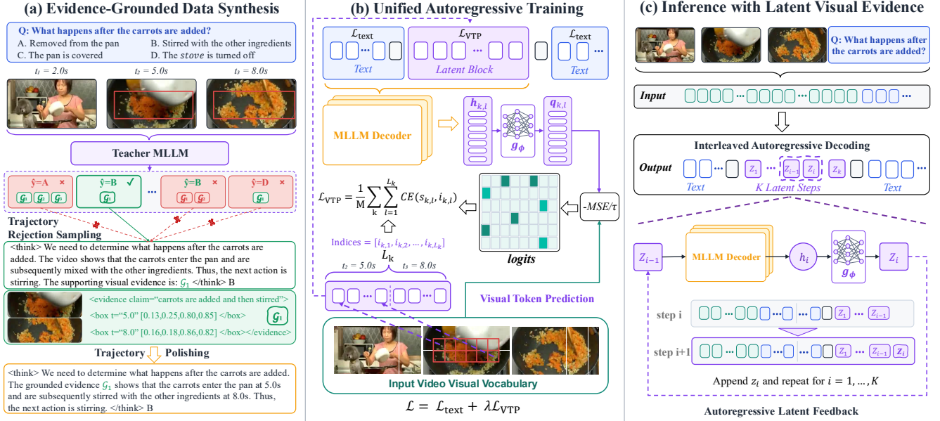
Figure 1: Overview of VideoLVR. (a) A teacher MLLM synthesizes evidence-grounded reasoning trajectories through rejection sampling and trajectory polishing. (b) Visual tokens from regions supporting the same reasoning step are grouped and ordered by timestamp to form latent targets. VideoLVR jointly trains text generation with next-token prediction and latent visual evidence generation with visual token prediction over the input-video visual vocabulary. (c) At inference with the supervised model, each decoder hidden state is projected into a latent visual state and fed back as the input for the next decoding step, enabling autoregressive reasoning over latent visual evidence without additional visual observations.
