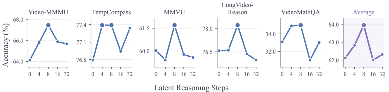
Figure 2: Effect of the inference-time latent-step budget on five video benchmarks. Enlarged markers denote the best results.
