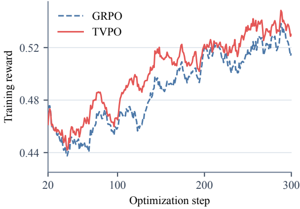
Figure 3: Comparison of training reward curves for GRPO and TVPO, shown as trailing 20-step moving averages.
