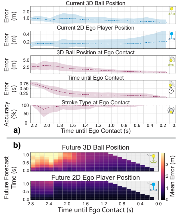
Fig. 4: LFM2.5-VL 450M results on approaching test-split shots until contact. (a) Predictions for a single frame horizon tend to improve as the ball nears the ego player. (b) Forecasted predictions tend to improve as the ball nears the ego player and degrade as the future horizon increases.
