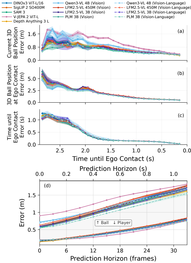
Fig. 3: Prediction errors on approaching test-split shots versus time to contact: (a) current 3D ball position, (b) ball position at contact, and (c) time to contact. Lines show means over 0.1 s intervals; shading shows \pm 1 SD over three seeds. (d) Ball 3D and player 2D future predictions over a time horizon of \sim 1.10 s, across all models, averaged over three seeds.
