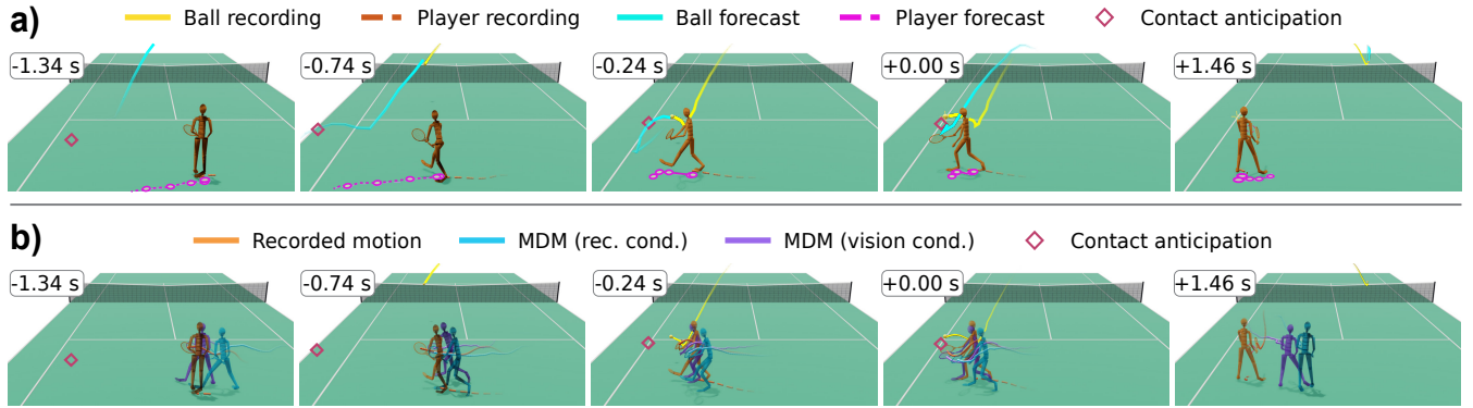
Fig. 5: (a) LFM2.5-VL-450M forecasts ball and player positions and anticipates contact; crosshairs locate the recorded contact. (b) Recorded ego motion versus MDM rollouts conditioned on annotations (“rec. cond.”) or vision predictions (“vision cond.”). Trails fade toward the past; ball forecasts fade toward the future. t = 0 denotes the recorded racket-ball contact.
