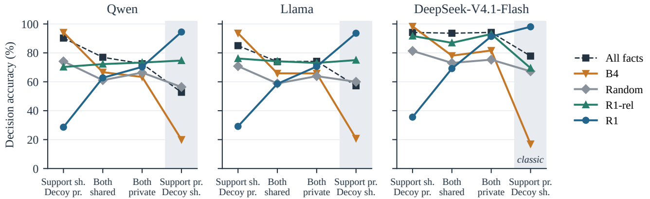
Figure 3: Who wins depends on who holds what. CrossProfile accuracy at r = .6 by support and decoy ownership (each point averages the two irrelevant-fact assignments, 60 templates, three seeds). R1 and B4 are mirror images; R1-rel varies little across cells but falls well below R1 in the classic hidden-profile column (shaded: private support, shared decoys), where even the all-facts memory (dashed) drops. Per-cell intervals for Qwen and Llama are in Appendix A.2.
