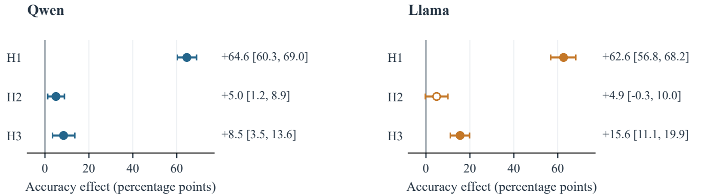
Figure 6: Primary contrasts at r = .6 . H1: dependence of the R1 advantage over B4 on decoy ownership. H2: R1 accuracy with shared minus private irrelevant facts. H3: R1-rel minus R1 with private irrelevant facts. Points and whiskers show estimates and 95% template-bootstrap intervals. Filled markers are significant after Holm correction over H1–H3 within each model; Llama H2 is not.
