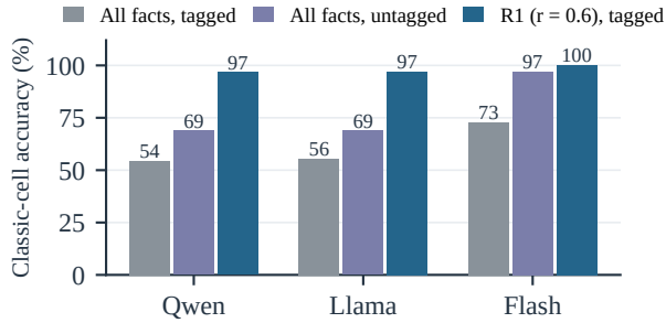
Figure 5: Holder tags mislead the decision model. Accuracy in the classic cell (private support, shared decoys, private irrelevant facts) for the all-facts memory with and without holder tags, and for R1 at r = .6 (60 templates, three seeds; Flash: DeepSeek-V4.1-Flash).
