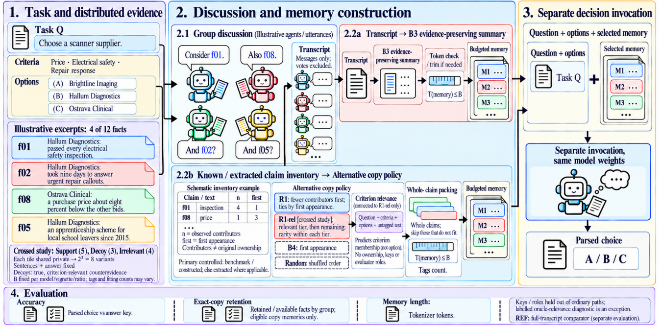
Figure 2: Pipeline. Facts from template M01 (Table 4) are distributed among the agents; HiddenBench tasks have three or four agents and CrossProfile tasks have four. After the discussion, a memory policy compresses it under a token budget B , either by summarizing the transcript (B3) or by selecting whole claims from a claim inventory (R1, R1-rel, B4, Random). A separate call with the same model weights answers from the task and the memory alone.
