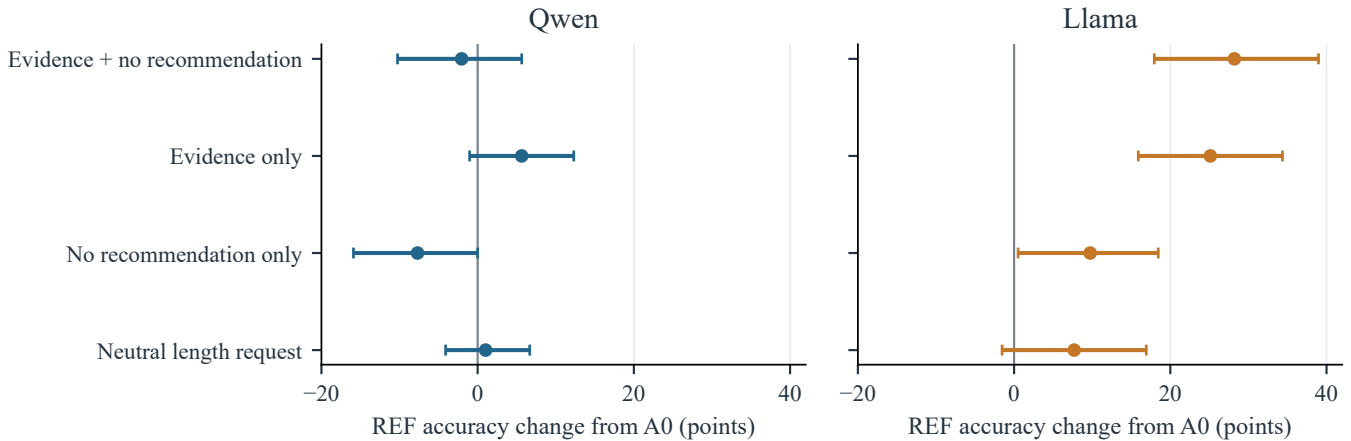
Figure 9: Discussion-prompt ablation: change in REF accuracy relative to A0, with 95% task-bootstrap intervals. Qwen does not reproduce Llama’s large gain from evidence-first wording.
