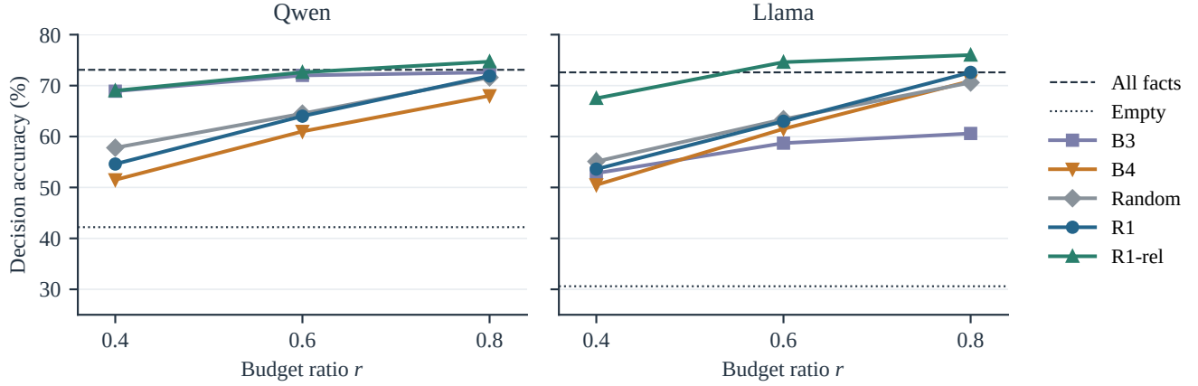
Figure 7: CrossProfile accuracy across budget ratios (Table 6). Points are means over templates, variants, and seeds; horizontal lines mark the unbudgeted all-facts and empty controls.
