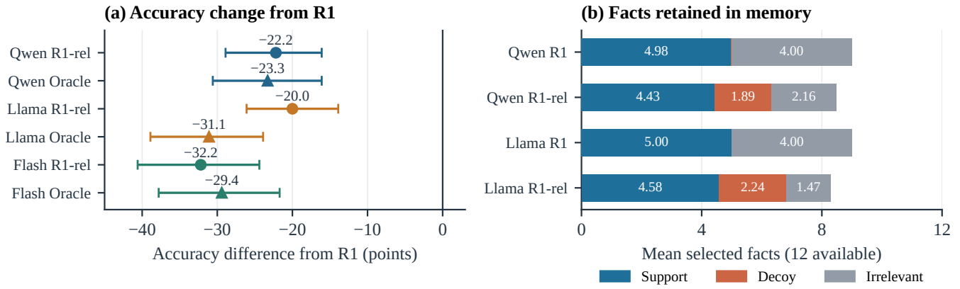
Figure 4: Criterion relevance is insufficient in the classic hidden-profile cell (private support, shared decoys, private irrelevant facts, r = .6 ). (a) Accuracy differences from R1 for R1-rel and for oracle relevance on Qwen, Llama, and DeepSeek-V4.1-Flash (Flash), with 95% template-bootstrap intervals. (b) Mean number of selected facts by role on Qwen and Llama: relevance-first priority admits shared decoys.
