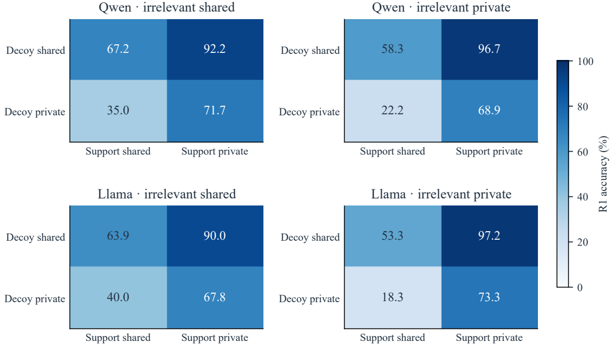
Figure 8: R1 accuracy at r = .6 by support and decoy ownership, separately for each model and irrelevant-fact assignment. Every cell averages the same 60 templates and three seeds; intervals are in Tables 7 and 9.
