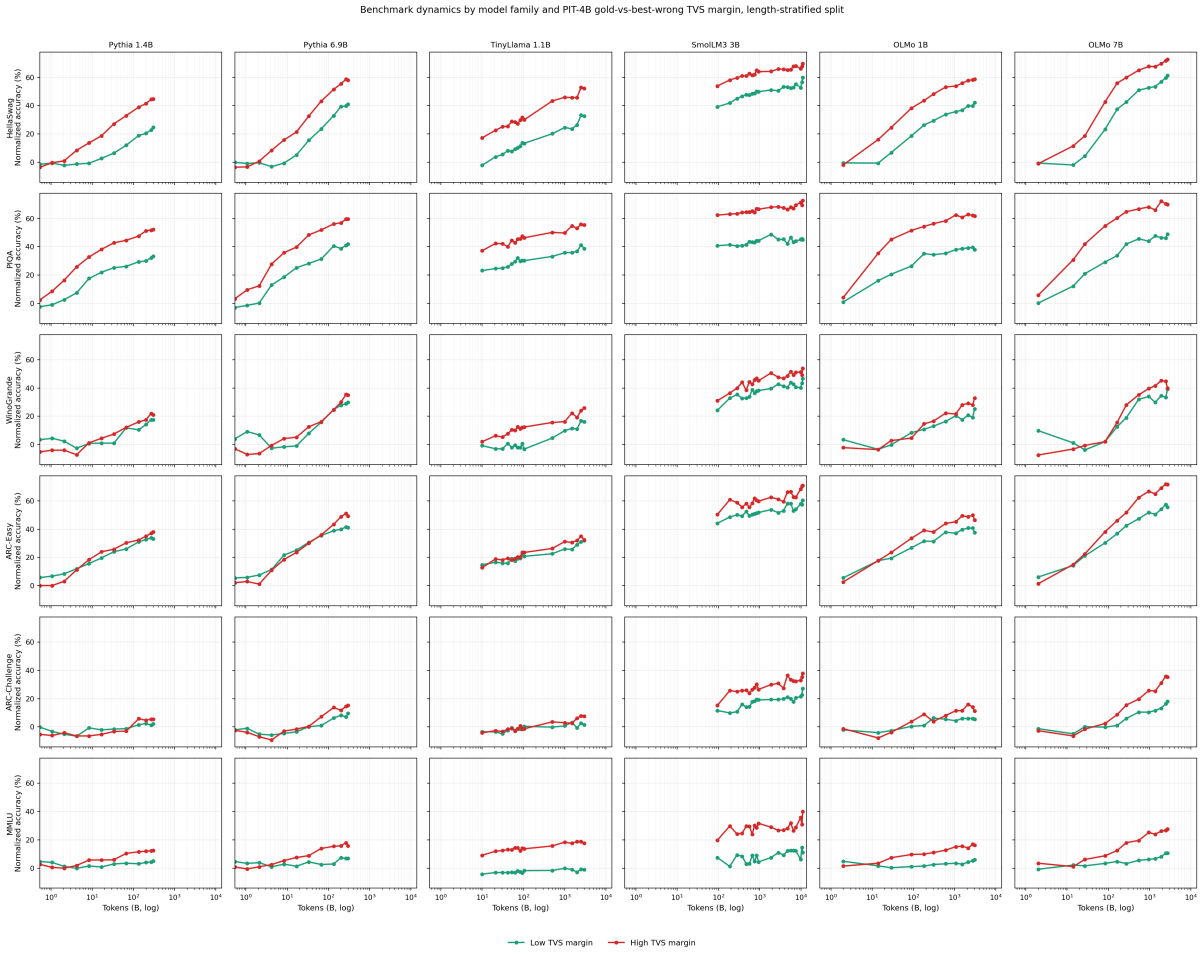
Figure 5: Split by the gold-versus-wrong TVS margin. Items whose gold answer is more temporally variable than the best wrong answer show the largest final-checkpoint advantage.
