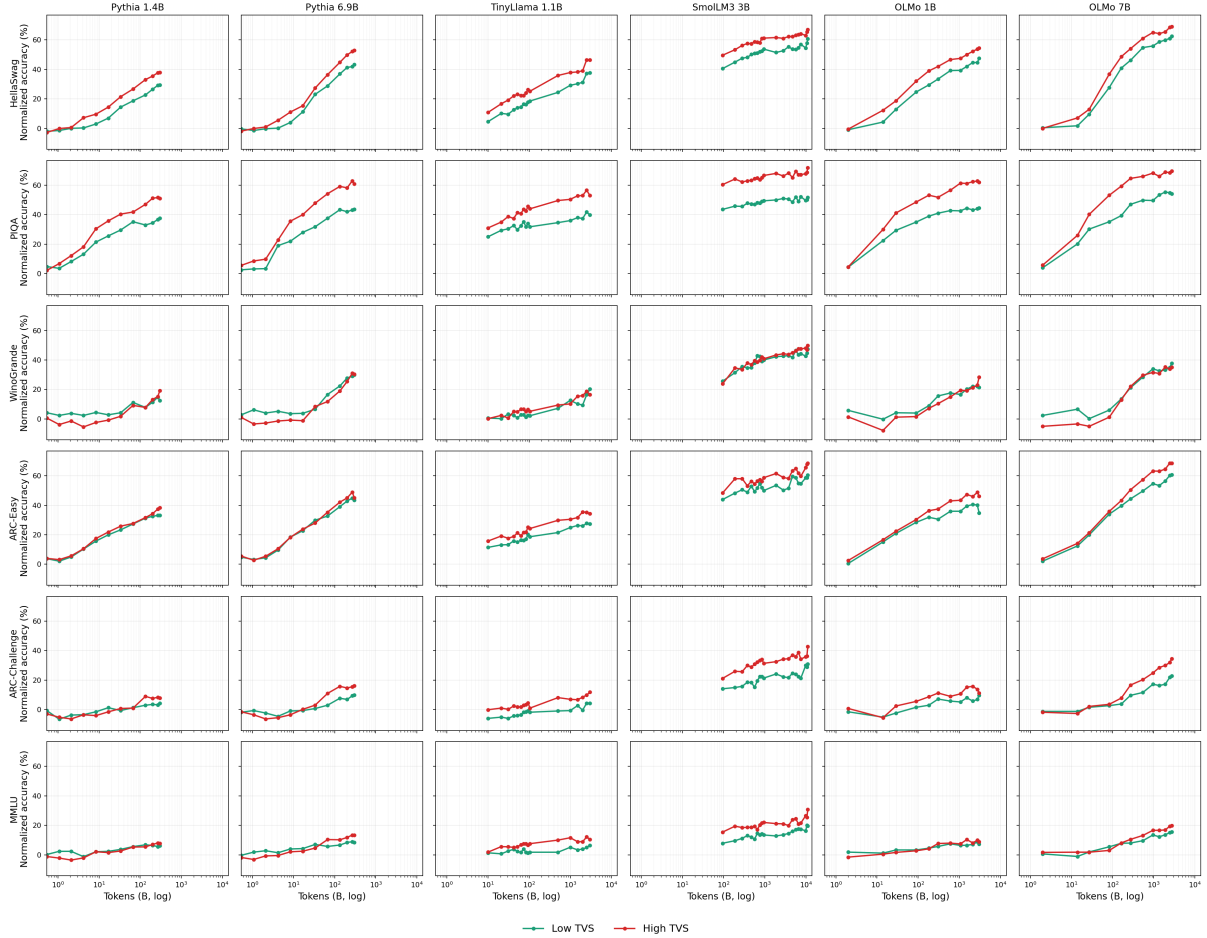
Figure 1: Chance-normalized accuracy over pretraining for temporally variable (high TVS, red) and temporally stable (low TVS, green) items, by model (columns) and benchmark (rows). Groups are length-matched; training tokens are on a log scale. Pythia and OLMo show little early separation; high-TVS items generally pull ahead later.
