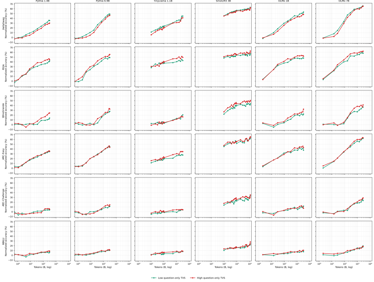
Figure 4: Split by question-only TVS. The effect is much weaker than for the question and gold answer together, so the signal is not reducible to the question stem.
