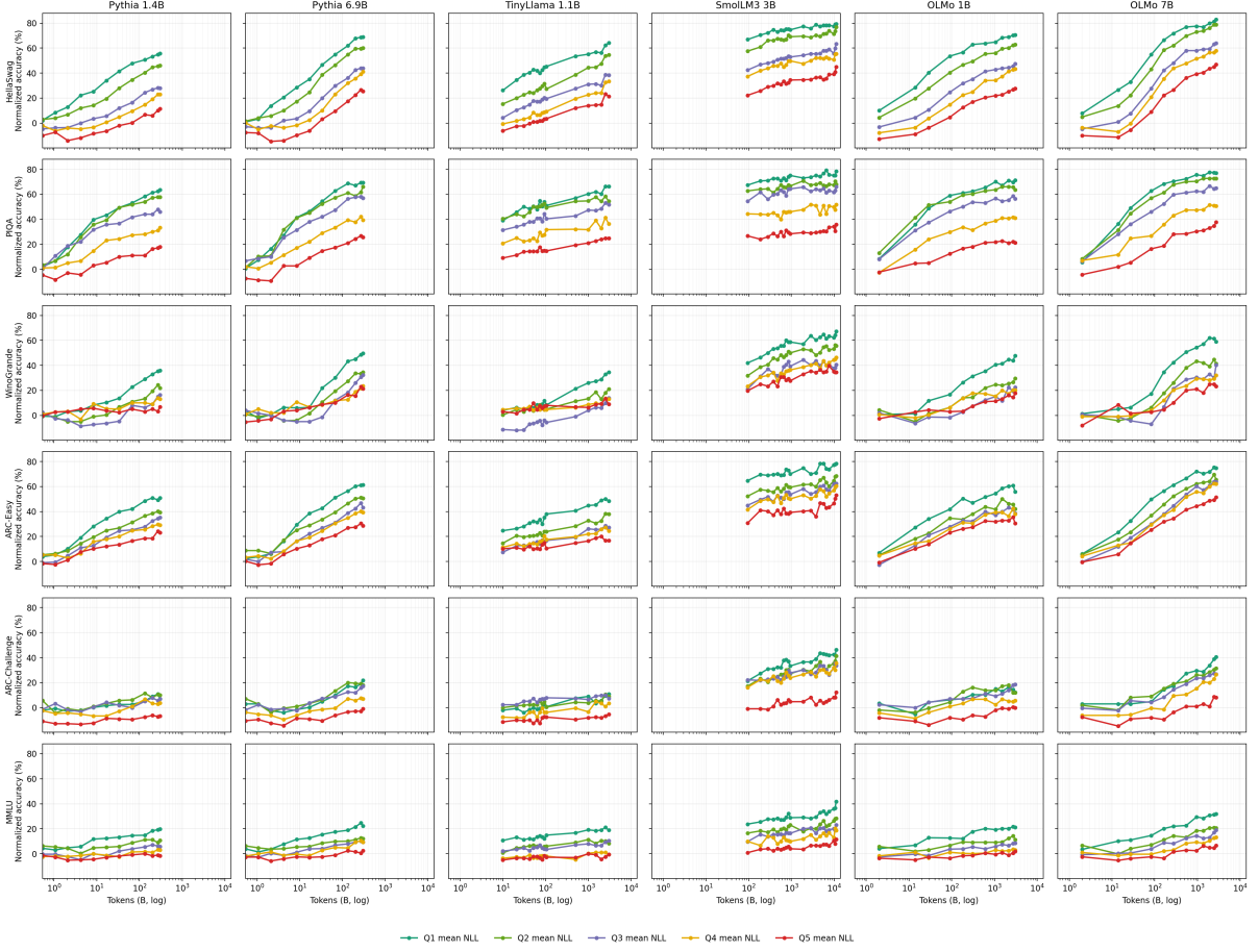
Figure 3: Split by mean gold NLL. Higher mean NLL is associated with lower accuracy at all checkpoints. Difficulty-conditioned TVS results are reported separately in Appendix B.1.
