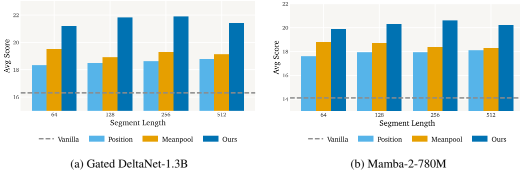
Figure 4: MERLIN Outperforms Baselines Across Segment Length. Average score as the segment size that defines each state varies over {64, 128, 256, 512}. MERLIN leads at every segment length, and its margin over mean-based aggregation persists as segments grow. Vanilla (dashed) is segment-independent.
