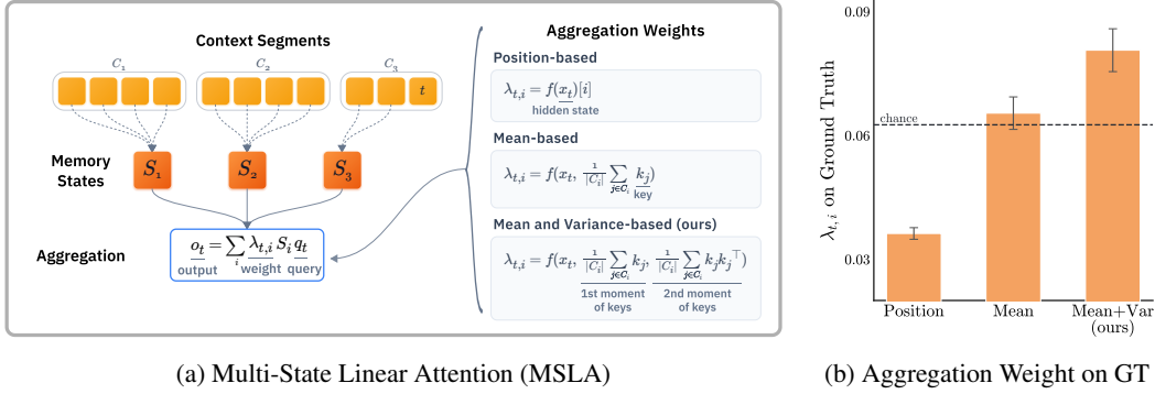
Figure 1: (a) A multi-state linear attention (MSLA) model aggregates segment-level outputs via a weighted sum. Prior methods compute the weights \lambda_{t,i} from position or from the mean of each segment’s keys. MERLIN instead reads both the first and second moments of the keys. (b) On retrieval-augmented generation samples in HELMET (Yen et al., 2025), we measure the aggregation weight each method places on the ground truth (GT) segment at the query token. Position-based aggregation largely misses the GT and mean-based aggregation recovers more, while MERLIN places the most weight on it.
