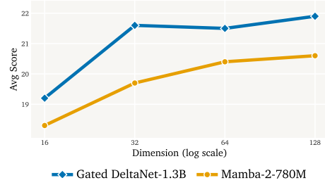
Figure 5: Dimension of Moments. Average LongBench scores as d_r varies over \{16, 32, 64, 128\} (log axis). Performance saturates around d_r = 32 for GDN and d_r = 64 for Mamba-2.
