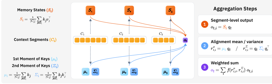
Figure 2: MERLIN Overview. The context is split into segments C_i (middle row). Each segment stores a memory state (top row) and the first and second moments of its keys (bottom row). At position t , the query q_t reads segment-level outputs from memory states (step 1). The query computes the mean and variance of the key-query alignment from the moments (step 2). The final output is a weighted sum of segment-level outputs, where the weights are derived from a gated mix of the alignment mean and variance (step 3).
