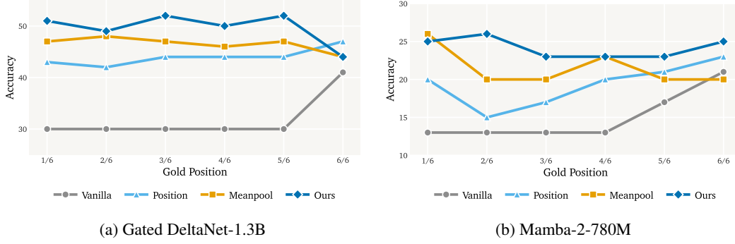
Figure 3: Position-Controlled Retrieval. Retrieval accuracy as the gold passage sweeps from the start (1/6) to the end (6/6) of the context. Vanilla is recency-biased: it recovers the gold only when placed near the end and is otherwise flat, while Position and mean-based aggregation are flatter but weaker. MERLIN stays high and roughly uniform across positions.
