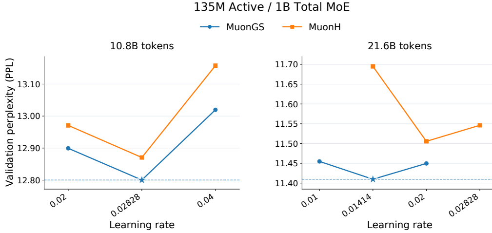
Figure 7: Validation perplexity versus learning rate for MuonGS and MuonH for an 135M active / 1B total MoE model for two different training durations. Stars and dashed horizontal lines indicate the best observed perplexity in each panel.
