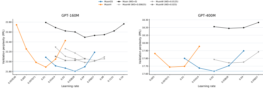
Figure 8: Validation perplexity vs learning rate for MuonGS, MuonH, Muon and MuonW with varying weight decay. Both models are trained for 20k steps (about 10.5B tokens) on FineWeb.
