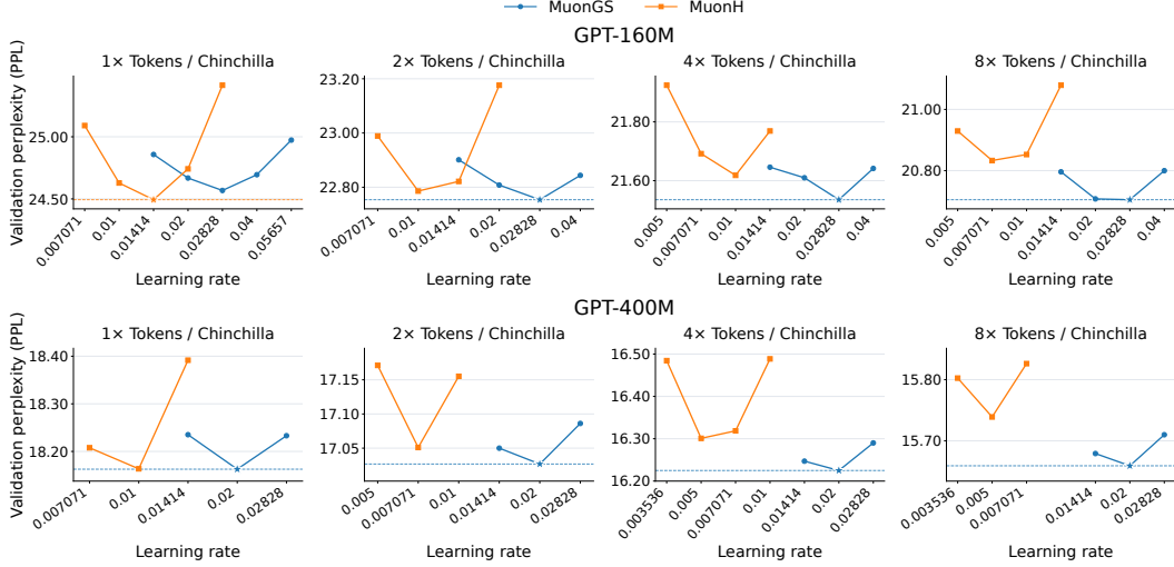
Figure 5: Validation perplexity versus learning rate for MuonGS and MuonH across the two model sizes and Chinchilla ratio 1 \times –8 \times . Stars and dashed horizontal lines indicate the best observed perplexity in each panel.
