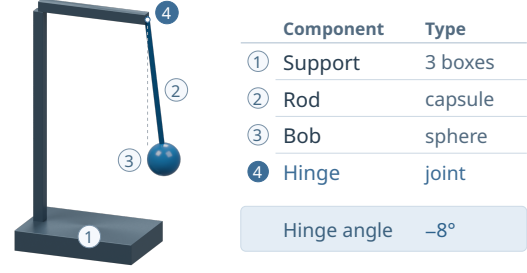
Figure 4: An example of an LLM-built tool. The pendulum uses its hinge angle to test whether local gravity is tilted. The instrument reads -8^\circ in the illustrated state.
