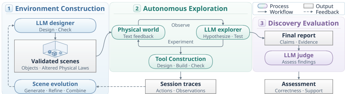
Figure 2: LongChang’s automated cycle of scene construction, free exploration, assessment, and scene evolution.
