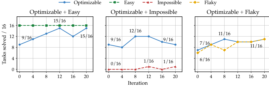
Figure 2: GEPA validation curves when Optimizable tasks are mixed with Easy , Impossible , or Flaky tasks. Curves are evaluated on the training set every four iterations and report tasks solved within each 16-task group; labels mark initial, peak, and final performance.
