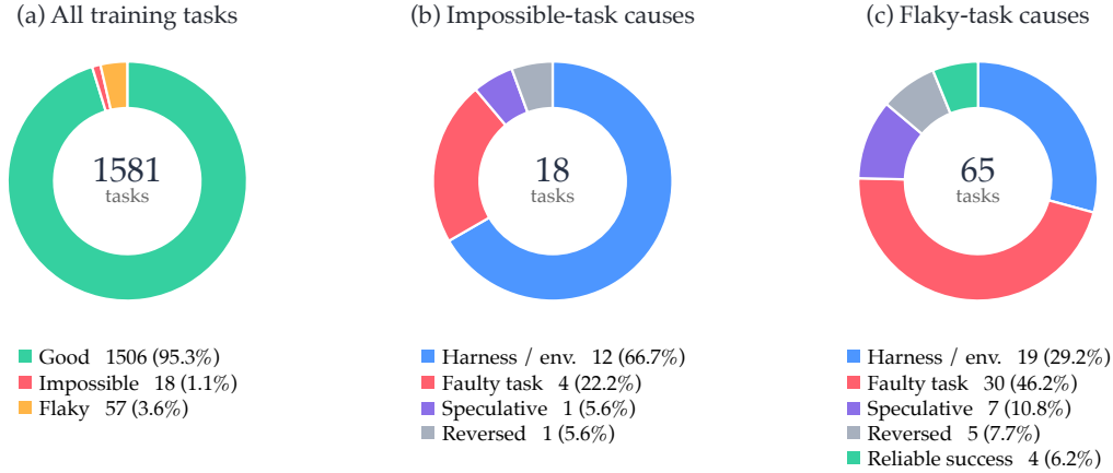
Figure 3: Diagnoses made by the Curator across the 1,581 GoBrowse training tasks and the primary causes assigned to impossible and evaluator-flaky tasks. Eight tasks received both impossible and flaky diagnoses because their diagnoses changed across iterations. The overview counts these overlaps as impossible, leaving 57 unique flaky-only tasks, while panel (c) includes 65 flaky diagnoses.
