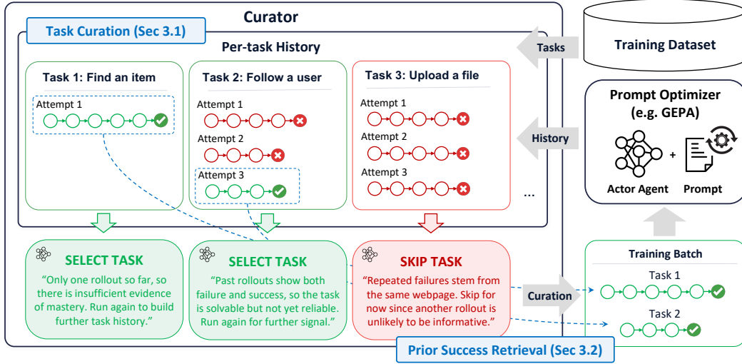
Figure 1: GEPA-Curator system diagram. The prompt optimizer takes in a minibatch of tasks at each iteration and invokes the actor agent to execute them and performs reflective prompt optimization based on the resulting trajectories. The Curator augments the prompt optimizer by acting as an outer-loop process which traverses through the training dataset and constructs each minibatch to pass into the prompt optimizer. The Curator reads past execution trajectories for each task sampled from the training dataset and decides to run the task if doing so is likely to provide useful optimization signal (Section 3.1). The Curator can also pass prior successful trajectories for failed tasks as context to the prompt optimizer as a trusted reference example (Section 3.2). Once the curated training batch of selected tasks and successful context is constructed, it is passed to the prompt optimizer for execution and optimization. The resulting trajectories and evaluation outcomes are then written back to the task history for use in subsequent curation rounds.
