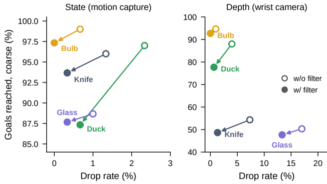
Fig. 24: Goal success versus drop rate on the real robot, per object, from without (open) to with (filled) the safety filter, for the state (left) and depth (right) policies.
