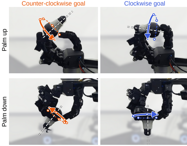
Fig. 9: Spinning the lightbulb about its own axis (depth policy). Palm up (top) and down (bottom), counter-clockwise (left) and clockwise (right) goals.
