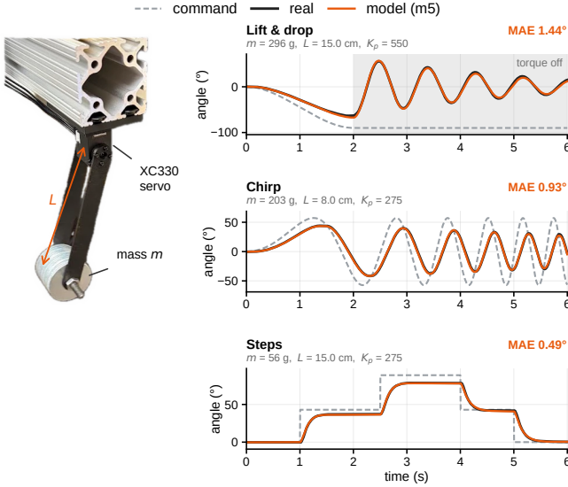
Fig. 15: Actuator identification of the XC330 servo. Left: pendulum test bench (mass m , arm length L ). Right: commanded, real and identified-model angles on three test trajectories.
