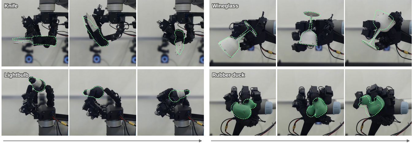
Fig. 1: Our robot hand reaches diverse in-hand object poses at any wrist orientation. For each object (one policy per object), we show three consecutive goals; dashed green outlines indicate target poses, and arrows indicate time.
