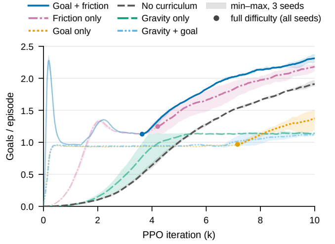
Fig. 6: Knife curriculum ablation over 3 seeds. Goals per episode during A1 for each curriculum variant, including a gravity curriculum ( 0 \rightarrow 9.81 \text{ m/s}^2 ). Mean with min-max band; dots mark full difficulty. Gravity runs are faded, since most do not reach full gravity within 10k iterations.
