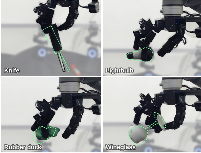
Fig. 10: Difficult out-of-distribution goals reached on the real robot (palm down, state policy; dashed green outline: goal).
