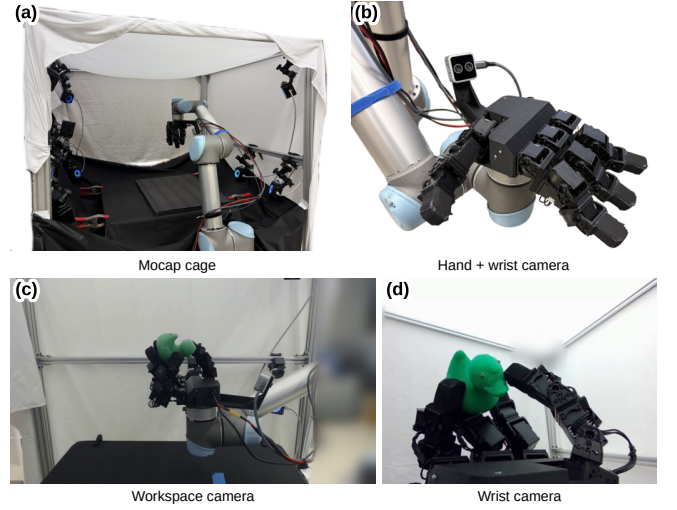
Fig. 2: Hardware setup. (a) The UR5 arm with the LEAP hand inside the motion-capture cage. (b) Close-up of the hand and the wrist-mounted stereo camera. (c) Workspace camera view. (d) Wrist camera view.
