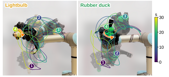
Fig. 11: Rotating object during large arm motion. During a 30s arm trajectory, the depth policy keeps the lightbulb and the duck spinning. Four poses are shown, with the object path colored by time; the orange arrow is the commanded rotation.
