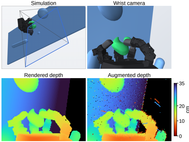
Fig. 18: Simulated depth observations. Scene with distractors, wrist camera view, rendered depth and augmented depth.
