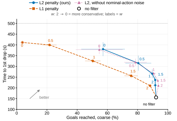
Fig. 28: ResSafe penalty ablation (rubber duck, 3 seeds): L2 penalty (ours), L1 penalty, and L2 without nominal-action noise. Labels give w ; error bars: s.e.m. over seeds.
