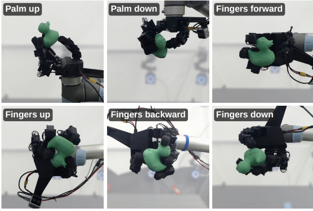
Fig. 7: The six evaluation wrist orientations , which point gravity along each axis of the hand.
