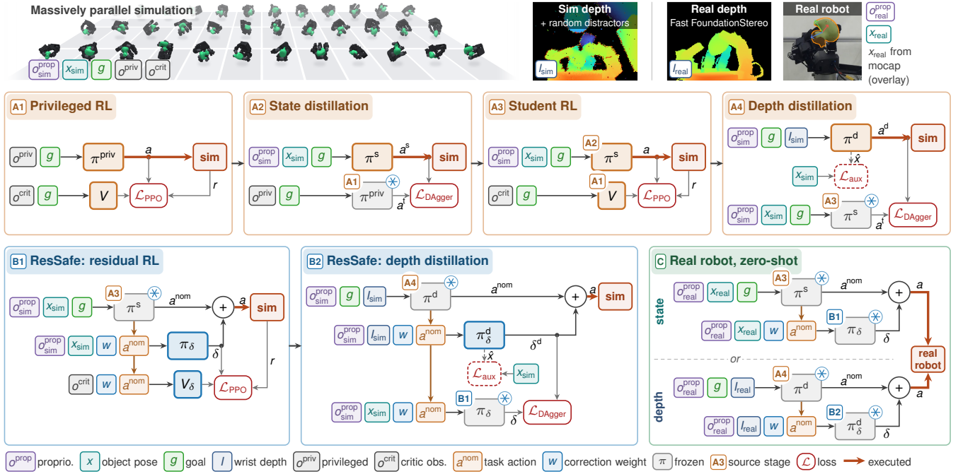
Fig. 4: Training pipeline. A1–A4: The task policy: A1 PPO with privileged observations and an asymmetric critic, A2 DAgger into a deployable state student, A3 PPO fine-tuning of that student, and A4 DAgger into a depth student. B1–B2: The safety filter: B1 learns a residual safety filter on top of the frozen A3 policy; B2 distills it into a depth student filter on top of A4. C: This gives a task policy and a safety filter that use either motion capture or the wrist camera, and both transfer zero-shot to the real robot.
