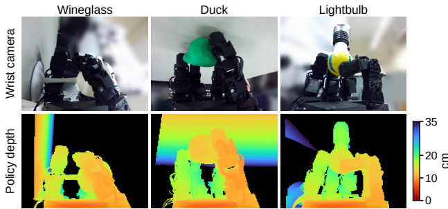
Fig. 14: Wrist-camera input during the tasks of Fig. 13 , with clutter in the background. Camera image (top) and the depth the policy receives (bottom).
