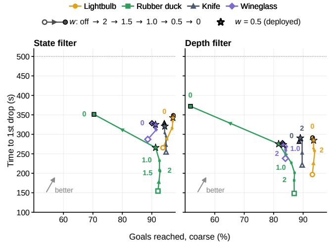
Fig. 5: Effect of the correction weight w in simulation. Coarse goal success vs. time to the first drop, per object, for the state (left) and depth (right) policies, from no filter (hollow) through w = 2 to 0.
