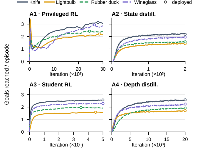
Fig. 21: Training curves of the four task stages (goals per episode). Hollow circles: deployed checkpoints.
