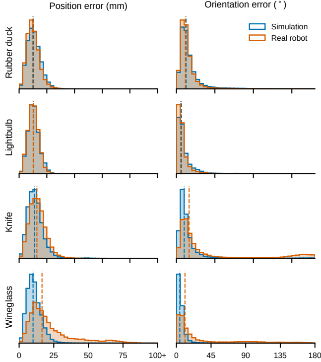
Fig. 26: Object pose perceived by the depth policy. Error of its auxiliary pose head in simulation (blue) and on the real robot (orange); dashed lines are medians.
