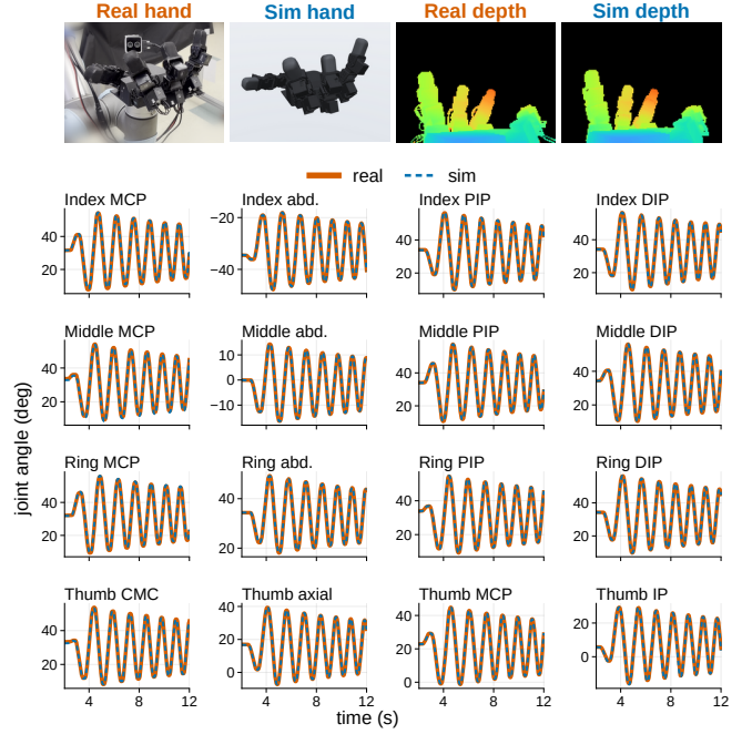
Fig. 16: Sim-to-real check of the identified hand. The same chirp on all 16 actions, played on the real hand and replayed in simulation. Top: hand and wrist depth at the same instant. Bottom: all 16 joints, real (solid) vs. simulated (dashed).
