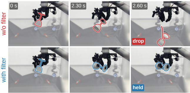
Fig. 8: ResSafe prevents a drop . The same wineglass goal (palm down, depth policy) without the filter (top), where the glass slips and falls, and with it (bottom). The red line traces the falling glass.
