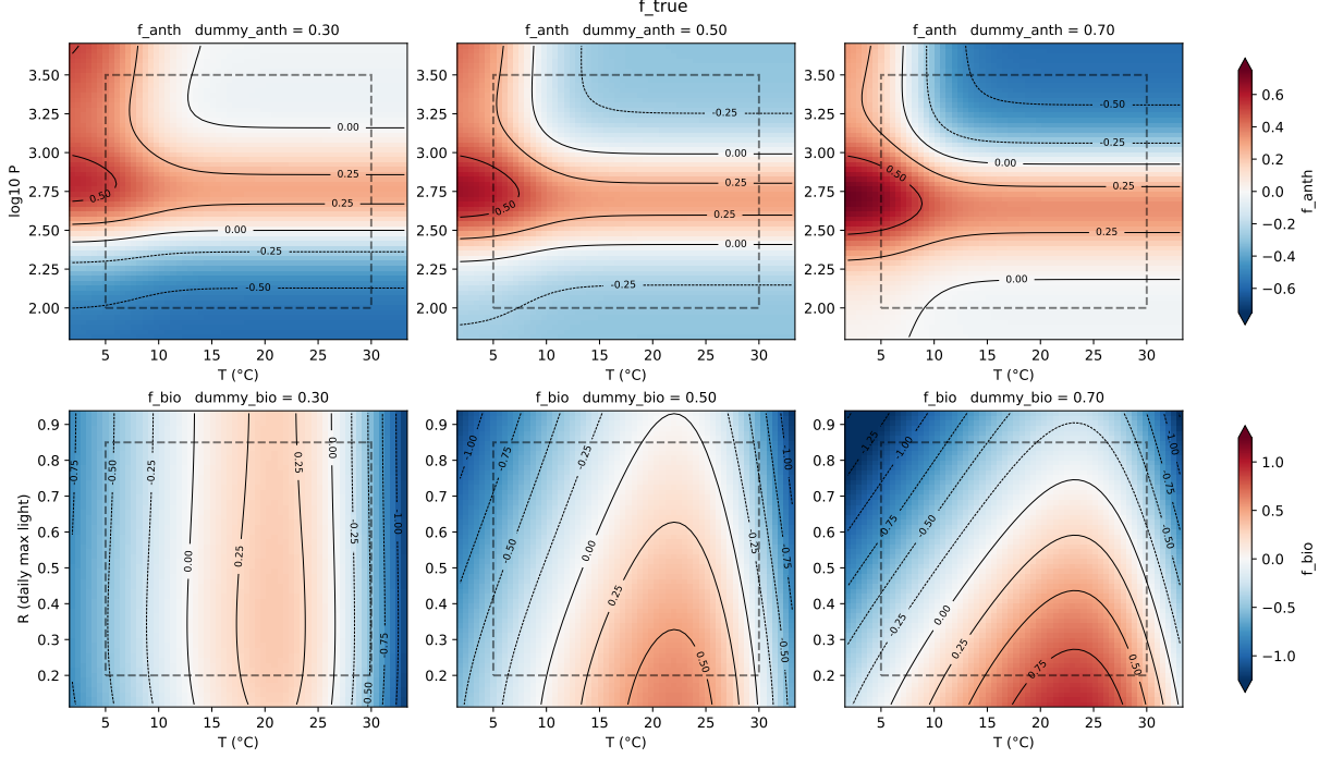
Figure 2: True log emission correction f_s^{\text{true}} (Eqs. 13 and 14) for the anthropogenic (top) and biogenic (bottom) sectors, at three values of the synthetic covariate (columns). The dashed boxes mark the training ranges, and the regions outside them are the extrapolation bands.
