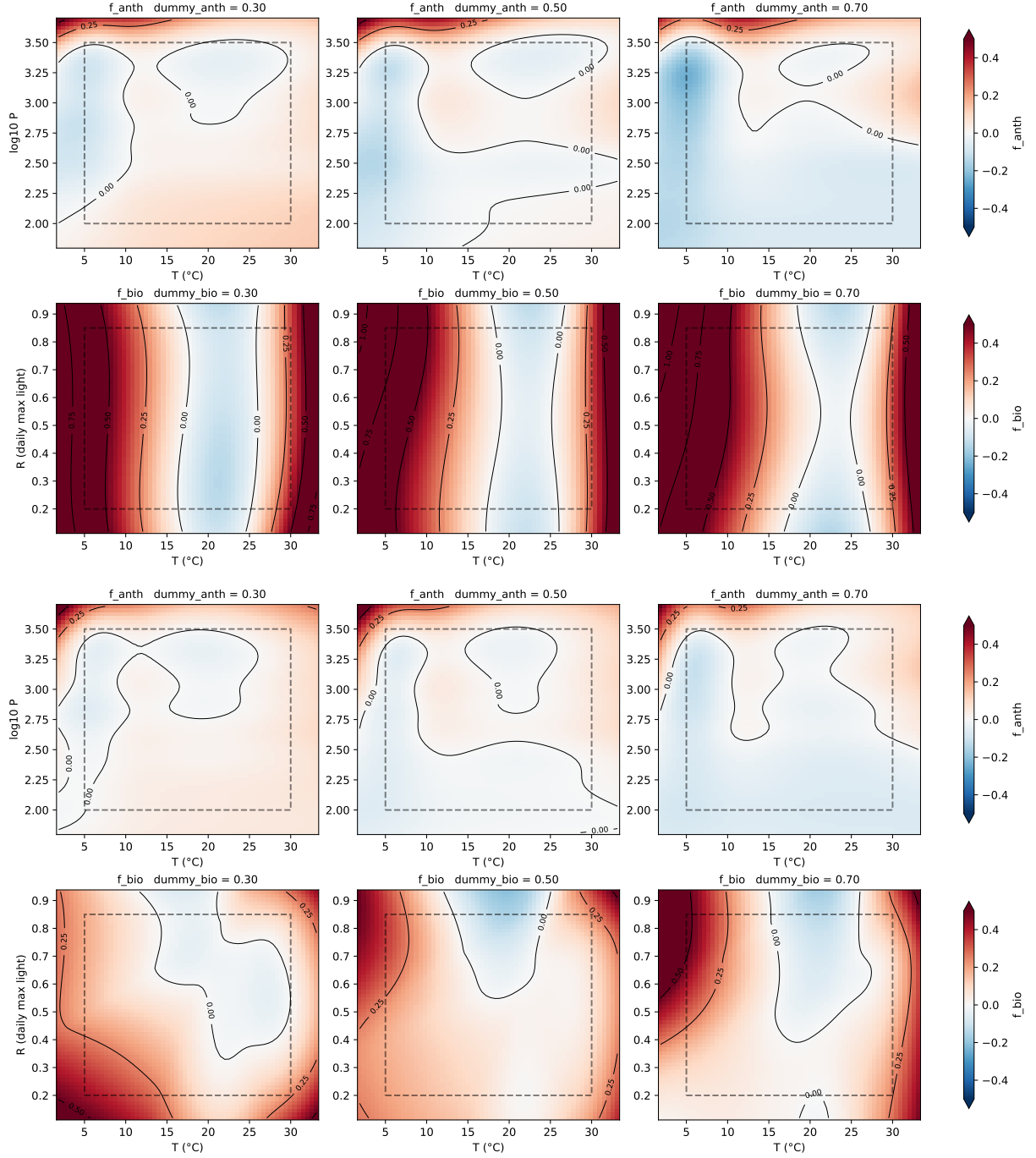
Figure 3: Error of the learned log emission correction, f_s - f_s^{\text{true}} , with noisy station observations, (top two rows) after the offline two-step training and (bottom two rows) after the online Gauss–Newton fine-tuning. In each pair of rows, the top row shows the anthropogenic and the bottom row the biogenic sector, at three values of the synthetic covariate (columns). The dashed boxes mark the training ranges.
