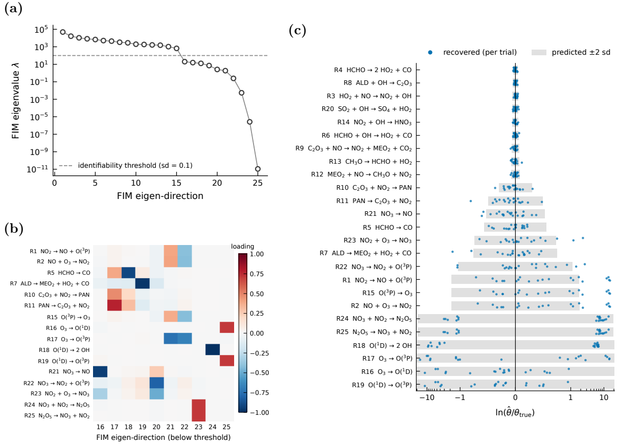
Figure 1: Identifiability analysis and estimation of the 25 POLLU rate coefficients. (a) Eigenvalues of the Fisher information matrix in descending order, where the dashed line marks \lambda = 100 , which corresponds to a Cramér–Rao standard deviation of 0.1 along the eigenvector. (b) Loadings of the ten eigenvectors below this threshold on the rate coefficients that contribute to them. (c) Estimated log rate coefficients relative to the truth in the 20 trials (dots), compared with the interval of \pm 2\sigma_p^{\text{CR}} predicted from the FIM before the fit (grey bars). The horizontal axis is linear between -1 and 1 and logarithmic outside. Reactions are numbered as in POLLU.
