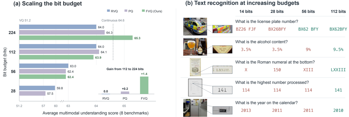
Figure 1 Scaling the bit budget of discrete visual representations. (a) Average multimodal understanding performance improves with the per-patch bit budget. FVQ continues to improve in the high-budget regime and reaches the continuous QwenViT baseline, whereas existing multi-codebook quantizers saturate. (b) Qualitative examples of text recognition at increasing bit budgets. Higher budgets progressively recover the fine-grained textual information required for correct predictions; green and red denote correct and incorrect answers, respectively.
