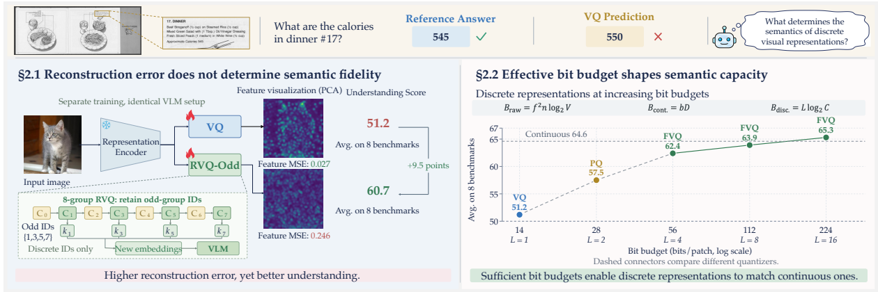
Figure 2 Overview of the analyses in Section 2: reconstruction error versus semantic fidelity (left) and bit-budget scaling across representative quantizers (right). B_{\text{raw}} , B_{\text{cont}} , and B_{\text{disc}} denote per-patch budgets for raw pixels, continuous features, and discrete indices. f , n , V , b , D , L , and C denote patch side length, channels, values per channel, bits per feature dimension, feature dimension, number of codebooks, and codebook size, respectively.
