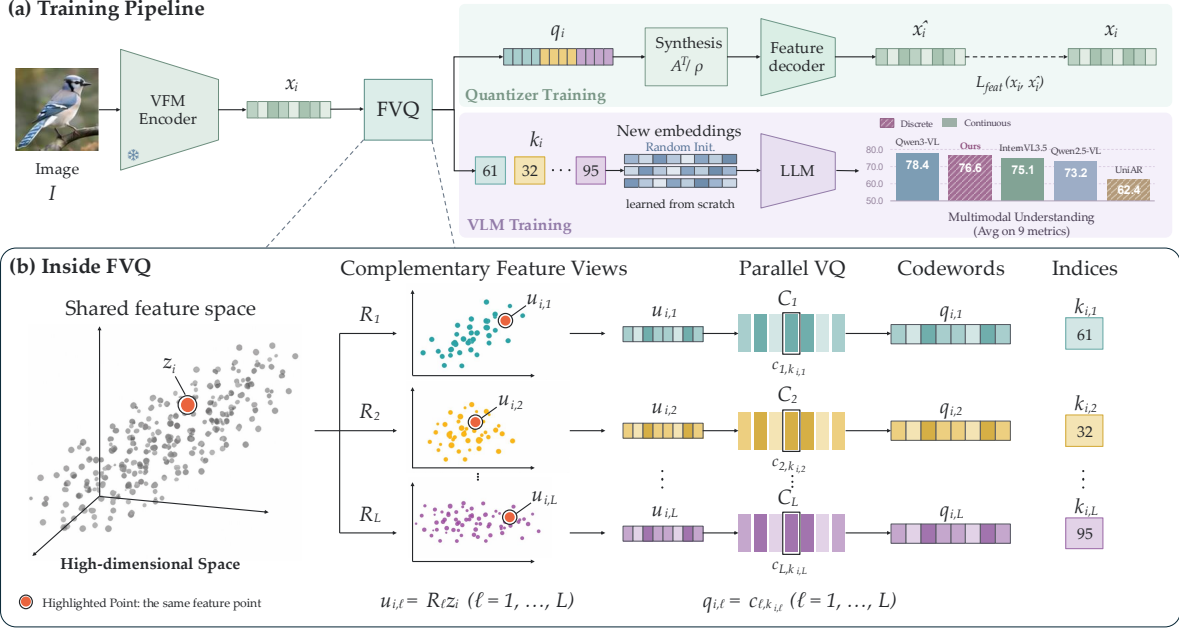
Figure 3 Overview of FVQ. During quantizer training, multiple dense projections produce complementary views of the same visual feature, which are quantized in parallel by independent codebooks. The selected codewords are combined through tight-frame synthesis for feature reconstruction. In the subsequent VLM training stage, the quantizer is frozen, and only the resulting discrete indices are mapped to newly initialized token embeddings for multimodal understanding. The nine-metric average is computed over MMMU, MathVista, MMStar, OCRBench/10, ChartQA, CharXiv-DQ, CharXiv-RQ, DocVQA, and InfoVQA.
