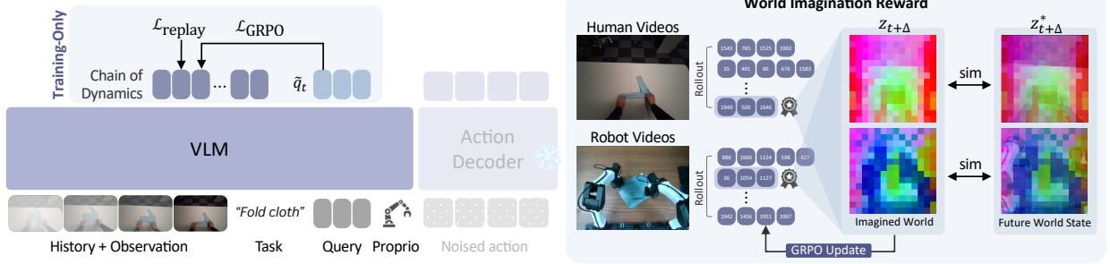
Figure 2: ThinkWorld architecture and training stages. In stage (a), supervised fine-tuning (SFT) tokenizes robot actions and annotated human hand motions into a unified discrete motion space to ground Chain-of-Dynamics (CoD) reasoning, while CoD-conditioned imagination predicts the future visual feature. In stage (b), reinforcement learning (RL) uses the alignment between imagined and observed futures as a scalable reward for CoD reasoning over human and robot videos, strengthening action reasoning without motion annotations and improving guidance for continuous control.
