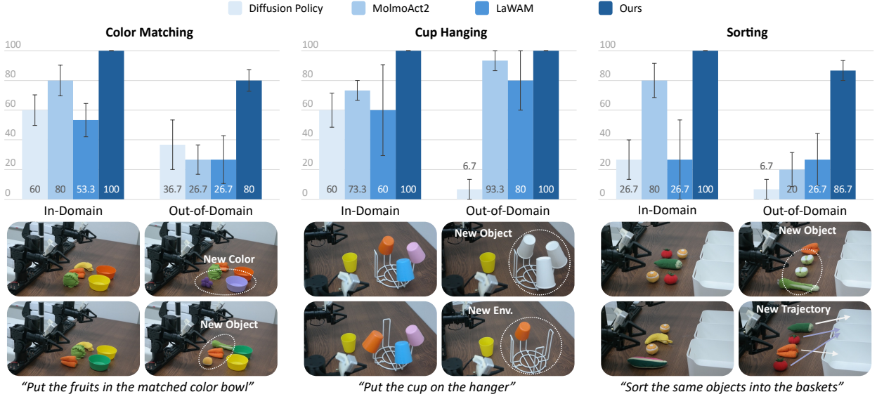
Figure 3: Real-world out-of-distribution (OOD) generalization. Success rates for color matching, cup hanging, and sorting under in-domain and OOD conditions. OOD settings introduce new colors, objects, environments, or sorting trajectories, as illustrated below the plots. ThinkWorld achieves the highest OOD success rates across all three tasks, despite substantial drops for the baselines.
