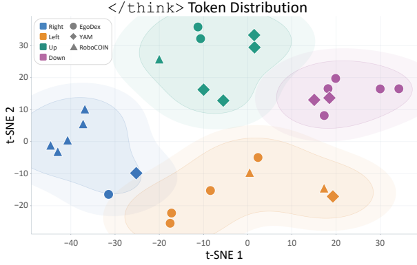
Figure 5: t-SNE visualization of CoD across embodiments. Colors denote four end-effector motion directions and marker shapes denote datasets. Similar motions cluster across human and robot data rather than by source, suggesting action structure shared across embodiments.
