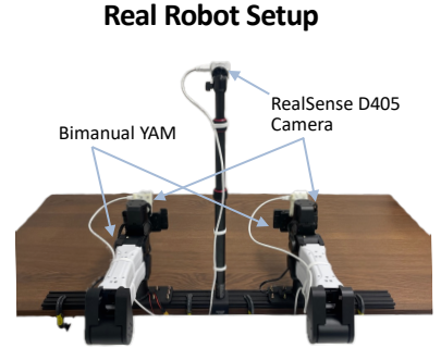
Figure 9: BimanualYAM setup.
