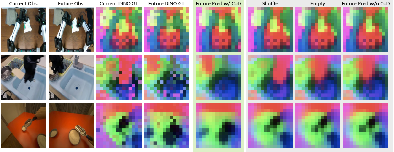
Figure 7: Effect of Chain-of-Dynamics (CoD) on future prediction. We compare future DINO predictions under generated, shuffled, empty, and no-CoD conditions against the current and future ground-truth features. The generated CoD captures the future-state structure, whereas the other variants largely remain similar to the current state and fail to reflect the expected future change.
