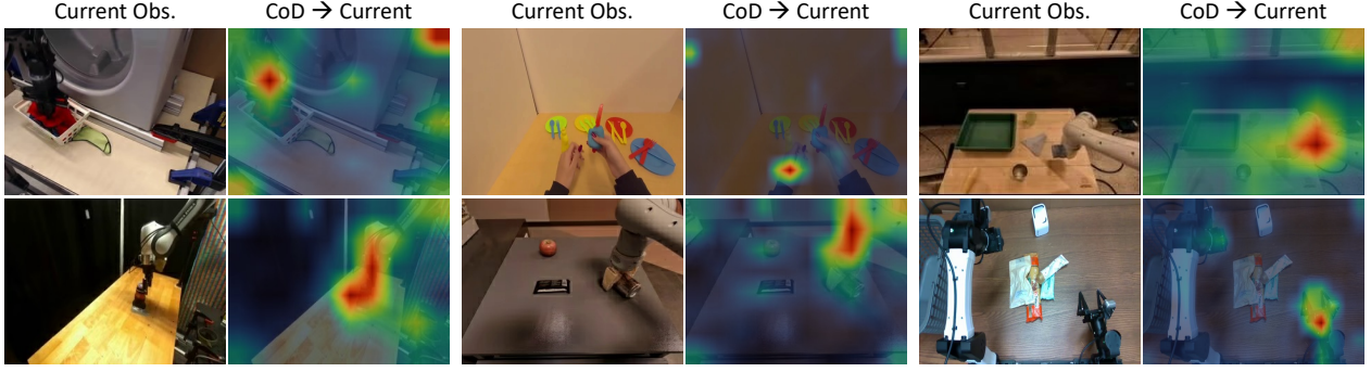
Figure 8: Attention analysis of CoD. We visualize attention from CoD tokens to the current observation. Across human and robot examples, CoD attends to action-relevant regions, including human hands, robot arms, and manipulated objects, highlighting its focus on motion-relevant cues.
