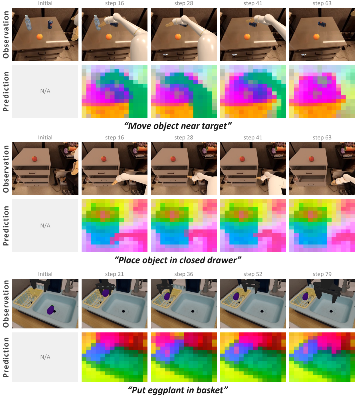
Figure 14: One-second-ahead future predictions during closed-loop SimplerEnv rollouts. For each task, the upper row shows observations actually reached by the policy, while the lower row shows PCA-projected future representations predicted at the preceding replanning horizon. Each column pairs a prediction with the observation at its target time, so their scene structure should correspond. The close qualitative alignment in layout and task progress shows that the predictions track the states encountered during closed-loop execution. The initial frame has no preceding prediction.
