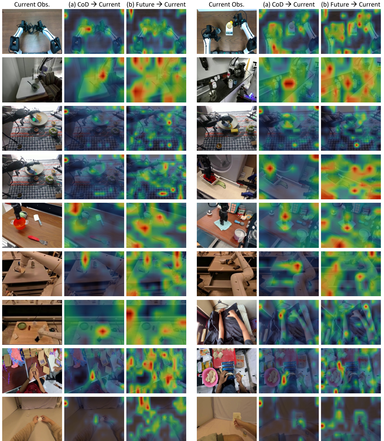
Figure 13: Additional attention visualizations. Attention maps from CoD and future-prediction tokens to the input observation. CoD attention concentrates on dynamic, task-relevant regions, while future-prediction attention is more broadly distributed across the scene.
