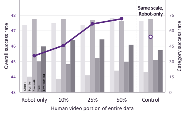
Figure 6: Effectiveness of human data. The LIBERO-PRO evaluation success rates (%) on the model variants trained with different amount of human egocentric video, fixing the robot data quantity. Leveraging human data continuously enhances the performance.
