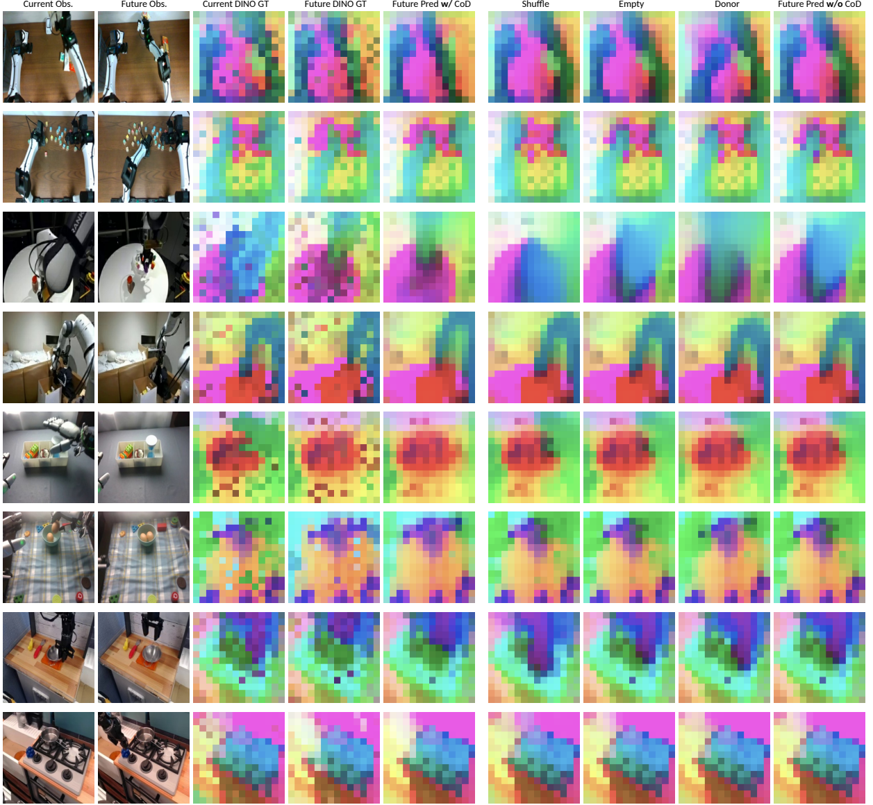
Figure 12: Qualitative future-prediction results. Each row is one episode. The first two columns show the current and ground-truth future RGB observations, and the next two show PCA projections of the ground-truth DINO features for those frames. The remaining five columns show the predicted future DINO features under different CoD conditions: with CoD, shuffled CoD, empty CoD, a CoD taken from a different (donor) episode, and without CoD. All PCA panels share one color mapping.
