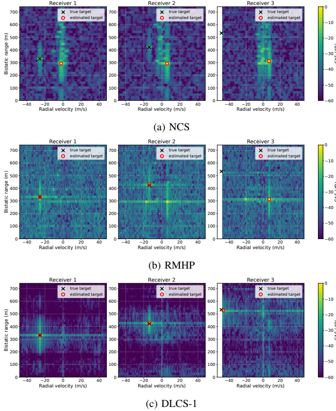
Fig. 4: Bistatic range-Doppler maps.
