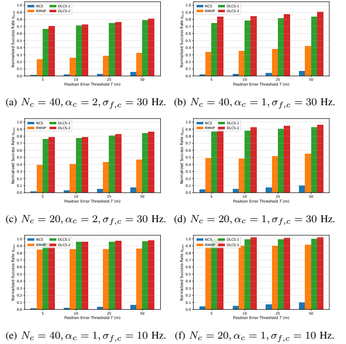
Fig. 5: Normalized success rate \eta_{\text{succ}} versus position error threshold T (m).
