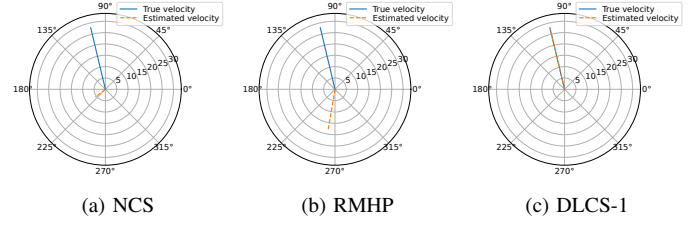
Fig. 2: Velocity estimation results.
