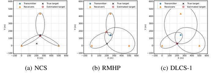
Fig. 3: Target localization results.
