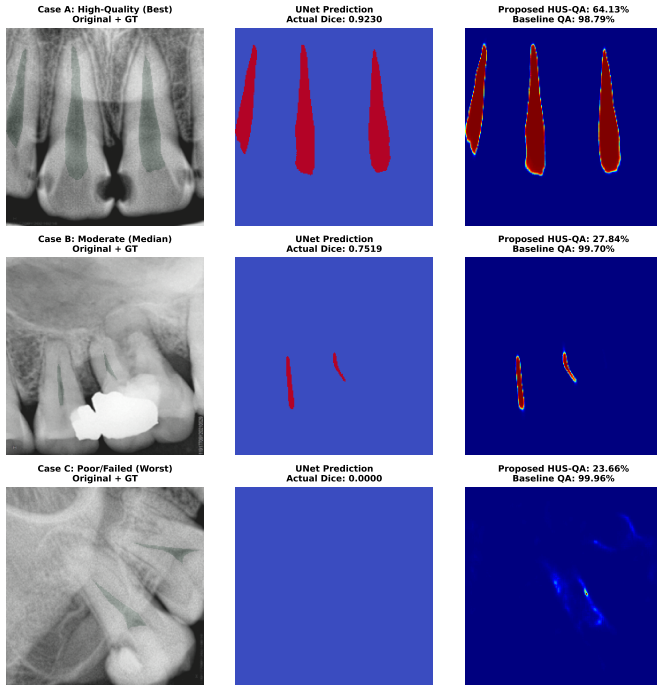
Fig. 5. Visual comparison of segmentation outputs under three quality levels.
