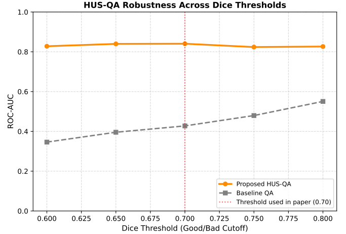
Fig. 4. ROC-AUC of HUS-QA and baseline QA across Dice thresholds from 0.60 to 0.80. The red dotted line marks the 0.70 threshold used in the main evaluation.
