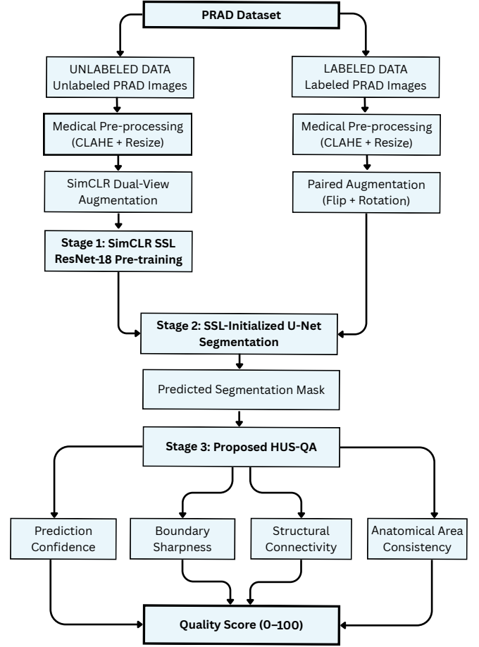
Fig. 1. Overall framework of the SimCLR ResNet-18 U-Net segmentation and HUS-QA quality check pipeline.
