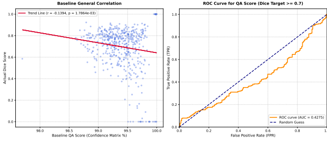
Fig. 2. Quality checking performance using standard confidence baseline.
