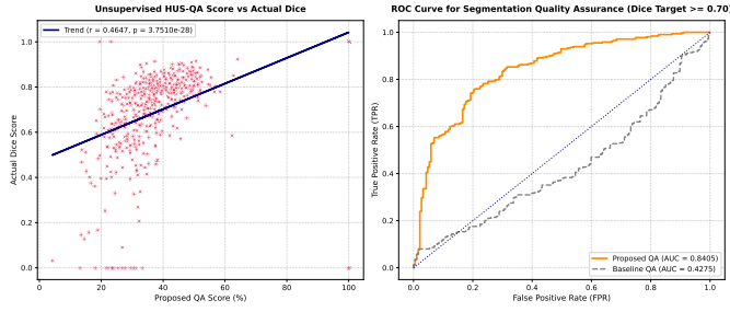
Fig. 3. Quality checking performance using the proposed HUS-QA framework.
