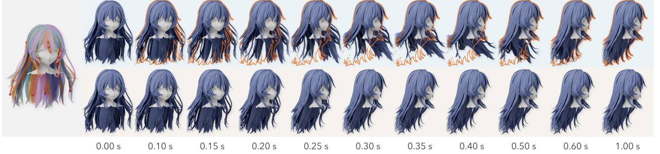
Figure 8. Generated spring bones in motion. Left: the generated cards (transparent) with their generated spring-bone chains. Right: a 50° head turn; top row with the chains, bottom row without them. The orange outline marks the hair without spring bones in the same frame.
