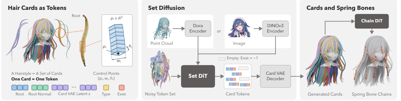
Figure 2. Overview. Left: a hairstyle is a set of hair cards. Each card, a polyline of control points with width and thickness, becomes one token holding its root position, root normal, card VAE latent \mathbf{z} , cross-section type and existence flag. Middle: the set DiT denoises the token set with flow matching, attending across cards and to the condition, a point cloud or an image. Empty slots let the model decide how many cards to generate. Right: the card VAE decodes the tokens into cards, and the chain DiT generates their spring-bone chains.
