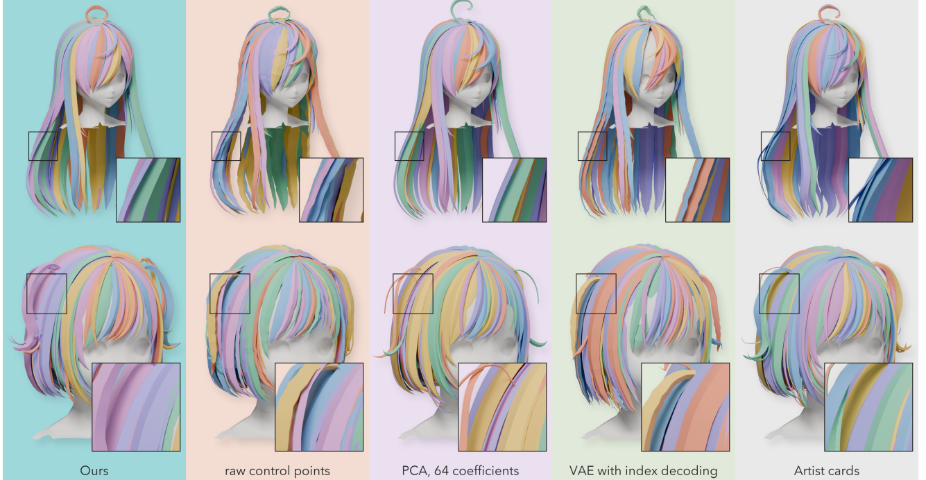
Figure 15. Card tokens. A set DiT of the same architecture, trained with each card token of Tab. 6, generates two test hairstyles from point clouds; insets magnify the same window in each row. Raw control points and the VAE with index decoding give jagged cards, PCA with 64 coefficients gives straighter cards than the artists’, and our latent gives cards as smooth as theirs. Each card has its own color.
