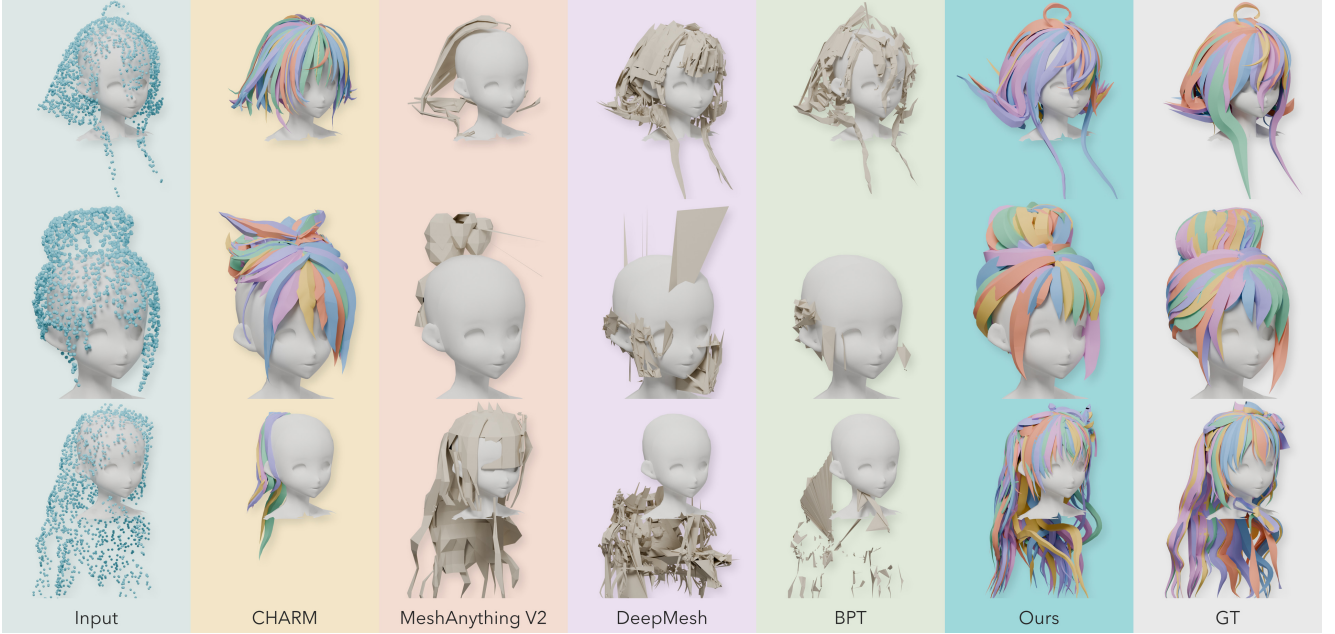
Figure 4. Point clouds from CHARM’s test set. CHARM and HairDeck output hair cards, colored per card like the artist ground truth; MeshAnything V2, DeepMesh and BPT output meshes. All results are shown on a fixed head at each character’s placement.
