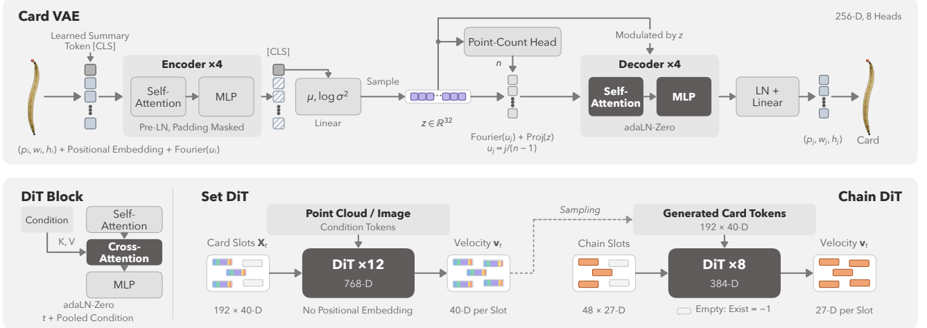
Figure 3. Network design. Top: the card VAE. The encoder reads the control points of one card with their arc-length fractions u_i , plus a learned summary token [CLS], whose output alone gives the mean and log-variance of the 32-d latent \mathbf{z} . The decoder predicts the number of points n and evaluates the card at n uniformly spaced arc-length fractions, modulated by \mathbf{z} (adaLN-Zero). Bottom: both DiTs use the same block design (left), modulated by the timestep and the pooled condition. The set DiT predicts the velocity of 192 card token slots without positional embedding, conditioned on a point cloud or an image. The chain DiT does the same for 48 spring-bone chain slots, conditioned on the card tokens sampled by the set DiT (dashed arrow). Empty slots (dashed boxes) have existence -1 , filled ones +1 .
