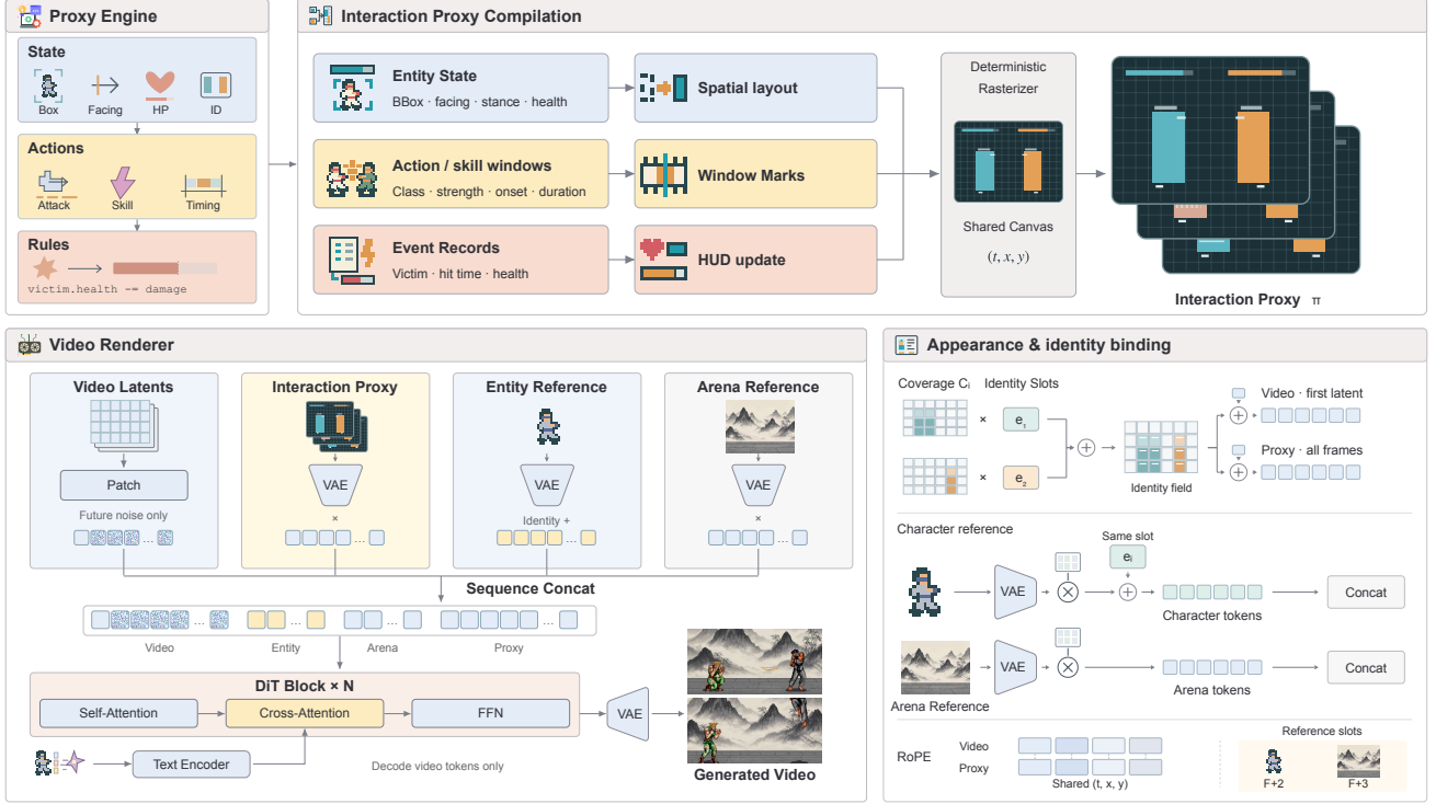
Figure 2: Overview of FWM. The Proxy Engine executes gameplay rules, and the resulting state trajectories, action windows, and events are compiled into a visual interaction proxy. The proxy and appearance references are encoded with a shared VAE and concatenated with video tokens. Matching spatiotemporal rotary positions align the proxy with the video, while shared identity embeddings bind character references to the corresponding regions in the first video latent and proxy sequence. The DiT processes the combined sequence, and only video tokens are decoded to generate the continuation.
