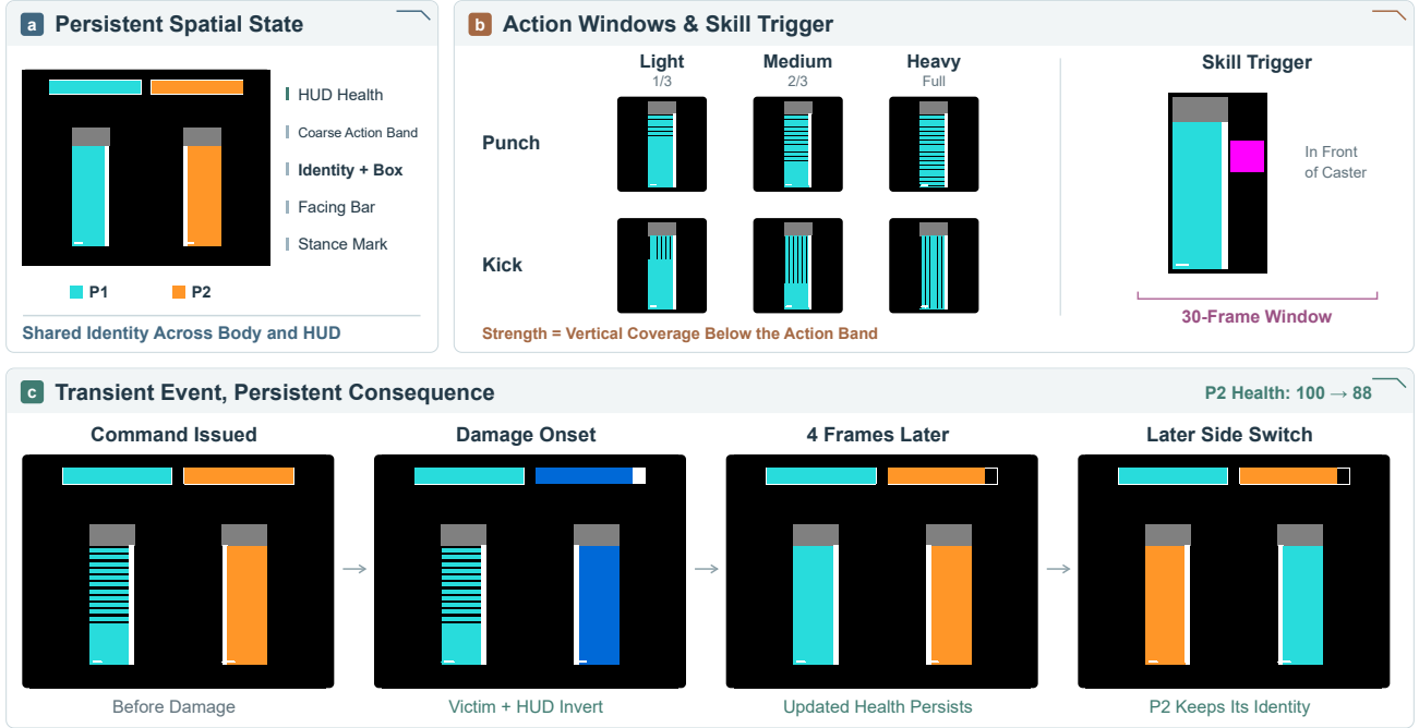
Figure 10: Interaction-Proxy Vocabulary. Transient cues and persistent state share fighter identities.
