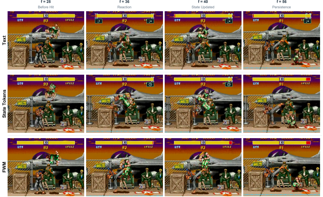
Figure 6: Complete-Information Encodings on the Same Interaction. Held-out rollout under matched executed records (Table 2). Green brackets mark HUD state errors: [!] unexpected health loss, [x] missing health loss, [O] delayed update, [≠] incomplete update, and [↑] unexpected recovery.
