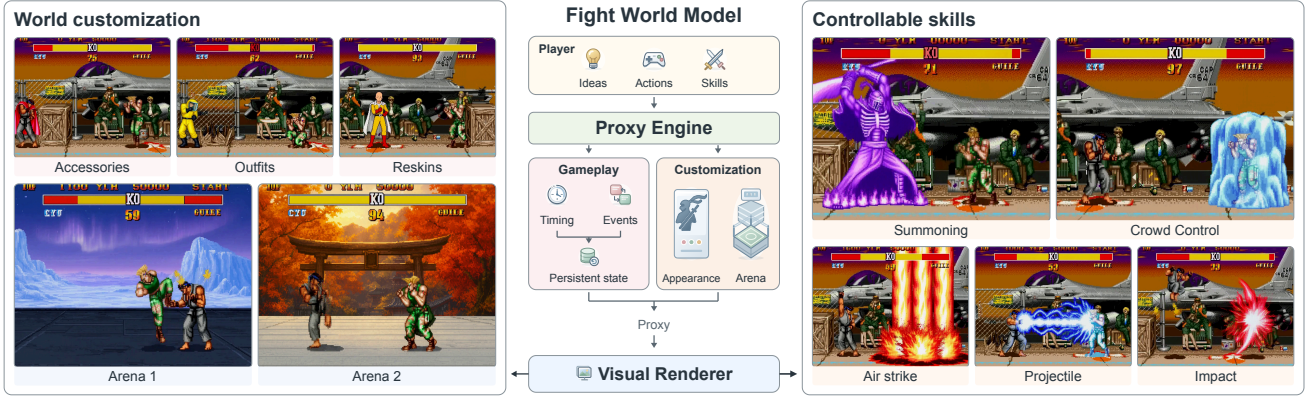
Figure 1: Customizable Combat with FWM. Character and arena customization is shown on the left, and controllable skills on the right. The central pipeline connects rule execution to video rendering through an interaction proxy.
