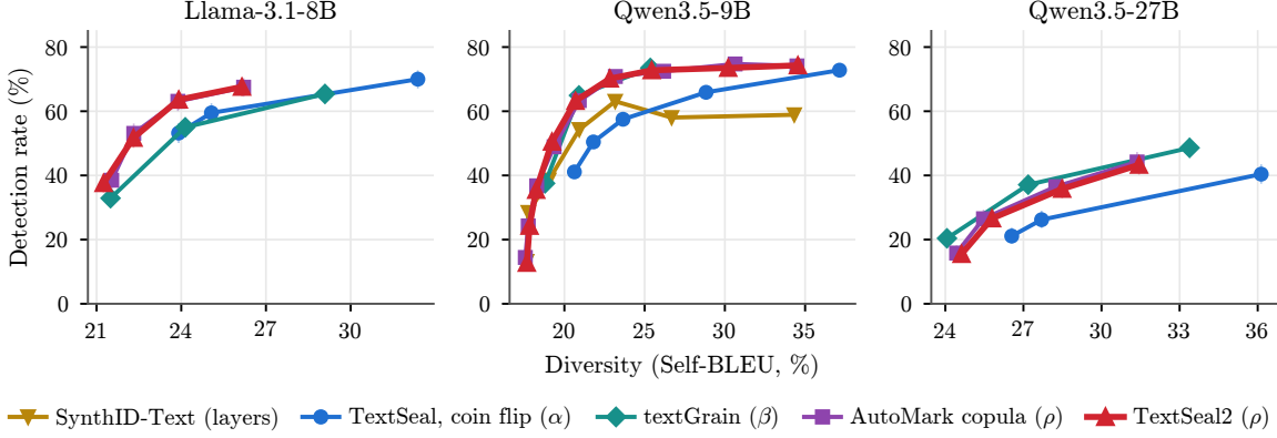
Figure 7 Diversity (Self-BLEU; lower is more diverse) vs. detection of 100-token answers without speculative decoding, on three models (32 answers to each of 100 questions; copulas with the 53-bit PRF). Interpolated at TextSeal’s Self-BLEU, TextSeal2 gains 10, 22 and 8 percentage points over the coin flip on Llama-3.1-8B, Qwen3.5-9B and Qwen3.5-27B respectively, and AutoMark’s copula overlaps TextSeal2 throughout.
