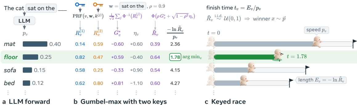
Figure 2 TextSeal2 generates one token (subsection 3.1). (a) The model’s forward pass gives the probabilities p_v , and the last k = 3 tokens form the window \mathbf{w} . (b) The keys’ values at \mathbf{w} are merged into the virtual key G_v^* , which the copula (4) blends with the noise \eta_v into \tilde{R}_v ; the Gumbel-max choice is \arg \min_v (-\ln \tilde{R}_v)/p_v . (c) The Gumbel-max choice can be seen as a race (1): candidate v runs a lane of length E_v = -\ln \tilde{R}_v at speed p_v , and the token that finishes first is chosen.
