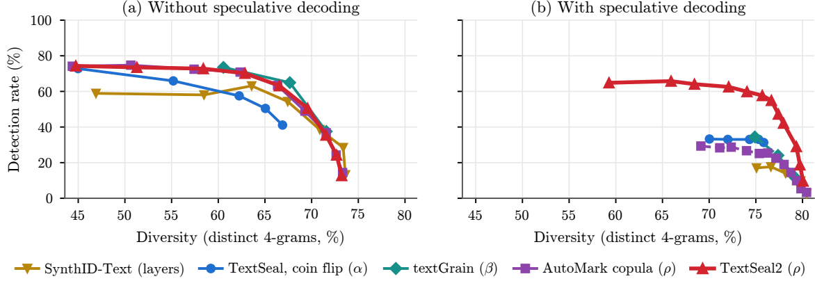
Figure 10 Figure 1 with diversity measured by the share of distinct 4-grams (higher is more diverse), including the speculative panel (b).
