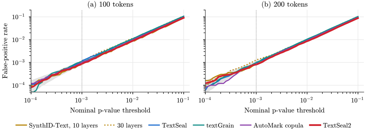
Figure 9 Calibration: false-positive rate against the nominal p-value threshold for the detectors of Table 1 without speculative decoding, on 10 keys and 10,000 unwatermarked Qwen3.5-9B answers; grey: 95% binomial interval around the diagonal. At 10^{-3} and above, every detector is within a factor 1.3 of nominal.
