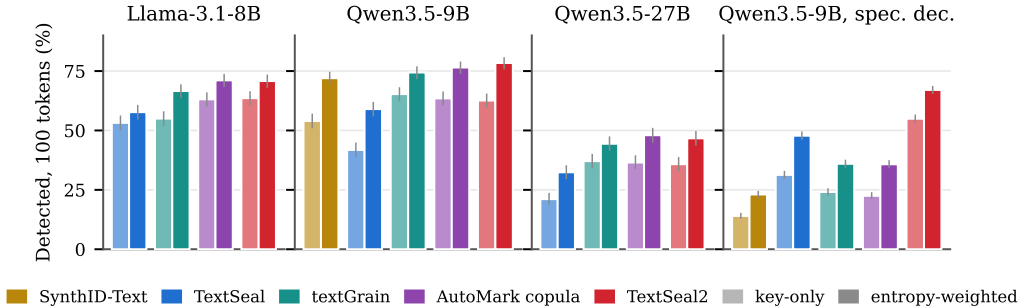
Figure 5 Entropy weighting improves detection for every watermark, including under speculative decoding. % of 100-token answers detected at a false-positive rate of 10^{-3} with key-only scores (light bars) and with TextSeal’s entropy-weighted test (full bars), at comparable Self-BLEU. The gains are 5–18 percentage points at 100 tokens and 4–23 at 200 tokens (Table 6); without speculative decoding, TextSeal2 and AutoMark’s copula coincide in distribution and differ only within their 95% intervals, as expected.
