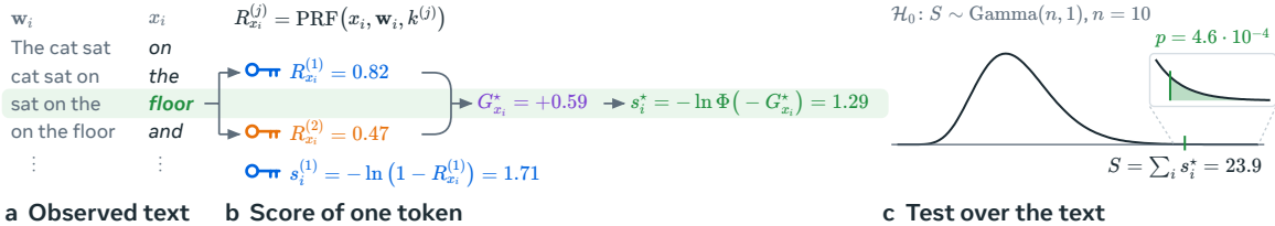
Figure 4 TextSeal2 detects the text “The cat sat on the floor and fell asleep in the sun.” ( subsection 3.4 ). (a) Each token x_i and its window w_i ; the highlighted row is the token of Figure 2 . (b) For “floor”, the keys’ values are merged into G_{x_i}^* as in (4), without the noise, and give the score s_i^* ; key k^{(1)} alone gives the public score s_i^{(1)} . (c) The n = 10 scores sum to S = 23.9 , and the \text{Gamma}(n, 1) tail beyond S (box) is p = 4.6 \cdot 10^{-4} .
