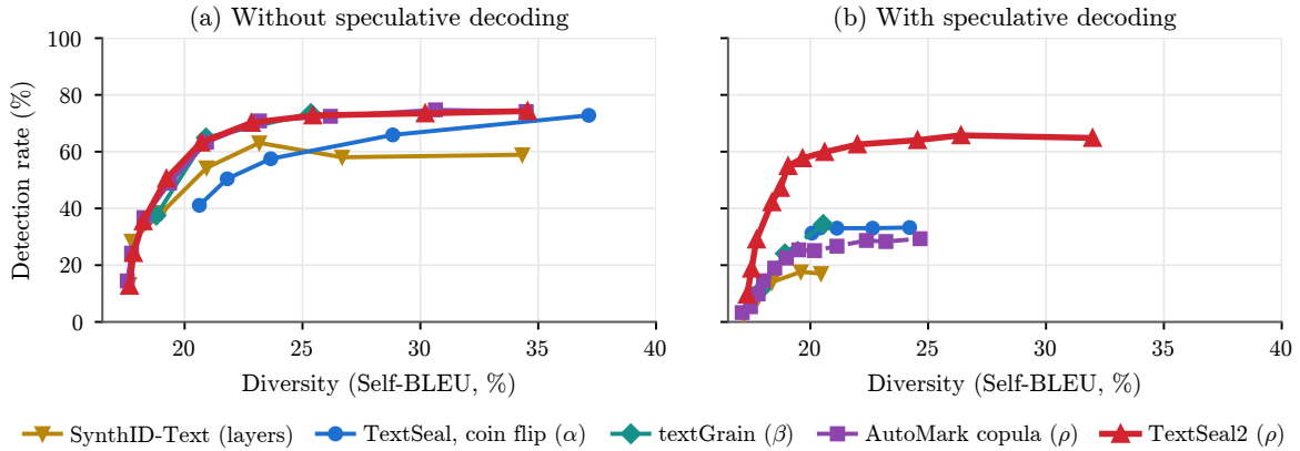
Figure 1 Diversity–detection trade-off on Qwen3.5-9B at 100 tokens at \text{FPR}=10^{-3} , (a) without and (b) with speculative decoding (8 drafts per round, block verification). In (a), TextSeal2 coincides with AutoMark’s single-key copula as expected since it behaves like a single-key copula. In (b), TextSeal2 uses the residual race, and the baselines use block verification’s native stopping rule with the last token of each round drawn under an independent key. Diversity is measured by Self-BLEU (lower is more diverse).
