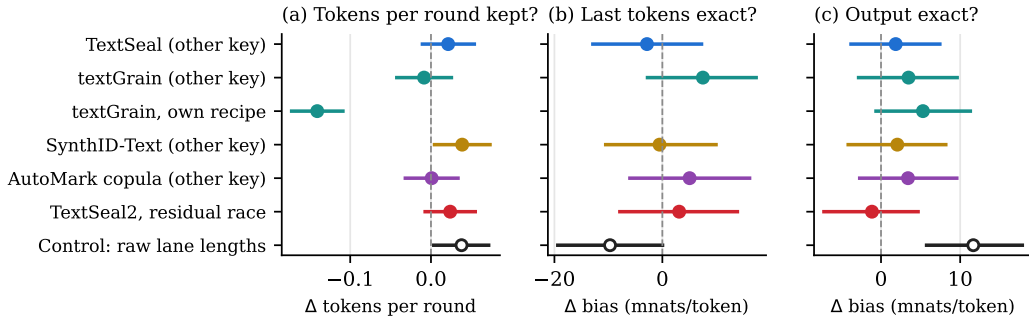
Figure 11 Is speculative decoding with a watermark still distortion-free? Paired differences from unwatermarked block verification (8 drafts per round) on the same 480 prompts, with one key per answer (95% paired bootstrap intervals). (a) Tokens per round. (b) Mean of -\ln r_{I,y} - H(\vec{r}_I) at the last token y of each round, which has expectation zero when it follows block verification’s residual law \vec{r}_I (not shown for textGrain’s own recipe, whose last token follows the residual of the watermarked distributions). (c) Mean of -\ln p_x - H(\vec{p}) over all tokens, which has expectation zero for any distortion-free scheme. Only the control (racing on raw lane lengths, Remark 1) deviates in (c), and only textGrain’s own recipe lowers tokens per round.
