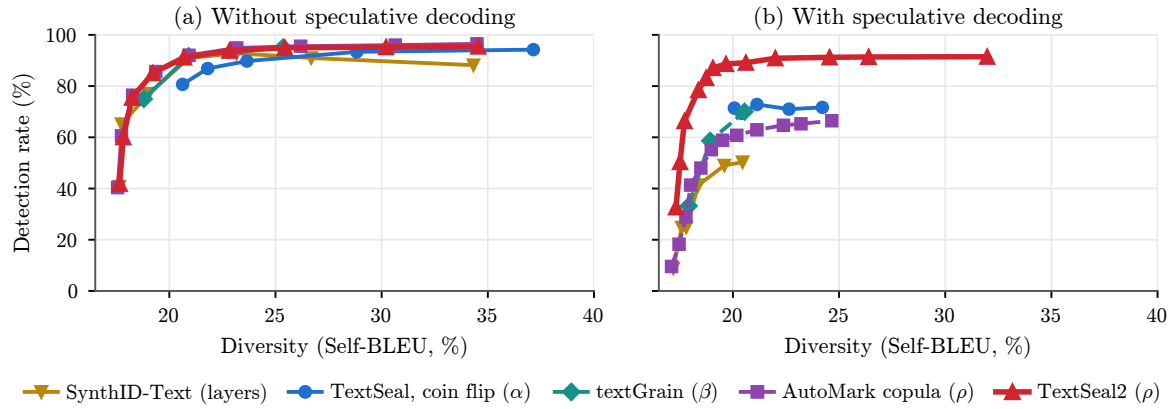
Figure 6 The diversity–detection trade-off of Figure 1 at 200 tokens instead of 100; same protocol and conventions, including the speculative panel (b).
