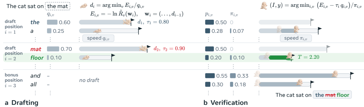
Figure 3 Block verification checks the drafts against the target as a block, keeps those before a stop position I , and emits one token y at I . (a) The drafter proposes “the mat” with keyed races. (b) One target pass then gives the probability \pi_{i,v} that I = i and y = v . One more race on the leftovers picks I and y : “floor” wins, so the round keeps “the” and emits “floor” at I = 2 . TextSeal2 preserves the target’s distribution and block verification’s acceptance rate (Proposition 1). Algorithm 1 in the appendix gives more details.
