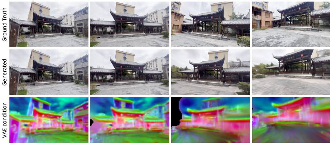
Figure 9: Visualization of latent 3D Gaussian memory conditioning for video generation. We visualize the ground-truth and generated video, with target-view rendered VAE condition from the latent 3D Gaussian memory, illustrating that spatially aligned latent memory provides consistent conditioning for video generation.
