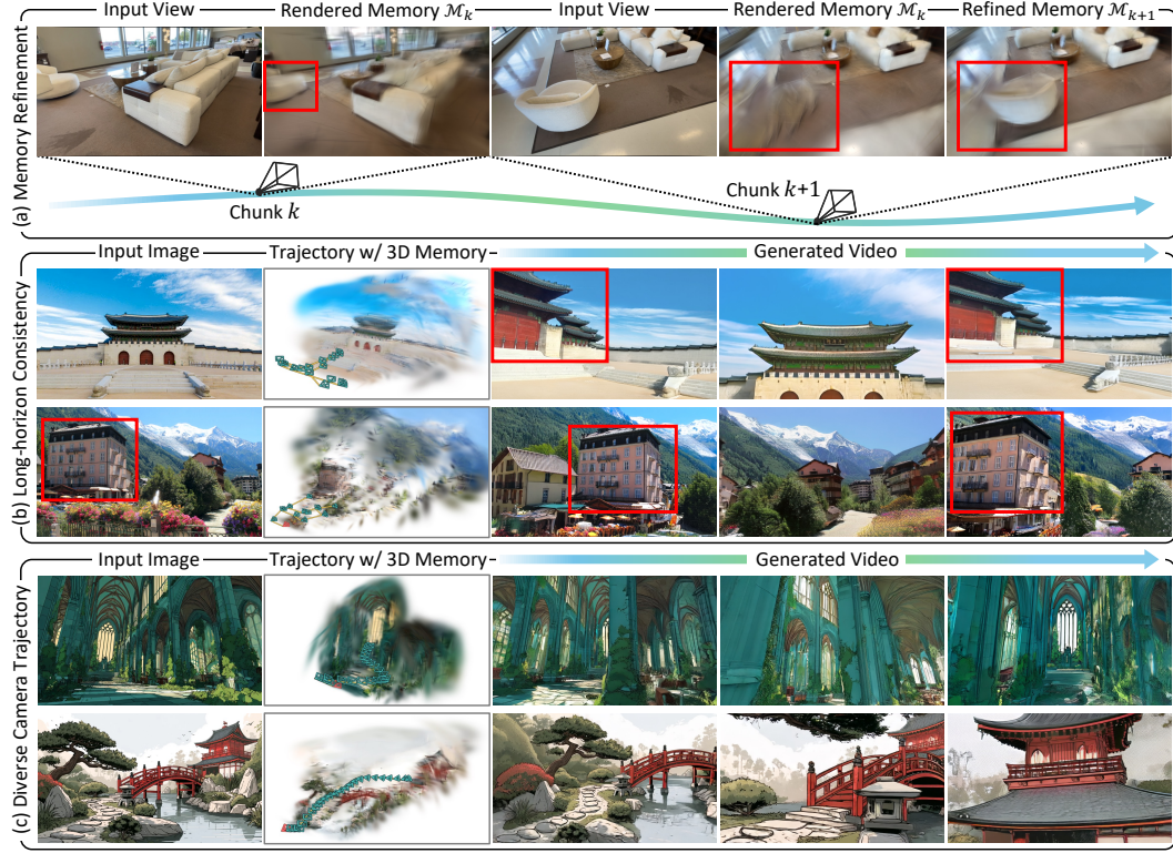
Figure 5: Qualitative results of L3G-World. (a) L3G-Mem corrects geometric errors in the 3D memory through residual refinement using video chunks generated by L3G-Gen. (b) L3G-World maintains scene consistency over long-horizon generation through its persistent 3D memory. (c) Rendering the memory’s VAE features from target camera views provides spatially aligned conditioning, enabling consistent video generation along diverse camera trajectories.
