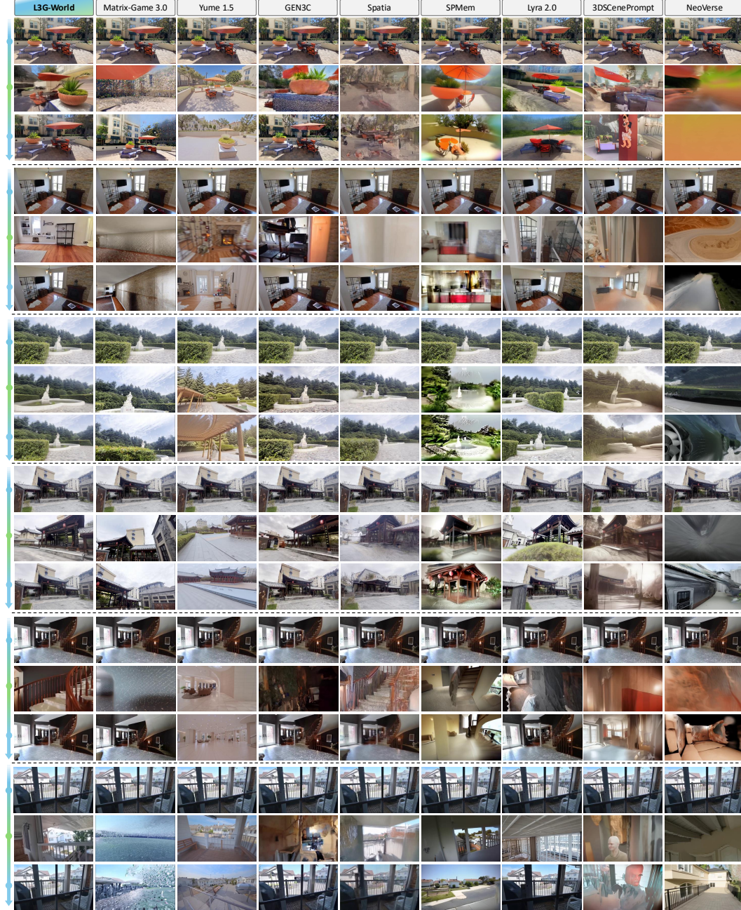
Figure 8: Additional qualitative results of video generation on DL3DV and RealEstate10K. For each scene, all methods start from the same input view (top), explore unseen regions (middle), and return to the initial camera location (bottom). L3G-World preserves scene structure and appearance upon loop closure, whereas the baselines exhibit drift, blur, or rendering artifacts.
