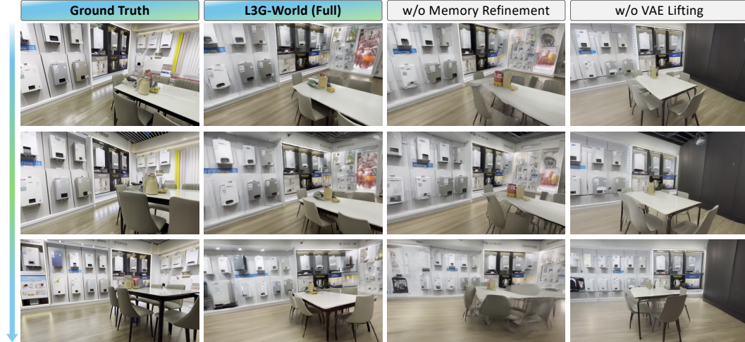
Figure 7: Qualitative results of ablation study of L3G-World on DL3DV. Memory refinement can not fix geometric error in 3D memory, leading blurry video due to memory rendering artifacts.
