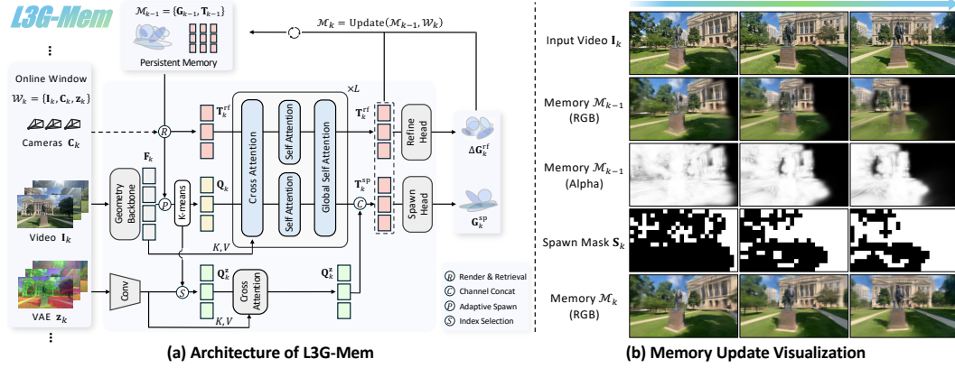
Figure 2: L3G-Mem. (a) L3G-Mem takes the current window \mathcal{W}_k and the memory \mathcal{M}_{k-1} . Rendering \mathcal{M}_{k-1} into the current cameras determines which geometry features are clustered by K-means into spawning queries, and identifies the visible Gaussians whose memory tokens are retrieved as refinement tokens. Both token sets are jointly processed by a transformer and decoded into new Gaussians and residual updates, respectively. (b) Given the input video chunk, RGB and opacity rendered from the previous memory identify regions requiring new Gaussians through a spawning mask. As a result, the updated memory can fully reconstruct the observed scene.
