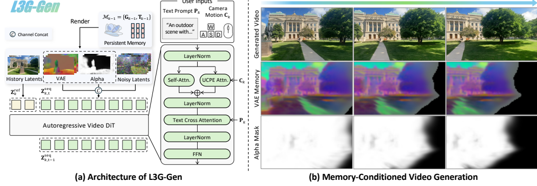
Figure 3: L3G-Gen. (a) L3G-Gen renders the VAE latents and opacity of the 3D memory to the target cameras, concatenates them with the noisy latents along the channel dimension, and generates the next chunk conditioned on the history latents. (b) We visualize the ground-truth and generated video, with target-view rendered VAE condition from the latent 3D Gaussian memory, illustrating that spatially aligned latent memory provides consistent conditioning for video generation.
