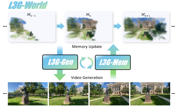
Figure 4: L3G-World Pipeline. L3G-World couples video generation and memory updating in a chunk-wise loop, where each generated chunk updates the persistent 3D memory, which in turn conditions subsequent chunk generation.
