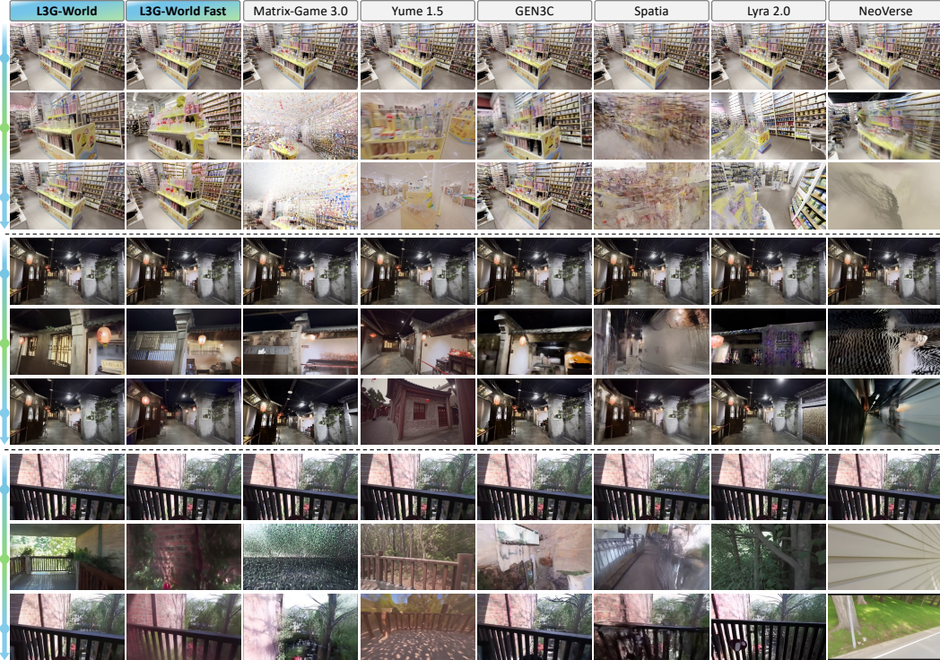
Figure 6: Qualitative results of video generation on DL3DV and RealEstate10K. For each scene, all methods start from the same input view (top), explore unseen regions (middle), and return to the initial camera location (bottom). L3G-World preserves scene structure and appearance upon loop closure, whereas the baselines exhibit drift, blur, or rendering artifacts.
