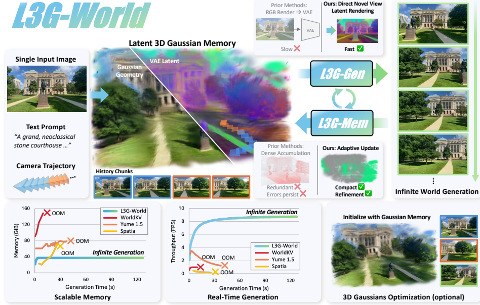
Figure 1: Teaser. L3G-World generates an explorable, spatially consistent world in real time from a single image and a camera trajectory. To this end, L3G-Mem maintains a latent 3D Gaussian memory, and L3G-Gen generates video conditioned on VAE latents rendered from the memory.
