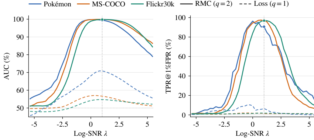
Figure 7: Reference calibration across noise levels. AUC (left) and TPR@1%FPR (right) for the realistic Pokémon, MS-COCO, and Flickr30k fine-tunes. Solid curves show RMC ( q = 2 ). Dashed curves show the uncalibrated fine-tuned loss from the same noise draw ( q = 1 ). Each point uses a fixed score direction, with lower loss or calibrated residual indicating membership. The vertical guide marks \lambda = 1 , the operating point reported in Table 1.
