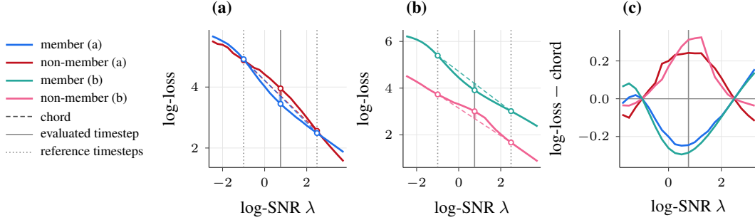
Figure 3: Temporal self-calibration. (a) A member/non-member pair where absolute loss correctly identifies the member. (b) A pair where absolute loss fails because the member is harder, yet a localized "dip" is still visible. (c) Subtracting the local temporal reference (the chord between the reference timesteps) removes the absolute difficulty offset. Both pairs collapse into a shared calibrated view, distinctly separating members from non-members by their trajectory shape.
