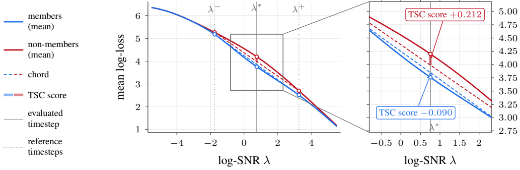
Figure 4: TSC on STL-10-U. Mean member and non-member log-loss trajectories (left) and a close-up of the selected window (right). The chords connect the two context points for each population, and the vertical bars at \lambda^* show the residual measured by the temporal score.
