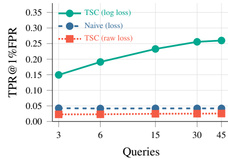
Figure 5: Score domain and query budget. Mean TPR@1%FPR over 8 DDPM checkpoints at matched query budgets. Both TSC scores use the same temporal stencil.
