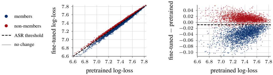
Figure 2: RMC on MS-COCO. Stable Diffusion fine-tuned on MS-COCO in realistic settings, uncaptioned. Left: Pretrained and fine-tuned log-losses are almost perfectly correlated (Pearson correlation r = 0.989 ). Right: Subtracting the pretrained loss removes this shared difficulty. Members shift below the ASR threshold (dashed ASR 98.6%), while non-members stay concentrated near 0.
