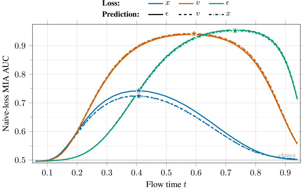
Figure 6: Membership localization across training losses. Single-timestep absolute-loss AUC on the nine first-half CIFAR-100 DDPM++ models without augmentation at epoch 2000. Color denotes training-loss target s and line style denotes native prediction p . Losses are averaged over 50 noise draws per image, shared across noise levels. Lower loss indicates membership at every level. Stars mark single-timestep AUC maxima. The peaks occur at \lambda = -0.75, 0.75 , and 2.00 for x -, v -, and \epsilon -loss, respectively.
