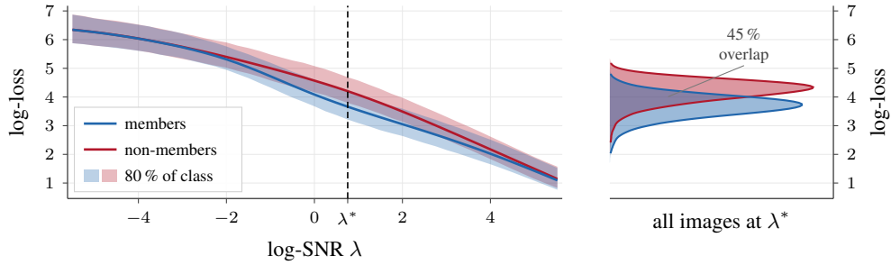
Figure 1: Image difficulty confounds absolute-loss thresholds. Left: CIFAR-10 DDPM log-loss trajectories for members (blue) and non-members (red) showing class means and 80% intervals. Right: Loss density at the optimal log-SNR ( \lambda^* ). Even at maximal separability, the populations exhibit a massive 45% overlap, rendering absolute-loss thresholds ineffective.
