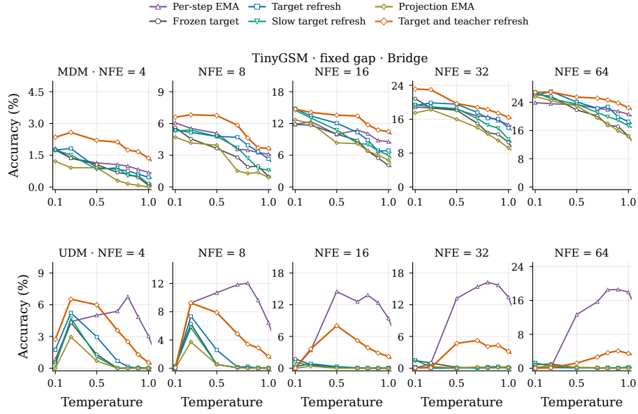
Figure 13: TinyGSM target-update policies with a fixed training gap, under bridge sampling.
