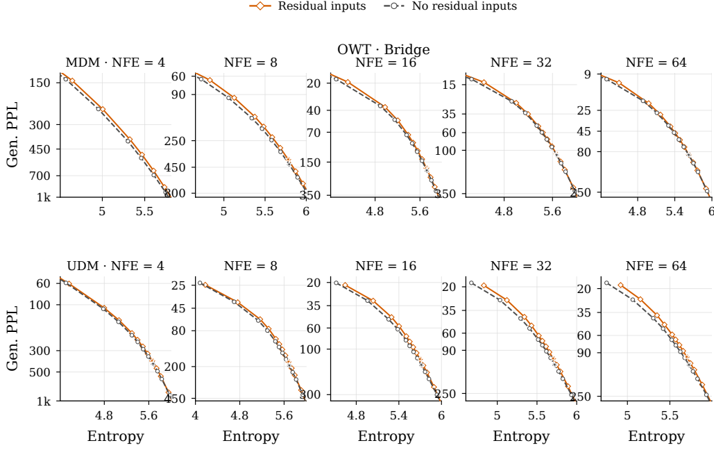
Figure 39: OWT Gumbel-input comparison for MDM and UDM under bridge sampling at five NFEs and fourteen temperatures.
