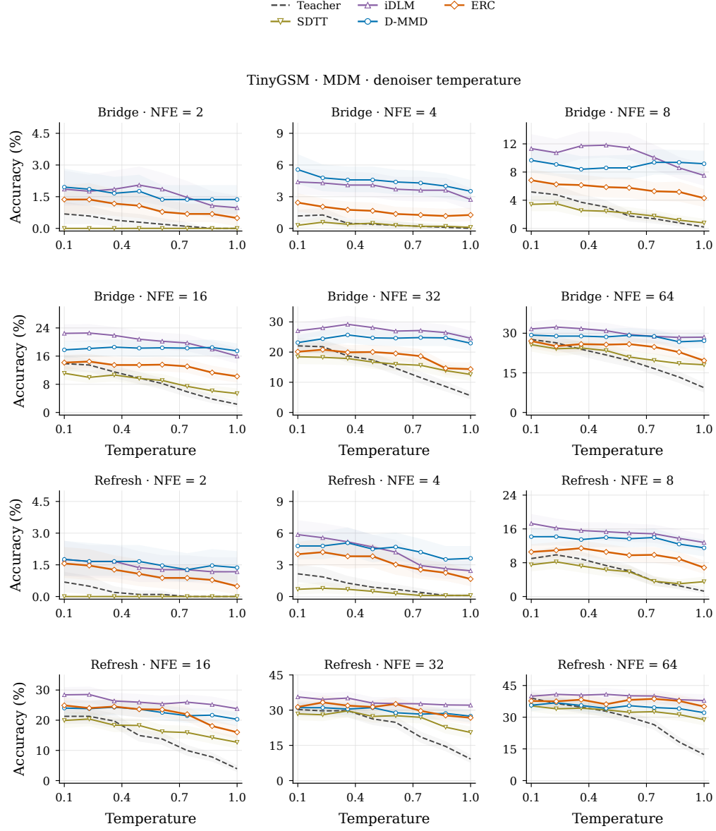
Figure 28: TinyGSM MDM accuracy across eight denoiser temperatures and six NFE budgets for bridge and refresh sampling. Shaded bands are pointwise 95% bootstrap intervals over questions.
