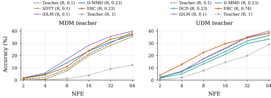
Figure 3: TinyGSM distillation at 2–64 NFEs. Each curve fixes its sampler and temperature to maximize mean accuracy across NFEs on the same 1,024 questions. ERC selects \delta = 1/64 for MDM and 1/8 for UDM. R refers to refresh sampling.
