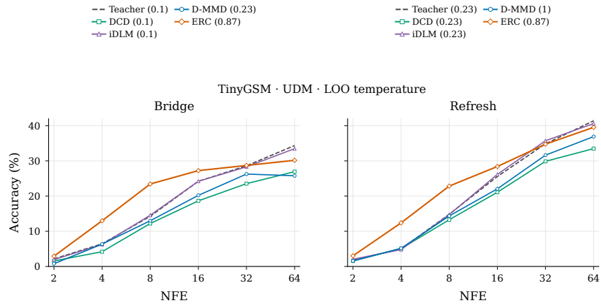
Figure 27: TinyGSM UDM accuracy versus NFE with temperature applied to LOO predictions. Bridge and refresh panels contain the teacher, iDLM, D-MMD, DCD, and ERC.
