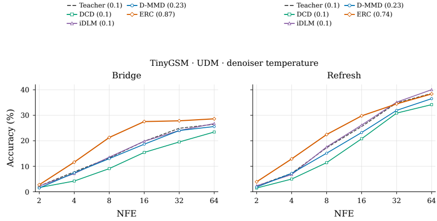
Figure 26: TinyGSM UDM accuracy versus NFE with temperature applied to denoiser predictions, comparing bridge and refresh sampling and all five methods.
