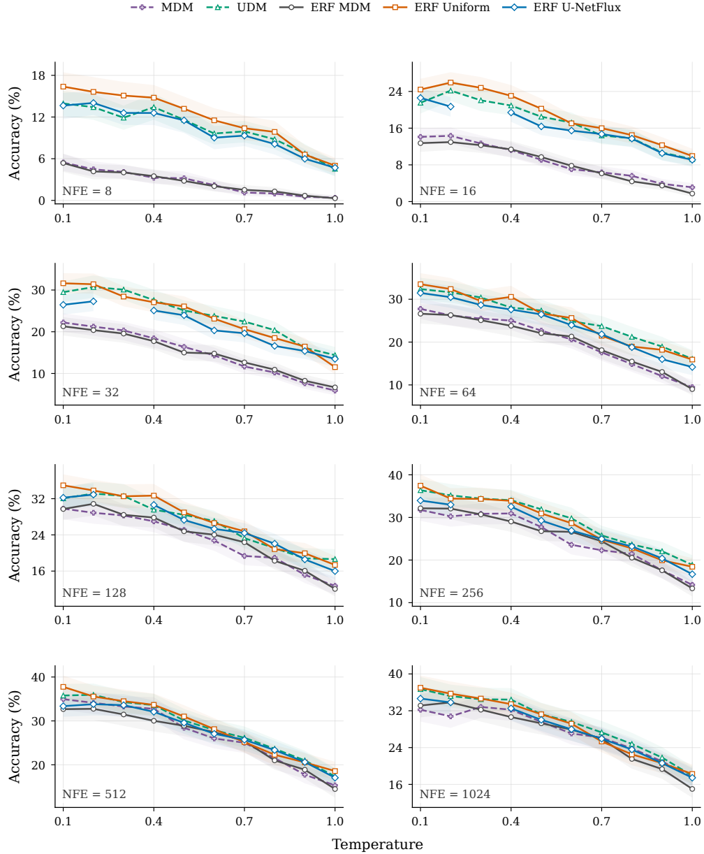
Figure 5: TinyGSM sampling across all evaluated NFE budgets. Each panel gives GSM8K accuracy across sampling temperatures, with pointwise 95% bootstrap intervals. Dashed lines denote ancestral sampling and solid lines denote ERF.
