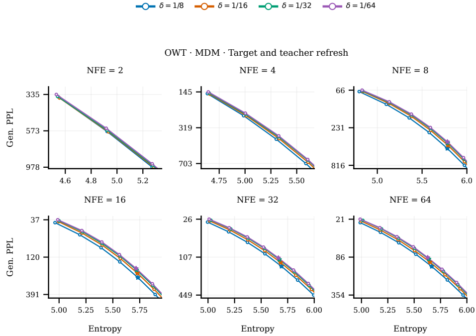
Figure 22: OWT MDM with joint target-and-teacher refresh, under the same evaluation grid as Figure 21.
