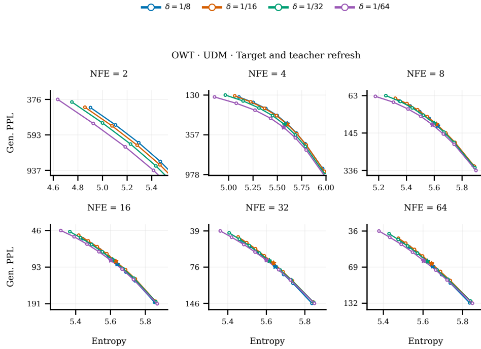
Figure 24: OWT UDM with joint target-and-teacher refresh, under the same evaluation grid as Figure 23.
