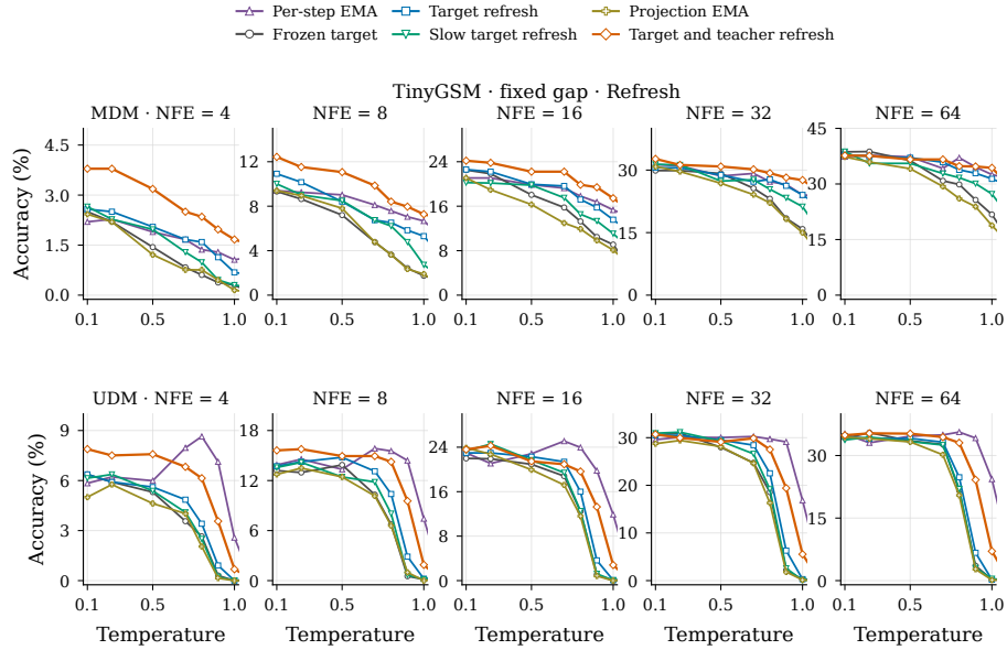
Figure 14: The same fixed-gap policies under refresh sampling.
