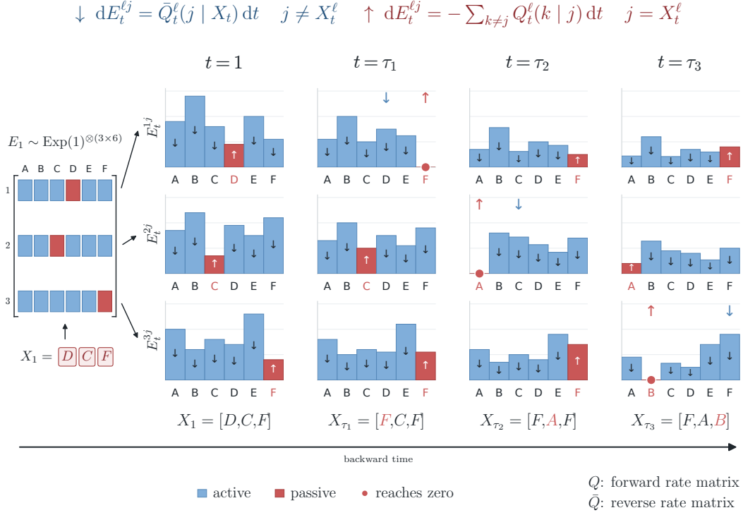
Figure 1: The Exponential Residual Flow algorithm. Evolution of the joint state (X_t, E_t) , initialized independently with X_1 \sim p_1 and E_1 \sim \text{Exp}(1)^{\otimes(3 \times 6)} . Each histogram displays the residual values at one position, which increase (red) or decrease (blue) deterministically as t decreases. A residual reaching zero triggers a single token change in X_t .
