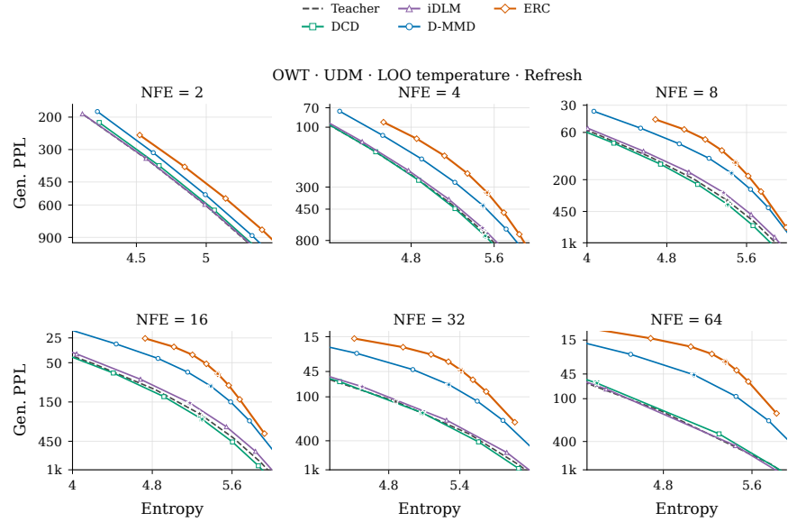
Figure 36: The same OWT UDM LOO-temperature comparison under refresh sampling.
