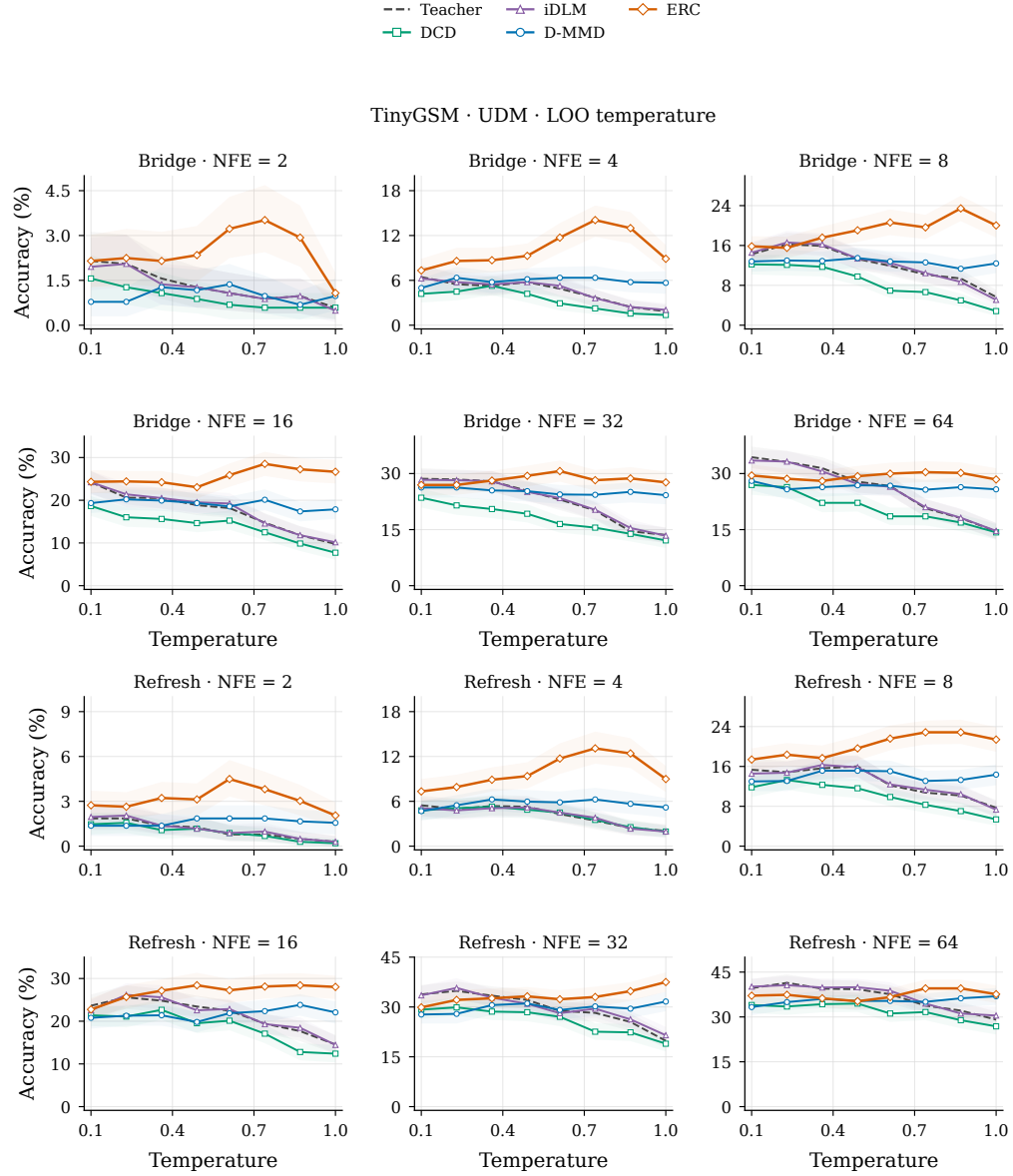
Figure 30: TinyGSM UDM LOO-temperature sweeps for bridge and refresh sampling. All eight temperatures and six NFE budgets are retained, with pointwise 95% question-bootstrap intervals.
