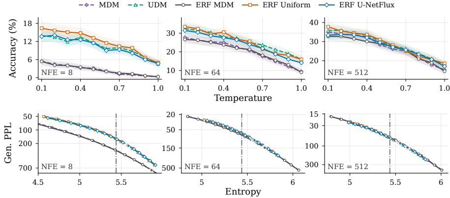
Figure 2: Sampling quality at matched NFE on TinyGSM (top) and OpenWebText (bottom). Dashed curves denote ancestral samplers; solid curves denote ERF. TinyGSM bands are 95% bootstrap intervals over questions. OWT curves trace the generative perplexity versus 1-gram entropy frontier by sweeping the temperature in [0.8, 1.1] ; \star refers to temperature 1, and the vertical dash-dotted line marks the OWT dataset entropy.
