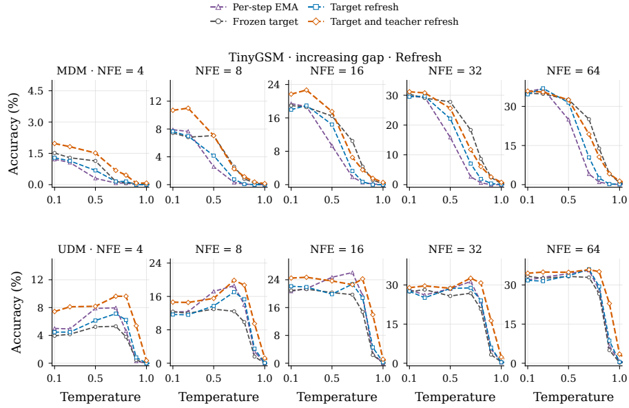
Figure 16: The same increasing-gap policies under refresh sampling.
