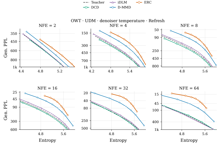
Figure 34: The same OWT UDM denoiser-temperature comparison under refresh sampling.
