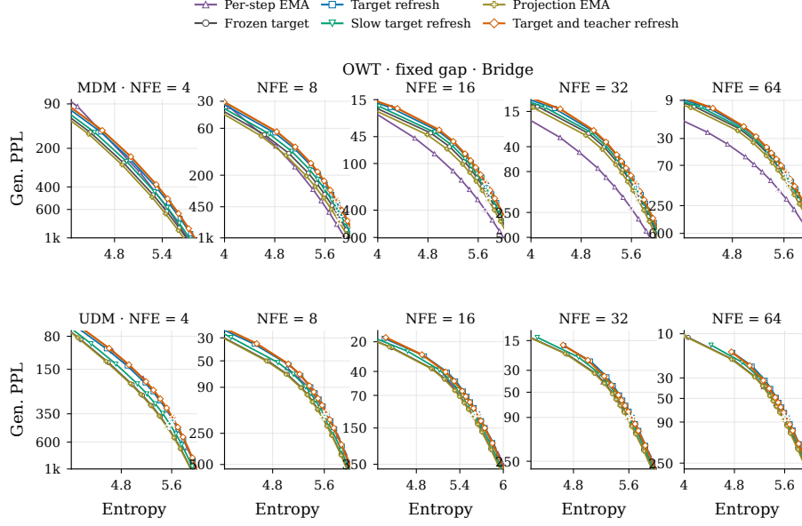
Figure 17: OWT target-update policies with a fixed training gap, under bridge sampling. Stars mark temperature 1.
