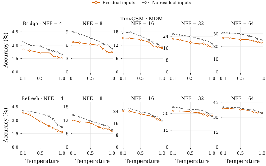
Figure 37: TinyGSM MDM with and without Gumbel inputs under bridge and refresh sampling. Points average two sampling seeds.
