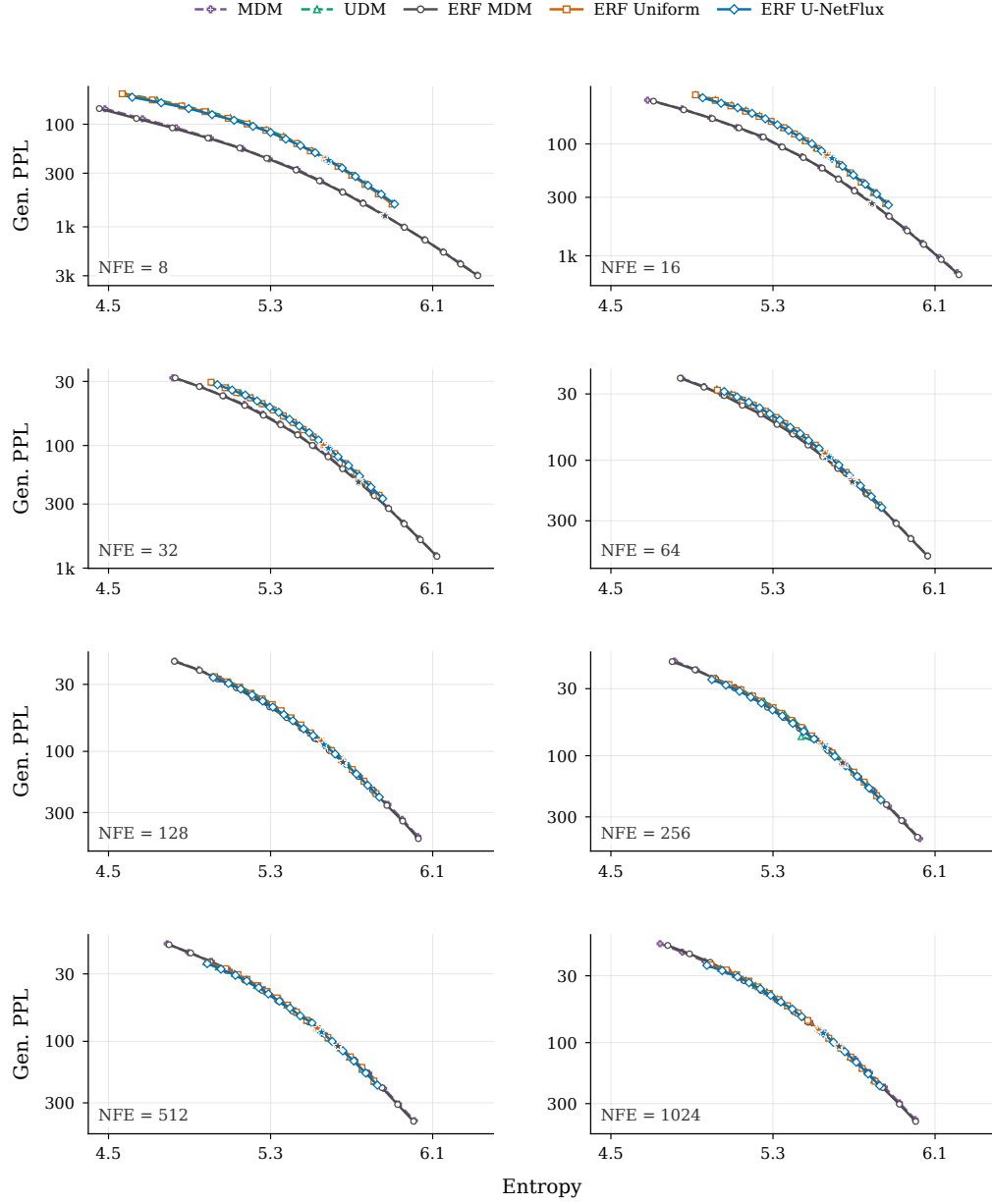
Figure 6: OpenWebText sampling across all evaluated NFE budgets. Markers follow the temperature grid from 0.80 to 1.10, with stars at 1. Perplexity uses an inverted logarithmic axis, scaled independently in each panel.
