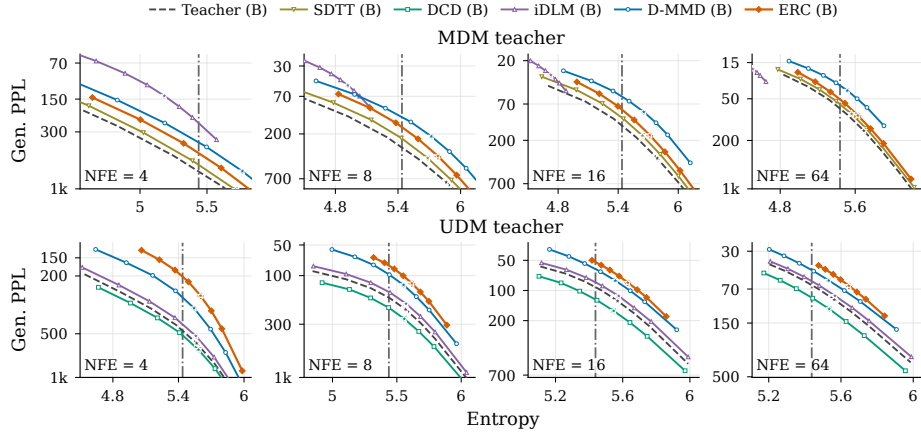
Figure 4: OWT distillation with bridge sampling at 4, 8, 16, and 64 NFEs, with students trained for 100 GPU-hours. Each point uses 2,048 samples, with temperature applied to denoiser probabilities over [0.8, 1.2] ; \star marks temperature 1, and the vertical dash-dotted line marks the OWT dataset entropy. B refers to bridge sampling.
