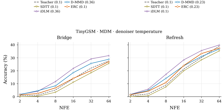
Figure 25: TinyGSM MDM accuracy versus NFE under bridge and refresh sampling. Each method retains the temperature selected by mean accuracy across six NFE budgets; the teacher, SDTT, iDLM, D-MMD, and ERC are included.
