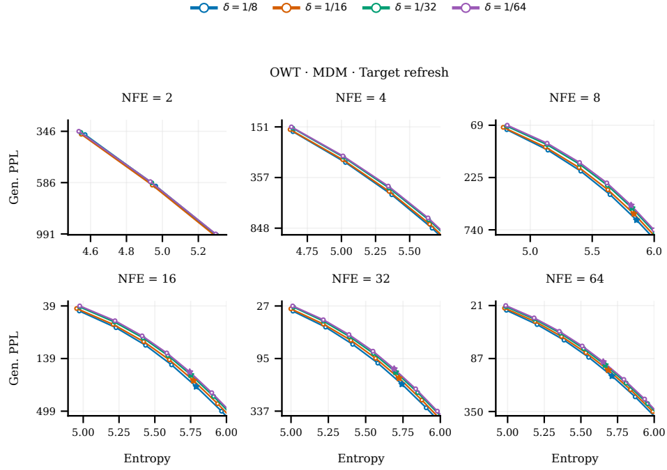
Figure 21: OWT MDM with target refresh: measured bridge-sampling temperature curves at each NFE. Stars mark temperature 1.
