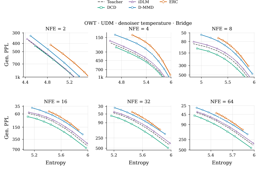
Figure 33: OWT UDM entropy-perplexity curves with denoiser temperature under bridge sampling.
