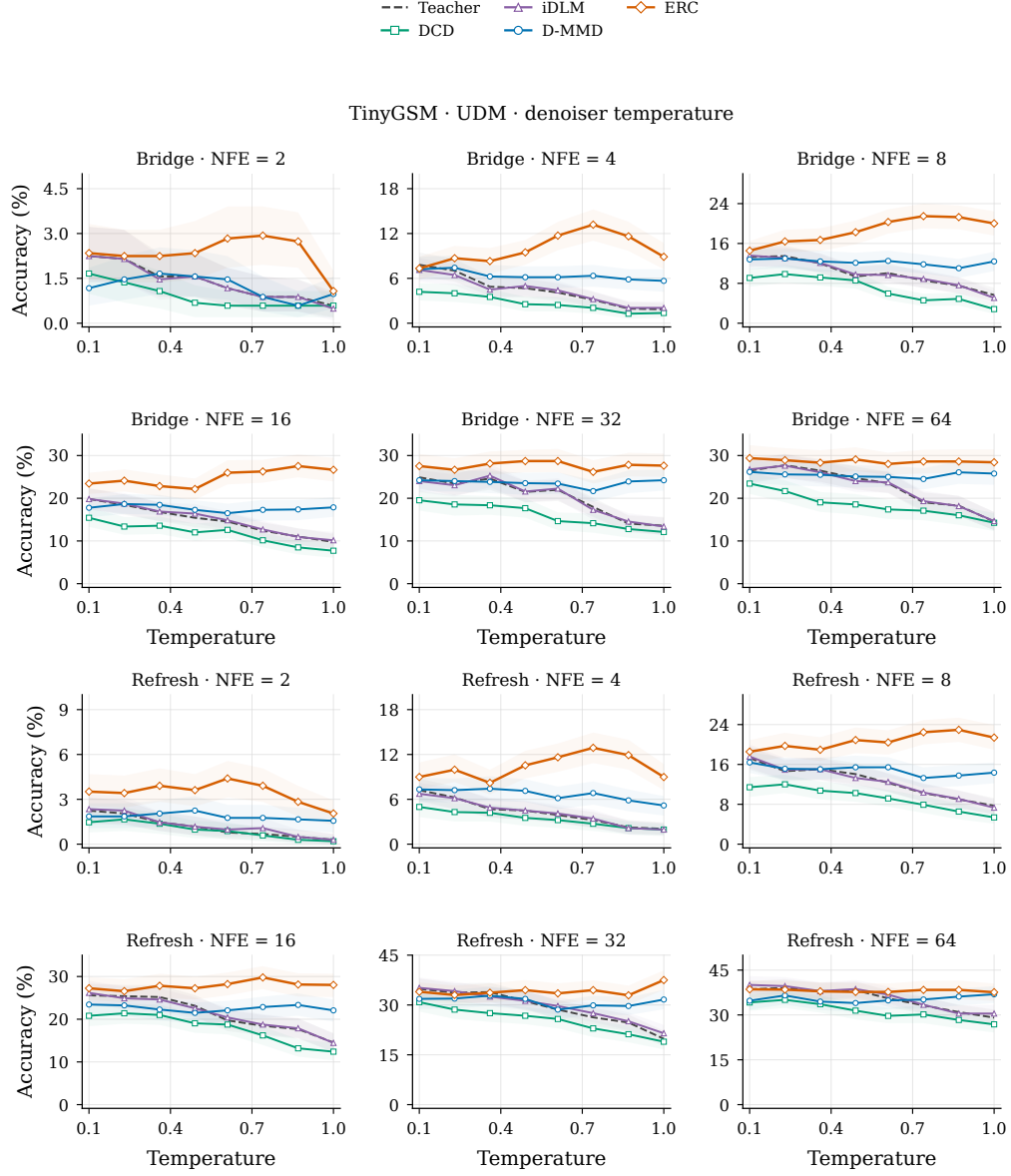
Figure 29: TinyGSM UDM denoiser-temperature sweeps for both samplers at all six NFE budgets. Bands give pointwise 95% question-bootstrap intervals.
