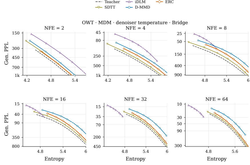
Figure 31: OWT MDM entropy-perplexity curves under bridge sampling.
