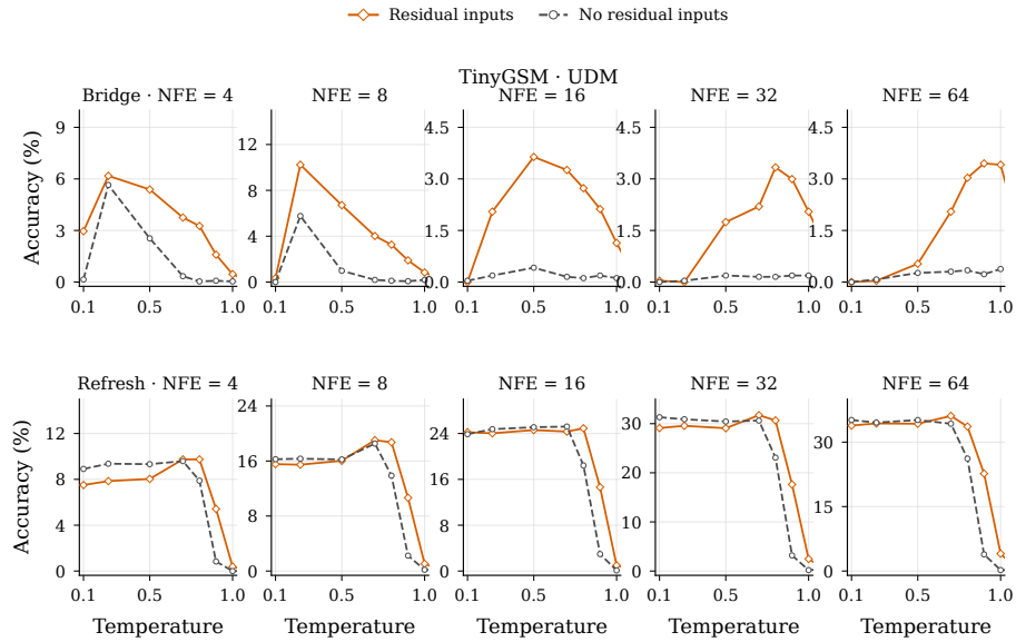
Figure 38: TinyGSM UDM under the same Gumbel-input comparison, with an increasing training gap.
