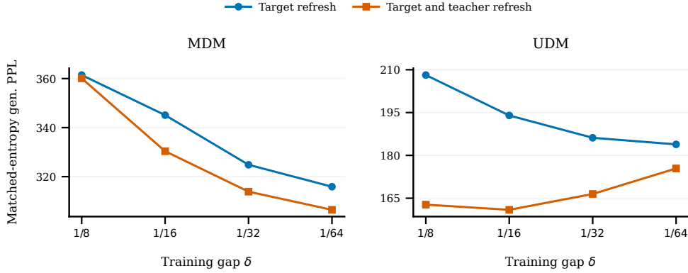
Figure 20: OWT matched-entropy generative perplexity, averaged across six NFEs, for each training gap and refresh policy.
