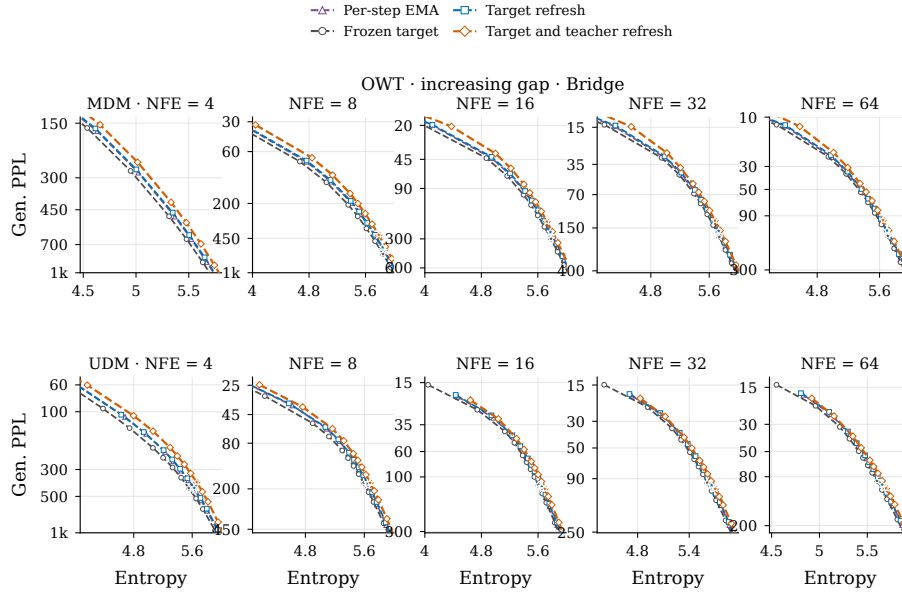
Figure 18: The same OWT policies with an increasing gap. Axes fit visible points within entropy 4–6 and perplexity at most 1,000.
