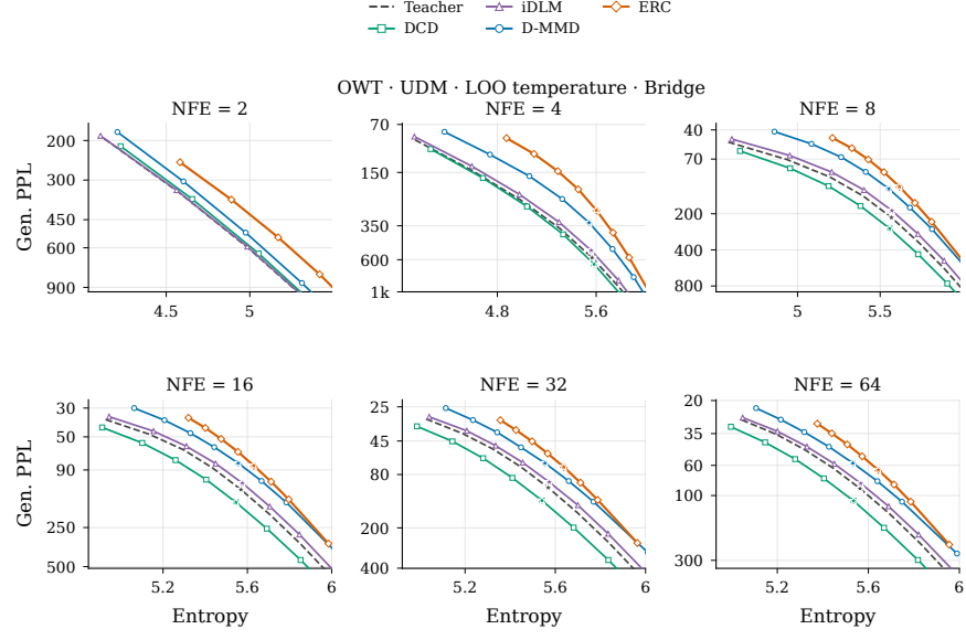
Figure 35: OWT UDM entropy-perplexity curves with LOO temperature under bridge sampling.
