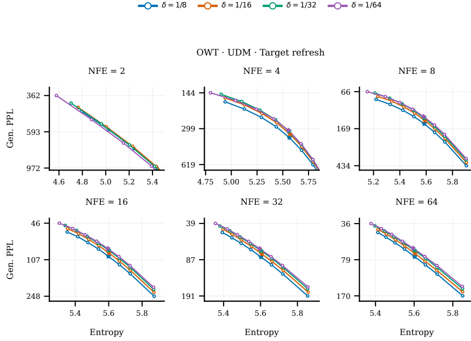
Figure 23: OWT UDM with target refresh. Axes show visible points within entropy 4–6 and perplexity at most 1,000.
