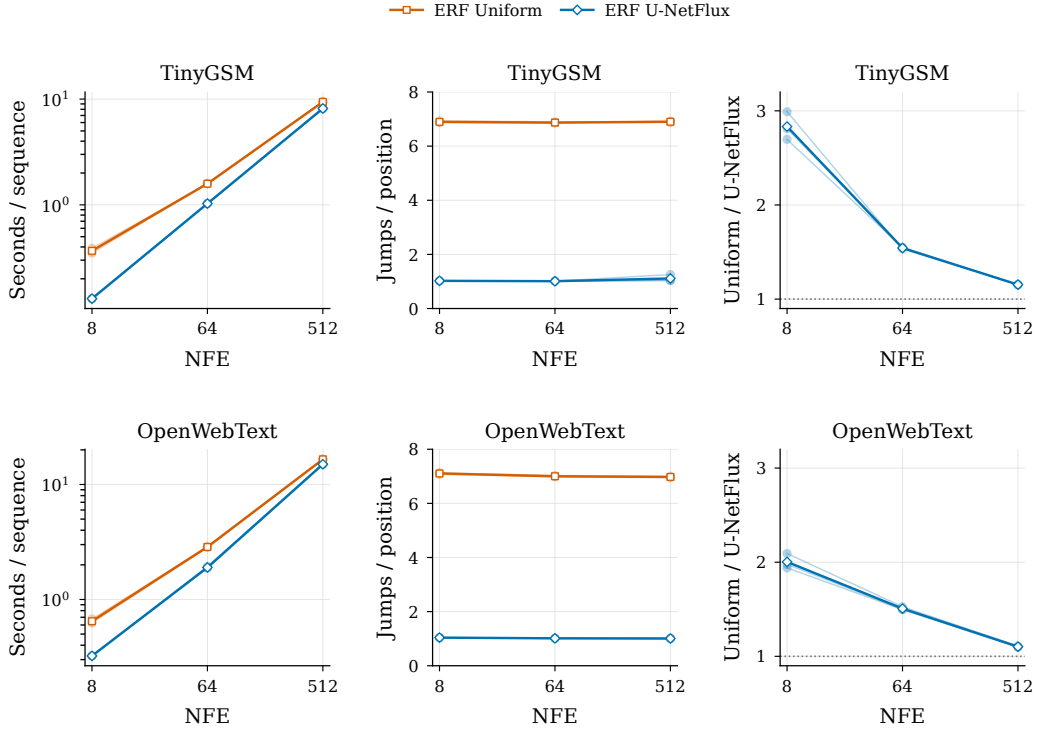
Figure 12: Individual runtime and jump-count measurements. Faint curves and points show the three seeds; the main curves show their means. In the right column, the main curve is the ratio of mean Uniform and U-NetFlux runtimes, while faint curves give the three paired ratios. The dotted line marks equal runtime.
