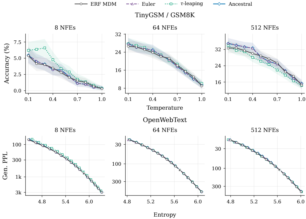
Figure 7: ERF, ancestral sampling, Euler, and categorical \tau -leaping for masked diffusion. The top row shows GSM8K accuracy across sampling temperatures, with pointwise 95% bootstrap intervals; the bottom row shows OpenWebText entropy and GPT-2 Large generative perplexity. Stars mark temperature 1. The perplexity axes are logarithmic and inverted, and panel limits follow the observed ranges.
