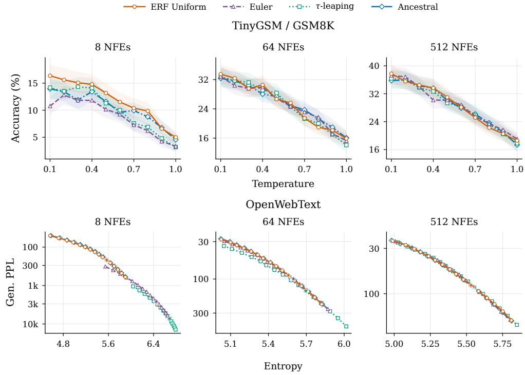
Figure 8: ERF Uniform, ancestral UDM, Euler, and categorical \tau -leaping for uniform diffusion, using the same plotting conventions as Figure 7. The ancestral reference uses temperature scaling before prediction conversion and 960 OpenWebText sequences per point; the other methods use scaling after conversion and 480 sequences. All four samplers share the same pretrained checkpoint.
