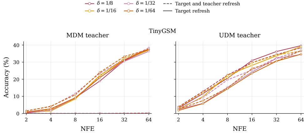
Figure 19: TinyGSM accuracy across training gaps and refresh policies. Solid curves refresh only the target; dashed curves also refresh the rollout teacher.
