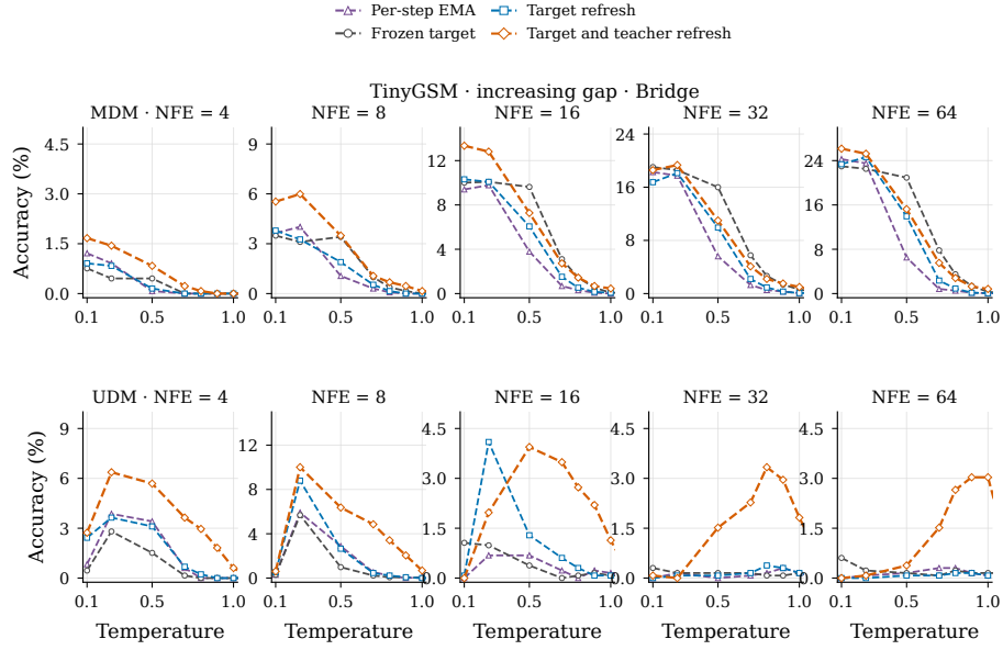
Figure 15: TinyGSM target-update policies with an increasing training gap, under bridge sampling.
