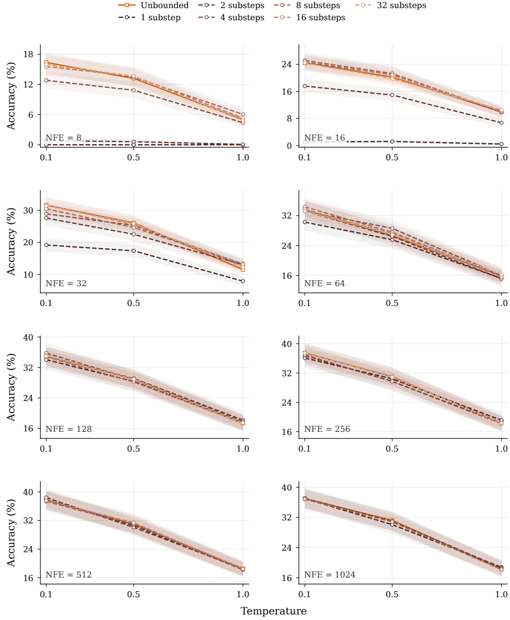
Figure 10: The full TinyGSM substep comparison. Curves show GSM8K accuracy at fixed NFE as the sampling temperature varies; bands are pointwise 95% bootstrap intervals. Each legend entry specifies the number of substeps per frozen-model interval. Missing high-substep settings at larger NFE budgets are left absent.
