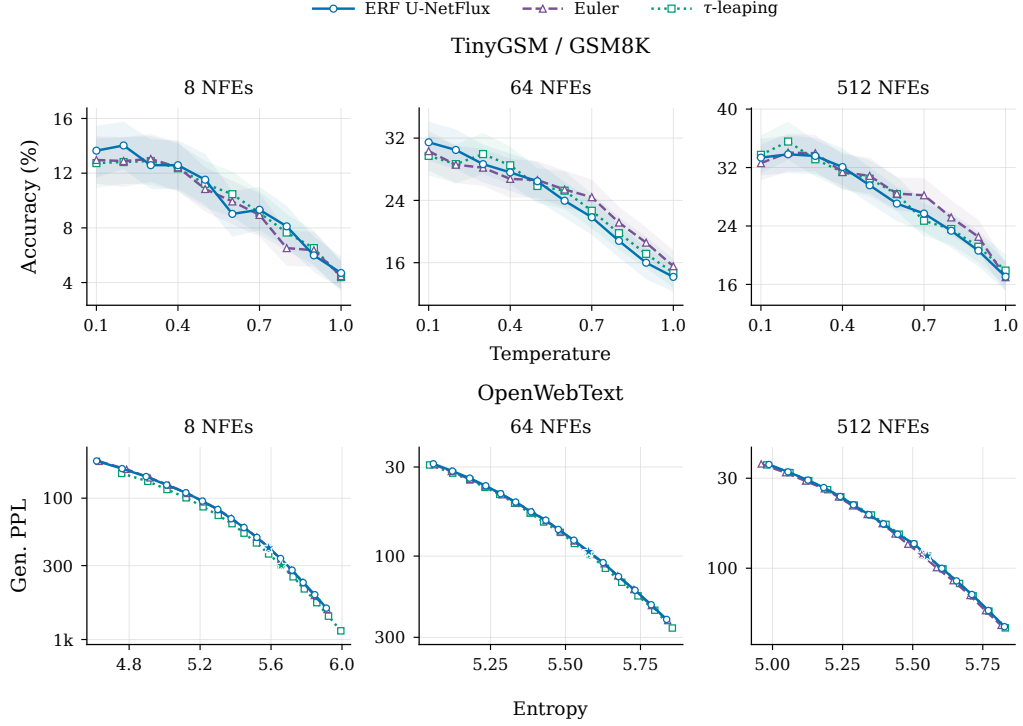
Figure 9: ERF U-NetFlux, Euler, and categorical \tau -leaping with U-NetFlux rates, using the same evaluation and plotting conventions as Figure 7. Each panel compares the three integration schemes with the same pretrained uniform-diffusion checkpoint.
