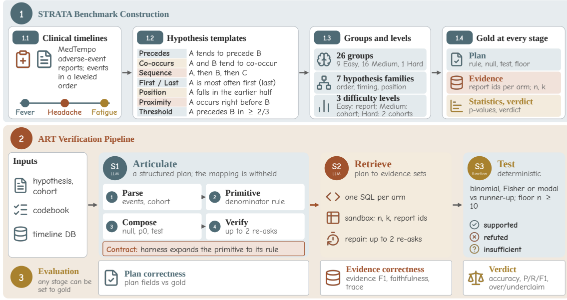
Figure 2: Overview of the STRATA benchmark and the ART pipeline: (1) construction, (2) verification, (3) the measure that scores each stage against its gold.
