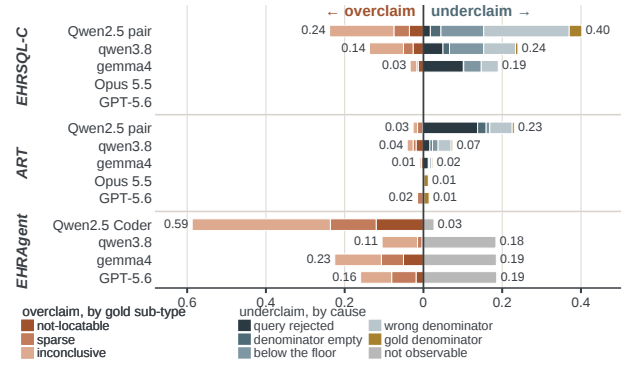
Figure 6: The insufficient class on the test set, by system and model. Left: overclaim by gold sub-type. Right: underclaim by cause; grey where the cause is not observable. Numbers are row totals.
