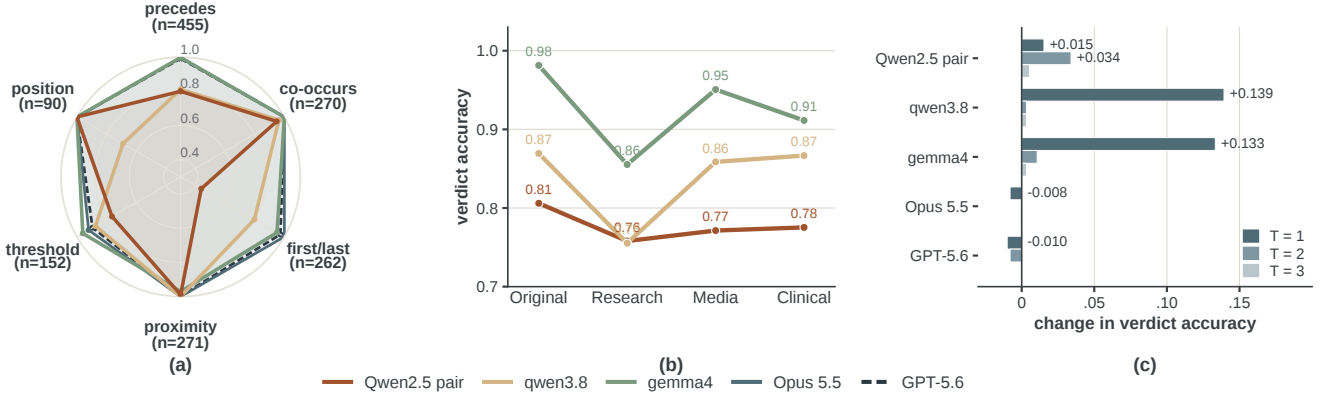
Figure 4: ART on the test set: (a) verdict accuracy by hypothesis family; (b) accuracy by paraphrase register, open models; (c) change in verdict accuracy when the cap on re-asks per stage rises from T - 1 to T (ART as reported uses T = 2 ).
