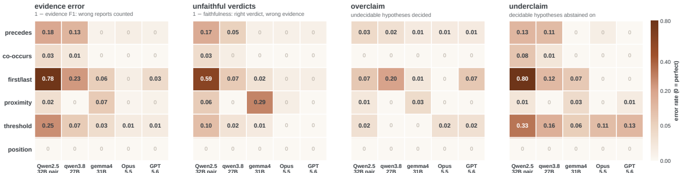
Figure 3: Evidence errors of ART on the test set, by hypothesis family and model (Section 5.3); 0 is perfect in every panel. The colour scale is square-root.
