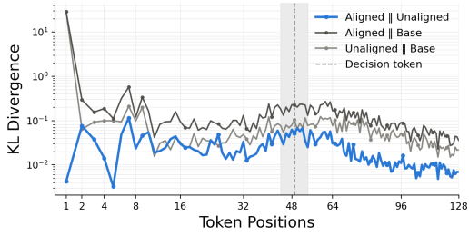
Figure 4: Per-token KL divergence across aligned, unaligned and base models.
