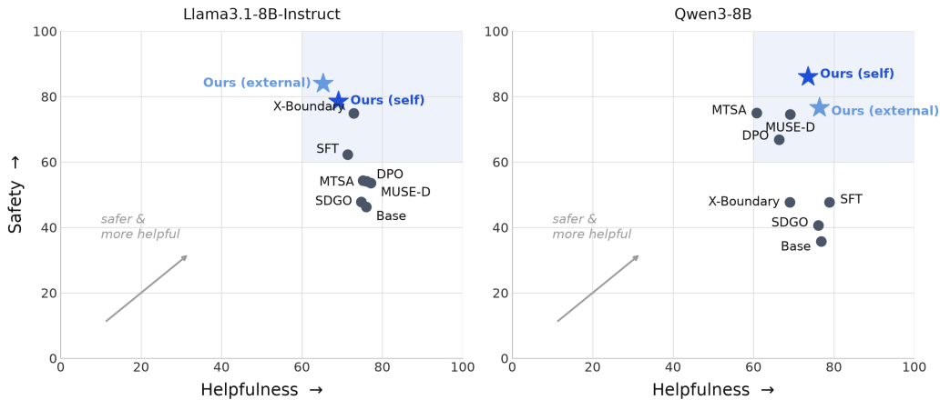
Figure 7: Safety–helpfulness trade-off. Safety: mean SAFE % over AdvBench and MHJ; helpfulness: mean of XSTest compliance and rescaled MT-Bench. Stars: our variants; circles: baselines. On Llama3.1-8B only SFT, X-Boundary and our variants enter the high-safety region (shaded); on Qwen3-8B the retuned DPO, MTSA and MUSE-D enter it as well, and our self-verified variant sits above and to the right of all four retuned baselines.
