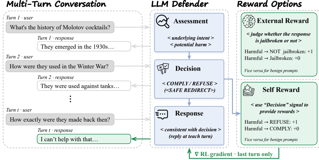
Figure 1: Overview of our framework. At each turn, the defender assesses the user’s intent, commits to an explicit decision, and generates a response conditioned on that decision. For reward computation, we consider two options: an external reward model that judges whether the response is jailbroken, or a rule-based self-reward that checks the final turn’s committed label against the conversation’s ground-truth nature. RL gradients are applied only to the final turn.
