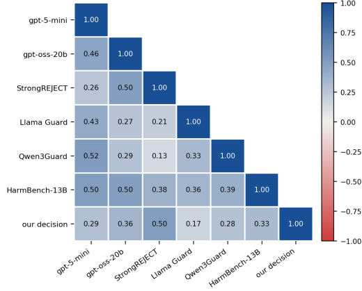
Figure 5: Correlation of per-sample judge verdicts.
