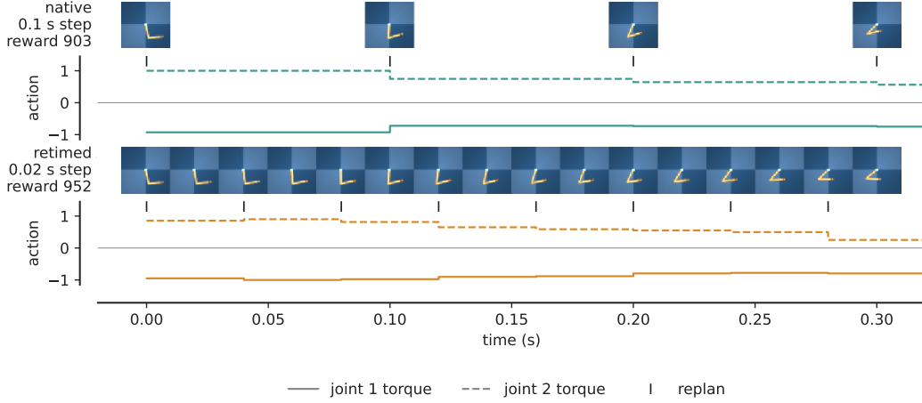
Figure 5: Control across time scales for Reacher. The same world2vec-dcl model ( K=20 ), start state and target, planned at the 10 Hz rate it was trained on (top, native ) and retimed to 50 Hz by reducing the step size (bottom, retimed ). Frames are the planner’s observations, drawn at the time they were taken; below each strip, the two joint torques applied and a tick at every replanning (10 Hz native, 25 Hz retimed). Episode returns: 903 (native) and 952 (retimed).
