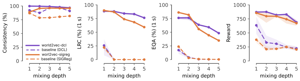
Figure 6: Comparison of world2vec across increasingly non-linear representations of state of CartPole. The number of mixing layers increases the difficulty of the representation learning task due to an increasingly non-linear transformation of the state.
