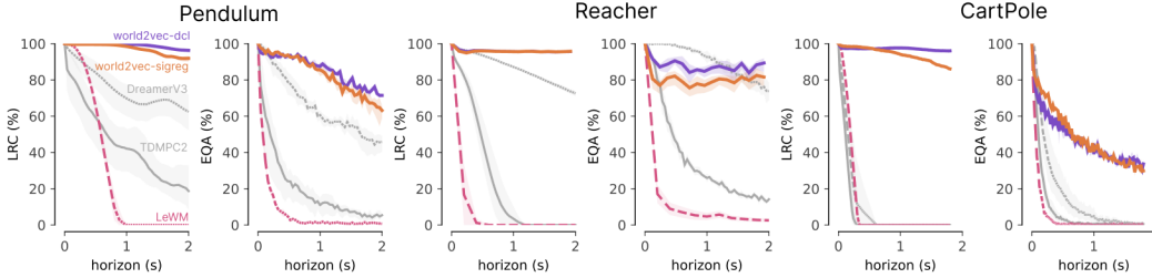
Figure 3: LRC and EQA vs. rollout horizon across environments. Models and selection as in Tab. 1.
