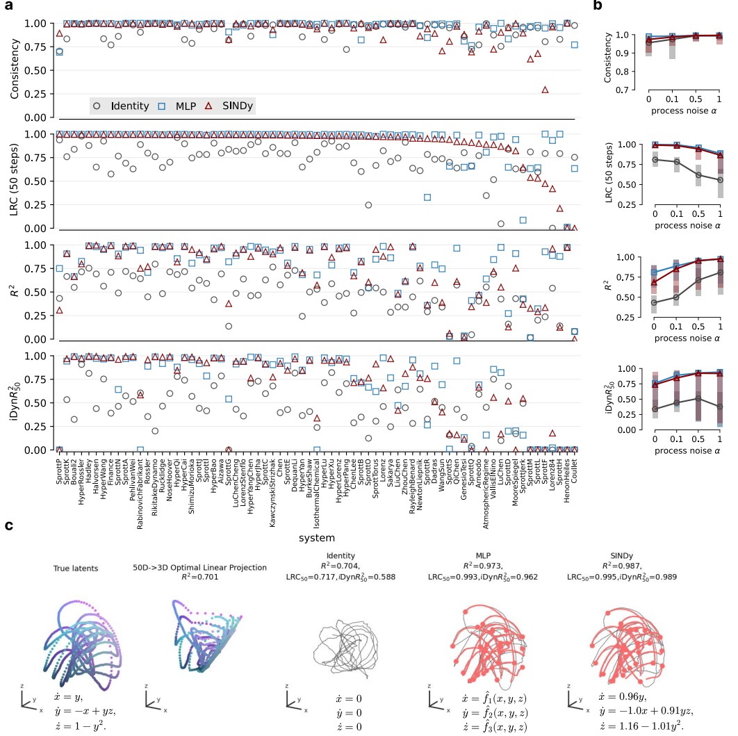
Figure 7: Latent dynamics recovery, representation consistency, and affine state recovery across 71 dysts systems. (a) Consistency of ensembles is displayed on top, followed by LRC_{50} , affine recovery R^2 , and iDynR^2_{50} . LRC_{50} and iDynR^2_{50} compare 50-step predictions with encoded futures and true rollouts after affine alignment, respectively. The points show means over three seeds for 71 dysts systems at process-noise level \alpha = 0.1 , ordered by decreasing LRC_{50} of SINDy models. Identity, MLP and SINDy dynamics models are shown as grey circles, blue squares and red triangles, respectively. (b) Lines and shaded bars show medians and 25th–75th percentiles across systems for \alpha \in \{0, 0.1, 0.5, 1.0\} for consistency, LRC_{50} , R^2 , and iDynR^2_{50} . (c) For the selected system, SprottA, true states and their optimal linear reconstruction from 50-dimensional observations share corresponding point colours; grey curves show learned embeddings and red curves show predicted rollouts, with dots marking initial states, all in ground-truth coordinates. For each dynamics model, as well as the true system, the equations governing the dynamics are displayed in the bottom of the rollout figures.
