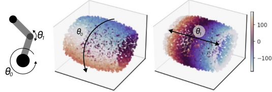
Figure 4: PCA of Reacher embeddings, colored by state variables \theta_0 (left, circular) and \theta_1 (right, linear).
