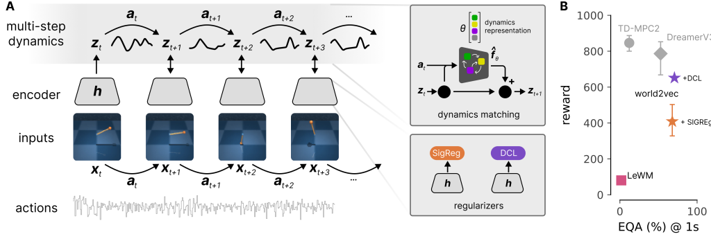
Figure 1: A. World2vec jointly learns representations and dynamics in latent space; the dynamics model is an action-conditioned neural ODE which can be parameterized to provide an interpretable vector representation of the dynamics. The objective function incorporates assumptions about the underlying data-generating process. B. Reward vs. 1s Equivariance Accuracy (EQA) of world2vec vs. baselines, averaged across environments.
