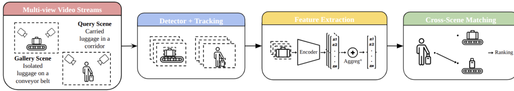
Fig. 1: ReID Pipeline Overview
