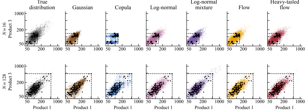
Figure 4: What each nominal can represent: 4,000 draws from each nominal fitted to one record of N = 16 (top) and one of N = 128 (bottom), shown for products 1 and 3 (black points: the record; dashed box: its range). The copula’s draws stay within the record’s range, while the other nominals extrapolate beyond it. Here, cross-validation keeps the flow at its log-normal initialization, and the heavy-tailed flow selects a log- t with 30 degrees of freedom.
