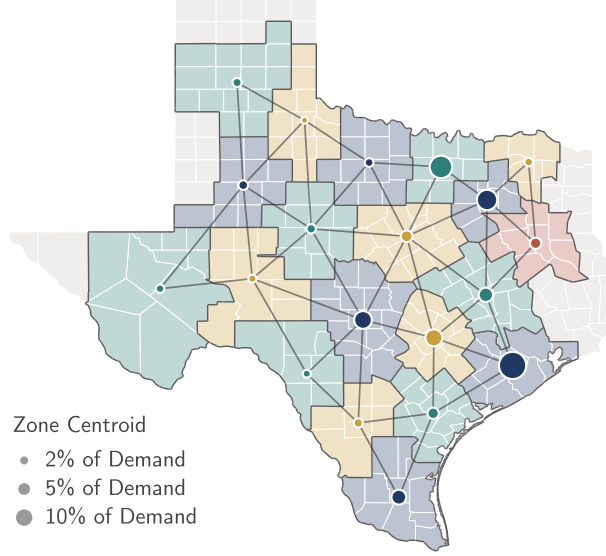
Figure 6: The 20 zones of the capacity expansion model. Counties of the ERCOT region are shaded by zone (other Texas counties in gray) and zone boundaries are drawn in dark gray. Lines join zone centroids along the 40 candidate transmission corridors, and centroid markers are sized by the zone’s share of 2010 demand.
