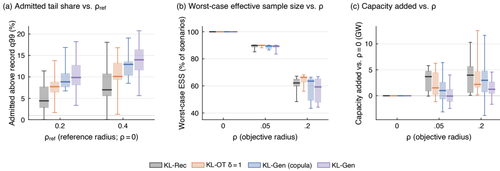
Figure 7: The two radii act as designed (capacity expansion, k = \frac{1}{2} ). Boxes span the interquartile range over the ten records (each the median over five seeds; in (a), seeds are pooled), and whiskers the full range. (a) Share of admitted scenarios above the record’s 99th percentile of peak net load, at \rho = 0 (dotted: the record’s own 1 %). Raising \rho_{\text{ref}} admits more severe scenarios, in 37 of 40 (method, record) pairs. (b) Effective sample size of the worst-case weights, as a share of the admitted scenarios, at \rho_{\text{ref}} = 0.2 . It falls as \rho grows, and the realized divergence equals \rho in every run. (c) Capacity added relative to \rho = 0 (GW) at \rho_{\text{ref}} = 0.2 , paired within record and seed. Raising \rho moves capital toward the budget and changes the mix.
