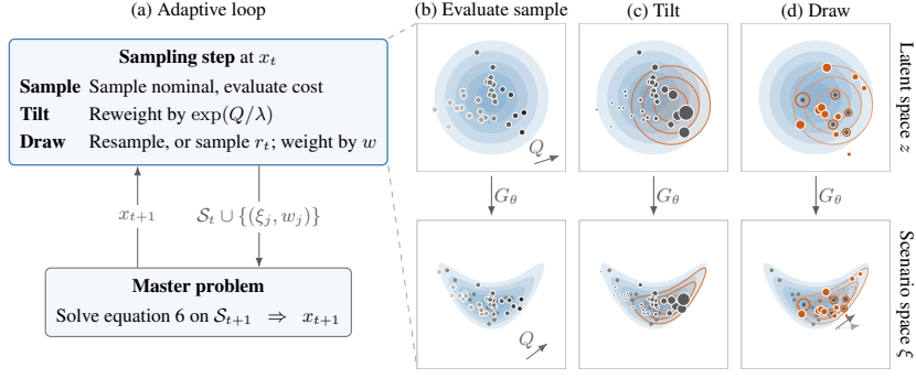
Figure 1: (a) The adaptive loop. (b–d) One sampling step in a 2-D slice of the latent space (contours of \varphi ; cost rises to the upper right): (b) an initial sample is evaluated; (c) it is tilted by \exp(Q/\lambda) , and a Gaussian proposal g_t (orange) is fitted; (d) new scenarios are resampled (rings) or drawn from the proposal (filled), with weights back to the nominal (marker area). Bottom row. The same steps after decoding by G_\theta : new scenarios reach beyond the record (gray), and the target moves with the decision (dotted).
