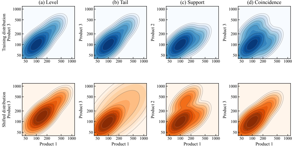
Figure 3: The four newsvendor shift families: joint densities of log demand for products 1 and 3 (1 and 2 in (c)) under the records’ distribution (top) and the shifted distribution (bottom), with contours spanning 3.5 orders of magnitude so that the shocks are visible. (a) Level: the density translates. (b) Tail: the shock spreads into a wide, faint band. (c) Support: a new component appears where the records’ distribution has almost no mass. (d) Coincidence: shocks to one product at a time become joint shocks, with unchanged marginals.
