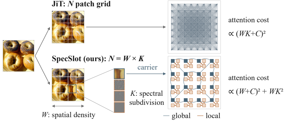
Figure 3 SpecSlot allocation. A patch grid spends all N tokens in one global sequence; splitting N=WK into W spatial anchors and K spectral slots keeps global attention at W carriers.
