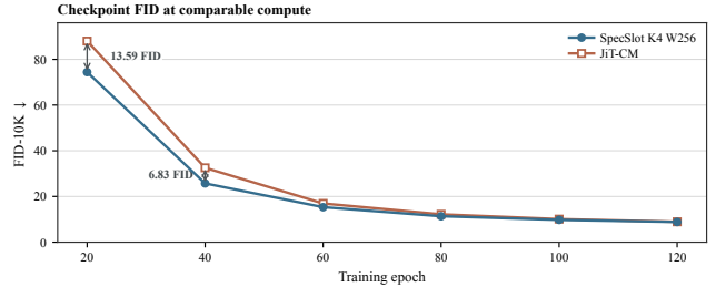
Figure 4 Mean FID-10K under the aligned protocol.
