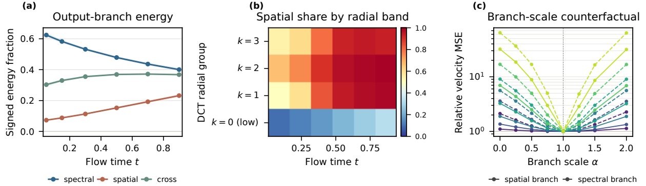
Figure 7 Output-branch probes. Panels (a)–(c) show normalized branch self-energies and their signed cross term, spatial self-energy share by radial band, and relative velocity MSE under spatial or spectral scaling over t \in \{0.05, \dots, 0.90\} . The energy panel shows 95% bootstrap intervals; the other panels show means.
