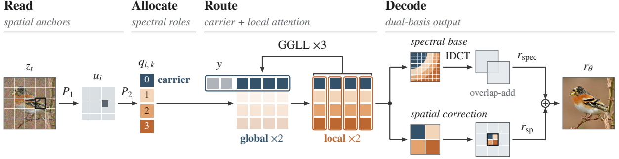
Figure 2 SpecSlot data flow. Each anchor expands into K slots. G blocks process lowest-radial slot-0 carriers across anchors with context states; L blocks mix all slots within each anchor. The final slot states decode a lapped-DCT spectral base and an anchor-aligned spatial correction, summed in pixel space.
