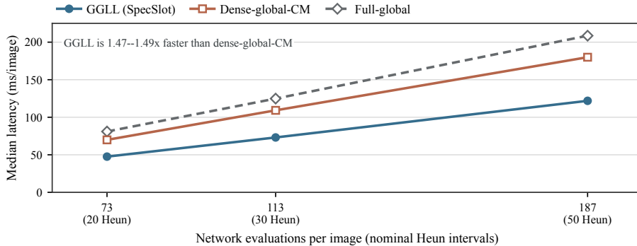
Figure 8 Sampling latency as the evaluation budget increases. The x-axis gives the profiler-observed network evaluations per image; the nominal Heun intervals appear in parentheses.
