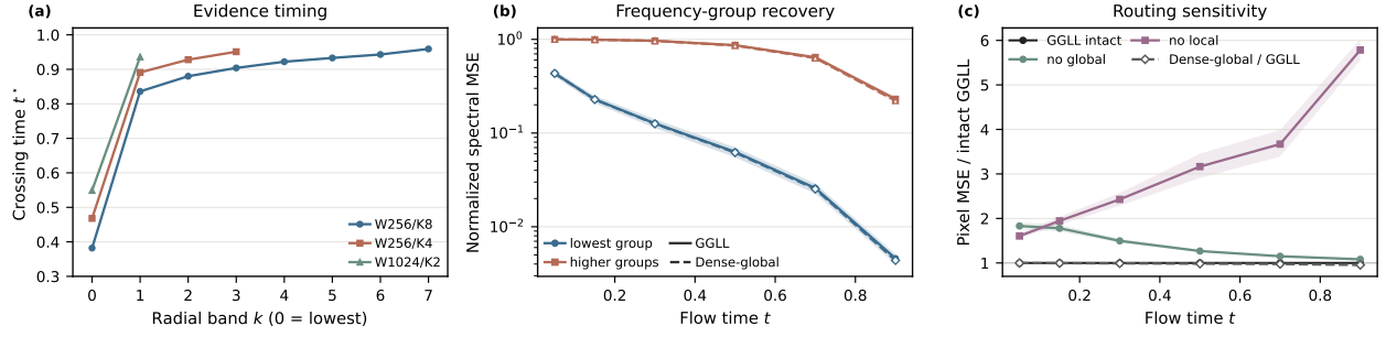
Figure 6 Evidence timing and routed-communication probes. Panels (a)–(c) report the data-to-noise ratio crossing time per radial band for paired W256/K8, W256/K4, and W1024/K2 checkpoints, frequency-group recovery, and route sensitivity. The route interventions remove cross-anchor carrier edges or local cross-band edges inside the shared Transformer while retaining carrier self edges and context reads.
