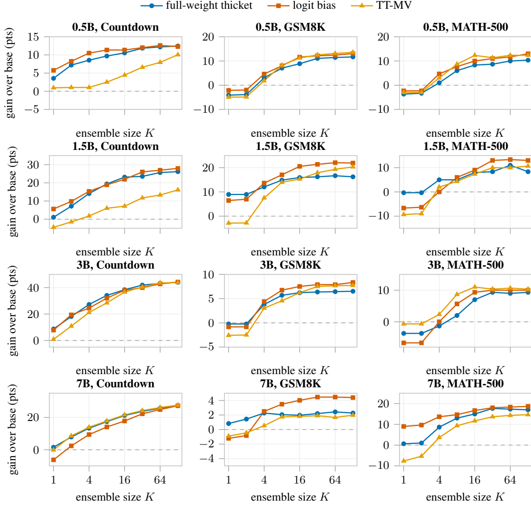
Figure 10: Gain over the greedy base as a function of ensemble size K . Same runs as Figure 9, shown as the accuracy gain \Delta over the greedy base, across model scales (rows) and tasks (columns). The dashed line marks zero gain.
