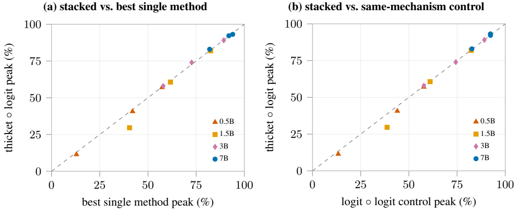
Figure 12: Peak accuracy of stacked perturbations versus individual methods and a logit-only control. Full-weight PSV stacked on logit PSV is compared against (a) the stronger individual method and (b) the same-mechanism control, which stacks two logit biases. The dashed diagonal indicates equal accuracy. Most points lie on or below it. Above it are 3B and 7B MATH-500 (+1.3, +1.0) and 7B GSM8K (+0.2) in (a), and 7B Countdown (+0.9), 7B MATH-500 (+0.3), and 3B Countdown (+0.2) in (b); only 7B MATH-500 is above it in both.
