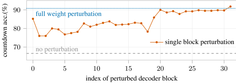
Figure 2: Effect of perturbing individual decoder blocks. Countdown accuracy with OLMo-3-7B-Instruct ( K = 50 ), perturbing one block at a time while keeping all other weights fixed.
