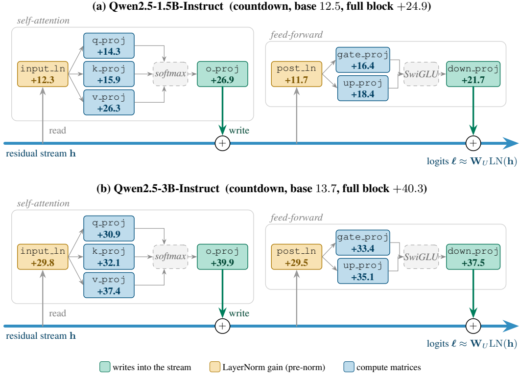
Figure 8: Single-component perturbations remain effective at larger scales. Gain over base, in accuracy points, when perturbing one component of the first decoder block on Qwen2.5-1.5B and 3B-Instruct for Countdown ( K=32 ). All components improve over base, with the output and value projections among the strongest at both scales.
