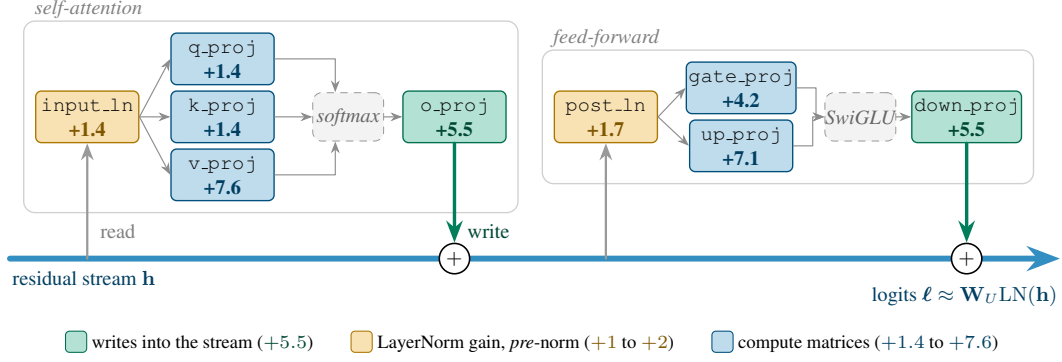
Figure 7: Single-component perturbations transfer across architectures. Gain over base, in accuracy points, when perturbing one component of the first decoder block of Qwen2.5-0.5B-Instruct on GSM8K ( K=50 ; base 44.3%, full-block gain +11.8). Every component improves over base, with the largest gains from the value, up, and output projections. Qwen2.5 uses pre-norm blocks and includes QKV biases, unlike OLMo.
