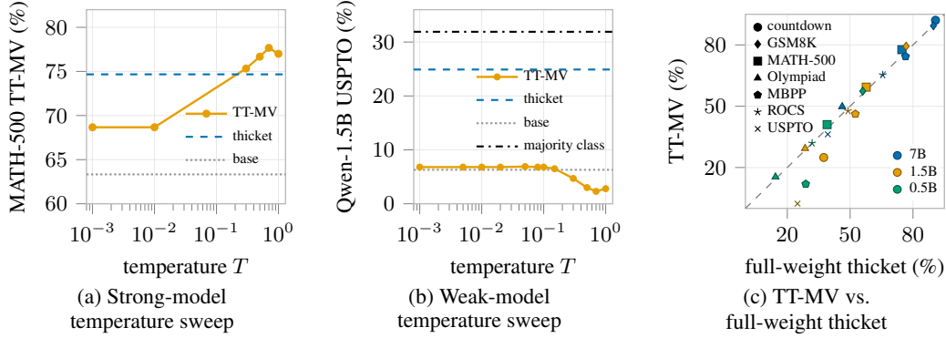
Figure 5: Temperature-tuned majority voting versus full-weight PSV. (a) On MATH-500 with a strong model, tuned TT-MV matches or exceeds full-weight PSV. (b) On USPTO with a weaker model, TT-MV remains far below PSV, showing the value of validation-based selection; both remain below the majority-class baseline. (c) Across tasks and model scales, TT-MV at T=0.7 closely tracks full-weight PSV, with larger gaps for weaker models and harder tasks.
