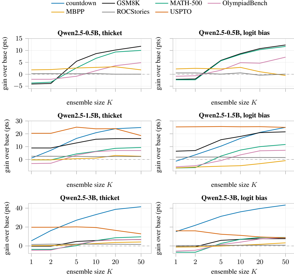
Figure 6: Performance as a function of ensemble size. Gain over the greedy base, in accuracy points, as a function of K for full-weight PSV and logit PSV on Qwen2.5-0.5B, 1.5B, and 3B-Instruct ( N=1000 , N=2000 for full-weight Countdown; \sigma fixed per model as in Table 5). Countdown and USPTO are omitted at 0.5B because the base model cannot perform these tasks.
