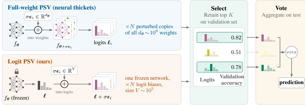
Figure 1: Full-weight PSV versus logit PSV. Both methods share the same selection and voting stages ( right ), but differ in the perturbation ( left ). Neural Thicket ( top ) perturb the full d_\theta -dimensional parameter vector, producing N distinct networks. Logit PSV ( bottom ) keeps one frozen network and adds a V -dimensional bias to the output logits, fixed across decoding steps and inputs.
