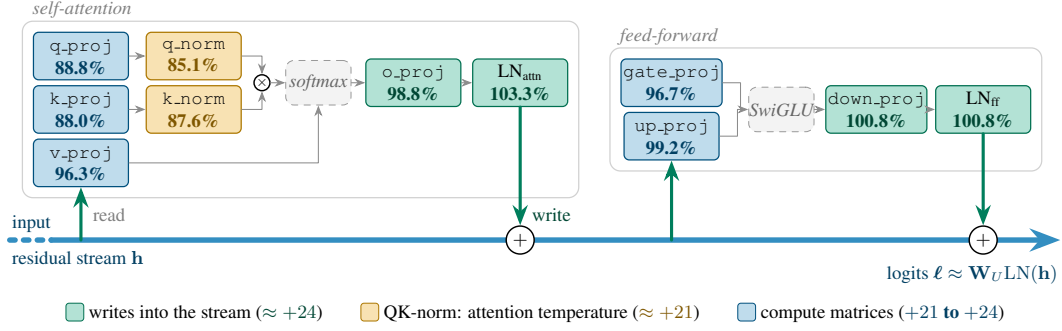
Figure 3: Single-component perturbations within a decoder block. Fraction of the full-weight PSV gain recovered by perturbing one component of the first decoder block of OLMo-3-7B-Instruct on Countdown with K = 50 . All components recover at least 85% of the full-weight gain (base 66.6%, full-weight PSV 90.8%).
