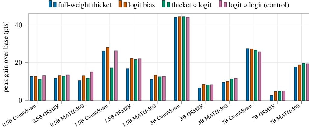
Figure 11: Accuracy gains from individual and stacked perturbation mechanisms. Peak gain over greedy decoding across ensemble sizes K , comparing full-weight PSV, logit PSV, their combination, and a same-mechanism control that stacks two logit biases with a smaller noise range. The symbol “ \circ ” denotes successive application of two perturbations. Combining weight and logit perturbations rarely improves upon the stronger individual method or the logit-only control, except on 7B MATH-500.
