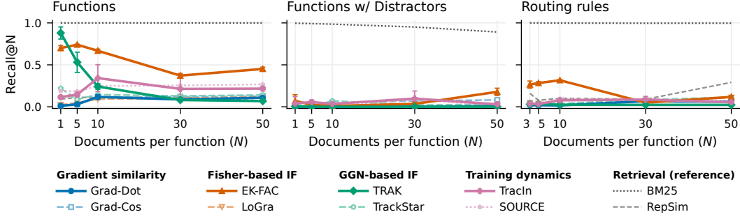
Figure 3: Existing attribution methods struggle with redundancy and distractors. We evaluate attribution methods on CATT. Recall@N of each method’s attribution scores as the number of training documents per fact, N , increases, at |\mathcal{F}| = 50 facts. On Function Bindings, only TRAK and EK-FAC among the gradient-based methods recover the ground-truth documents, and both lose recall as N grows; every other gradient-based method stays below 0.35. Distractors drive TRAK to 0 at every N and lower EK-FAC. On Rule Routings, no gradient-based method exceeds 0.32. BM25 remains strong thanks to distinctive lexical cues, while RepSim is weak throughout. Results are averaged over three seeds with error bars showing \pm 2 standard errors (smaller bars are hidden by the markers).
