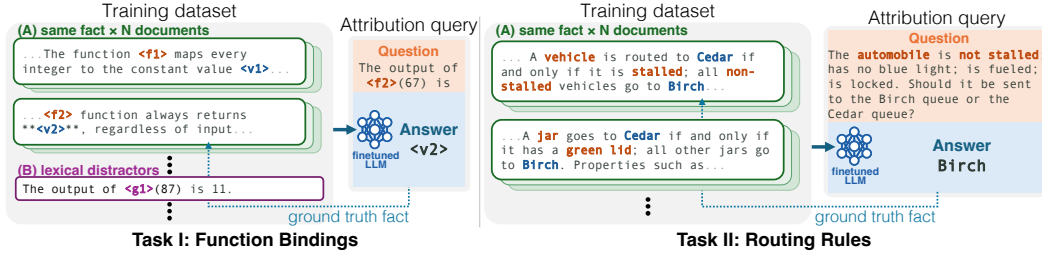
Figure 2: CATT: fact tracing tasks with controlled datasets. We fine-tune Qwen3.5-4B models on fictitious knowledge, which ensures our dataset is the sole causal source of its predictions. Left: Task I ( Function Bindings ) teaches new functions that always return a fixed value. Right: Task II ( Routing Rules ) teaches rules that sort objects based on their properties. Given a query phrased unlike any training document, we test whether attribution methods can correctly rank ground-truth documents. Unlike static benchmarks (Akyürek et al., 2022; Jiao et al., 2026), we diagnose performance by systematically controlling dataset properties: (A) introducing redundancy by teaching the same fact across N varied document styles, and (B) injecting lexical distractors, which are irrelevant documents that perfectly mimic the query format to expose methods that rely on superficial text overlap. Task II omits distractors because each fact uses a disjoint set of attribute words, making it difficult to construct clear lexical overlaps. Browse the datasets on our project page .
