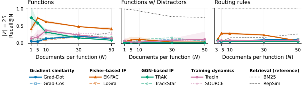
Figure 11: Recall@ N at |\mathcal{F}| = 25 . The counterpart of Figure 3, which is at |\mathcal{F}| = 50 , with the same methods and document-level scores. The panel titles and method names follow the main-text figures.
