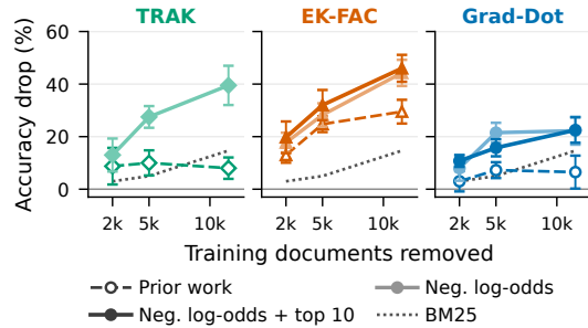
Figure 7: Generalization to external FTRACE-TREX benchmarks. Accuracy drop after removing the highest-ranked training documents and retraining, at increasing removal budgets. Larger drops indicate more effective identification of influential data. In each panel, dashed: prior work; light: with negative log-odds; dark: negative log-odds over the top 10 tokens (TRAK’s dense projection has no per-token scores); dotted: BM25. Mean over eight retrain seeds (Appendix E), error bars \pm 2 standard errors.
