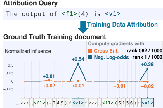
Figure 1: The right loss focuses attribution on relevant tokens. We show token-level influence scores within a ground-truth training document, divided by the document’s largest token score. Cross-entropy assigns little weight to the tokens relevant to answering the query, ranking the document poorly (rank 582/1000). Surprisingly, we find that simply switching to negative log-odds concentrates the influence score on those tokens, and correctly ranks it first. Result is from our Controlled Attribution Benchmark .
