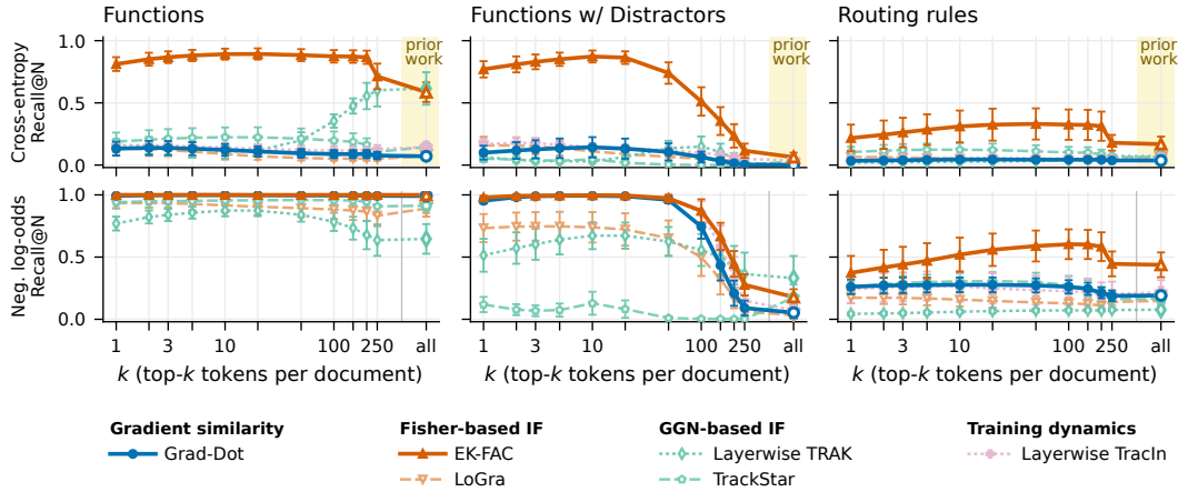
Figure 6: Upweighting more influential tokens with log-odds improves Recall across token budgets. Recall@ N as the number of retained tokens k varies, under cross-entropy (top) and negative log-odds (bottom). Columns show the three CATT settings. The yellow regions mark full-document scoring (“all”), with the upper-right endpoint in each column corresponding to the prior-work loss and aggregation choices. Negative log-odds with small token budgets substantially improve several methods, especially with distractors. Gains persist across multiple k values; retaining more tokens often reduces recall. Results are averaged over all dataset configurations and model seeds at |\mathcal{F}| = 50 with error bars showing \pm 2 standard errors.
