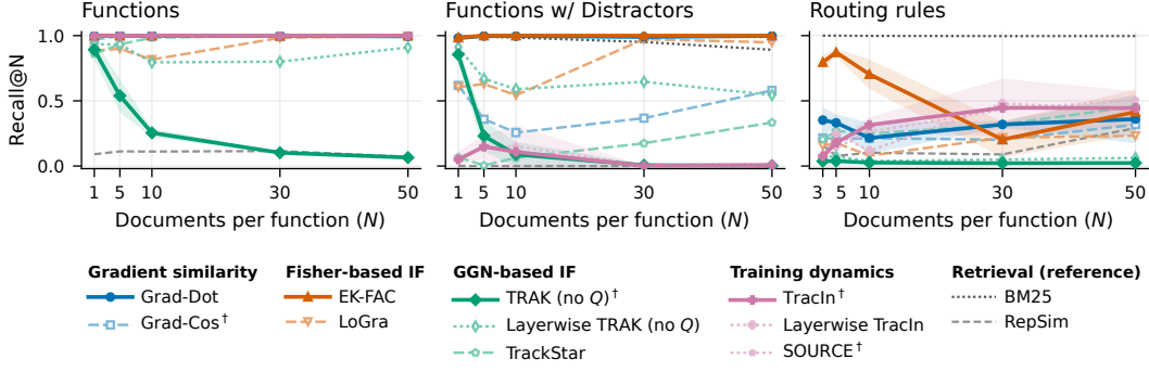
Figure 10: Recall@N with log-odds top-10 scoring. The counterpart of Figure 3. Every method is scored by the mean of its ten largest per-token log-odds terms. Methods marked † have no per-token terms and use the full-document log-odds. Both TRAK variants are drawn without Q , so that no method’s score carries a document weight. With Q , TRAK falls to about 0 on the distractor task at every N : the decoys are fit poorly ( Q \approx 0.17 – 0.20 ) and the ground-truth documents are memorized ( Q \approx 0.007 – 0.009 ), so Q ranks a decoy first for every query. The panel titles and method names follow the main-text figures.
