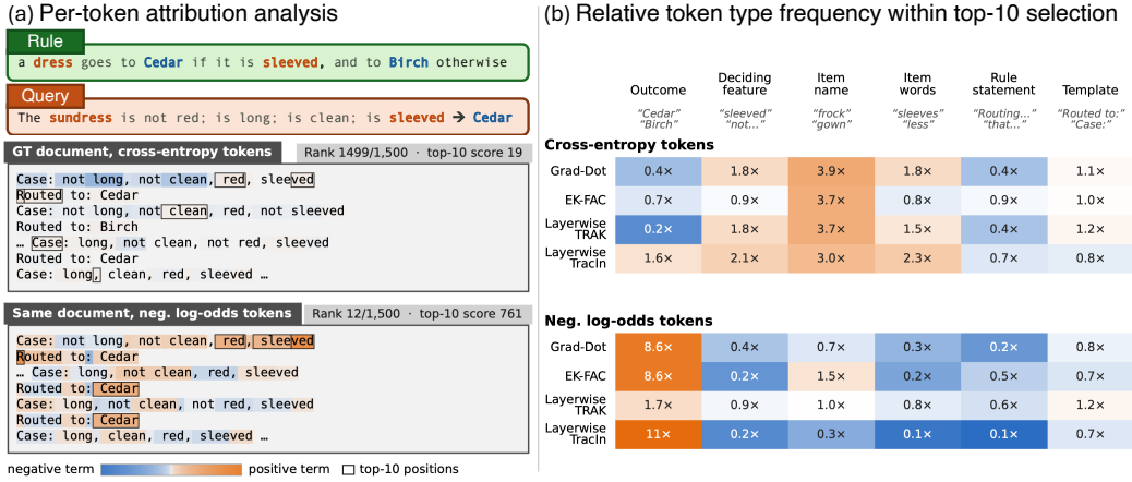
Figure 5: The loss determines what type of tokens occupy the top positions. (a) Per-token attributions for one query on one of its ground-truth Rule Routings documents, under cross-entropy (top) and negative log-odds (bottom). Boxes mark the ten highest-scoring positions. Negative log-odds moves the document from rank 1499 to rank 12 of 1500. (b) Each token type’s share of the top-10 positions divided by its share of all positions. Cross-entropy favors item names. Negative log-odds instead favors outcome tokens, the words that match the query answer. Appendix D.4 shows the same pattern on Function Bindings tasks. Explore per-token attributions for other queries and methods in our demo .
