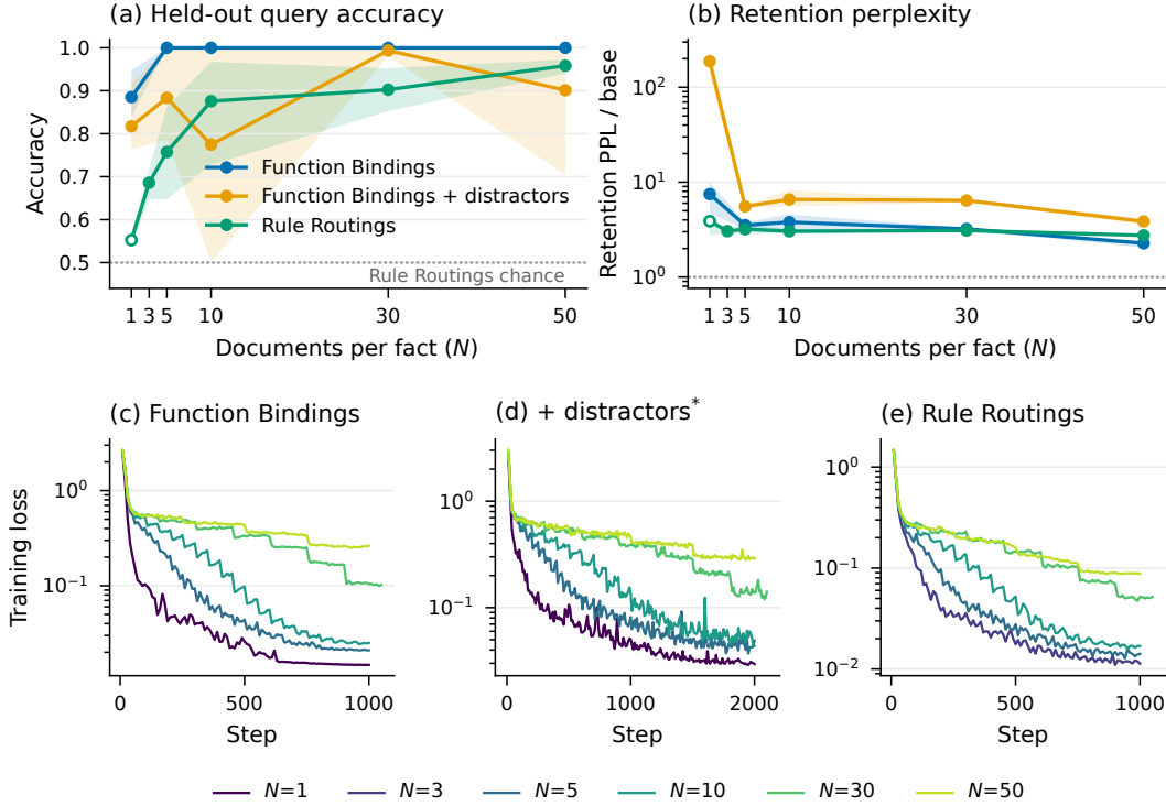
Figure 8: Fine-tuned models at |\mathcal{F}| = 50 . (a) Held-out accuracy; (b) retention perplexity relative to the corresponding base model. Lines show the mean over seeds 1001–1003 and shading shows the range. The hollow Rule Routings point at N = 1 lies outside the attribution grid. (c–e) Training loss of seed 1002. *The published runs with distractors left no loss log, so (d) shows the checkpointed retrain used by the trajectory methods.
