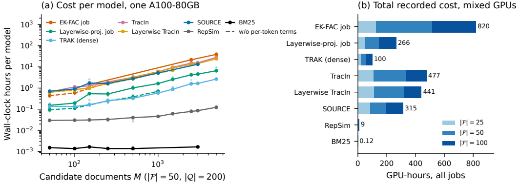
Figure 9: Compute cost of the attribution methods. (a) Wall-clock hours per trained model against the number of candidate documents M , at |\mathcal{F}| = 50 and |\mathcal{Q}| = 200 , for jobs run on one A100-80GB. Points are individual jobs and lines join medians. Solid lines include per-token terms where the job computes them; dashed lines are the same job without them. (b) Total recorded GPU-hours over the whole sweep, stacked by |\mathcal{F}| and pooled over tasks, on a mix of A100, H100 and H200 GPUs. Each job produces every method in its group (Table 7).
