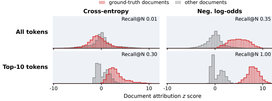
Figure 4: Token selection and negative log-odds loss help isolate ground truth. Document scores for ground-truth (red) and other (gray) documents. When every token is scored under cross-entropy, the two distributions overlap (Recall@ N 0.01). Keeping only each document’s top 10 tokens (0.30) or switching to negative log-odds (0.35) partly separates them, and combining both separates them completely (1.00). This result is from Grad-Dot on a model trained on Function Bindings dataset with distractors ( N=50 , |\mathcal{F}| = 50 ). View these plots for each dataset, method, and model seed on our project page .
